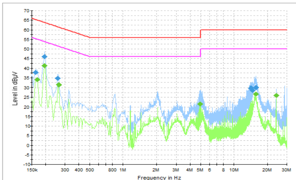
Fig.8 Conducted Emission
