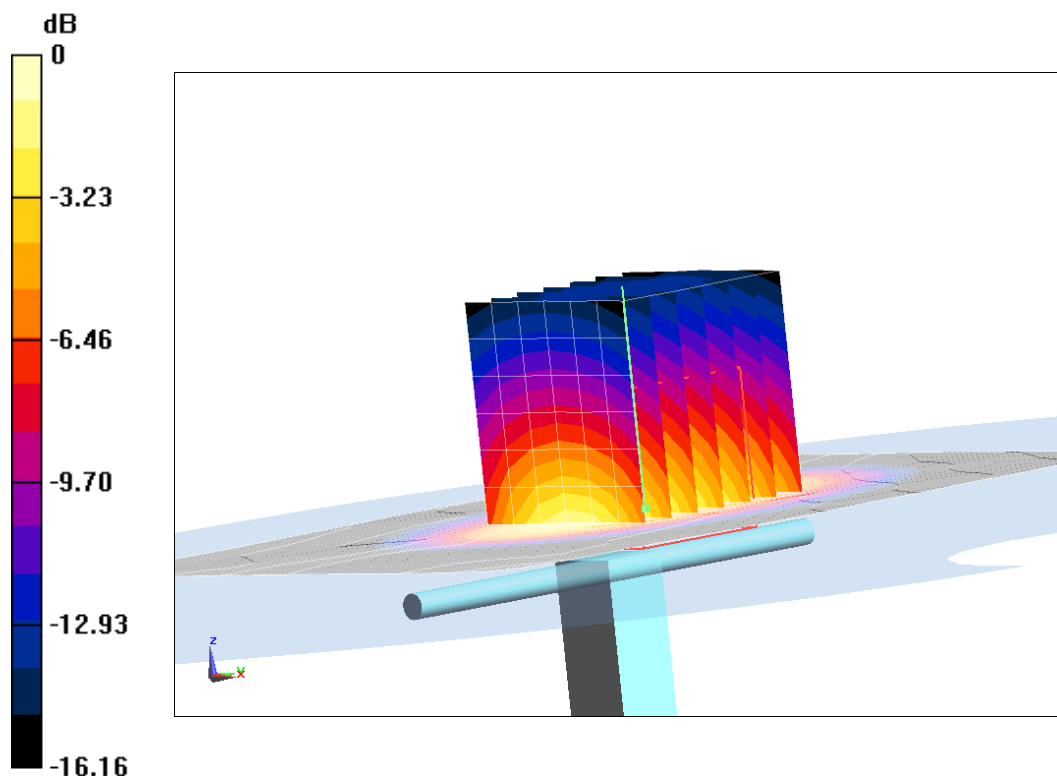
Fig.B.15 validation 1750 MHz 250mW
