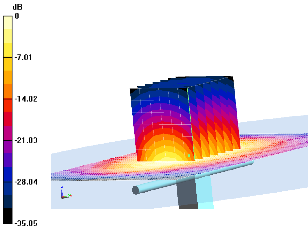
Fig.B.16 validation 1750 MHz 250mW
