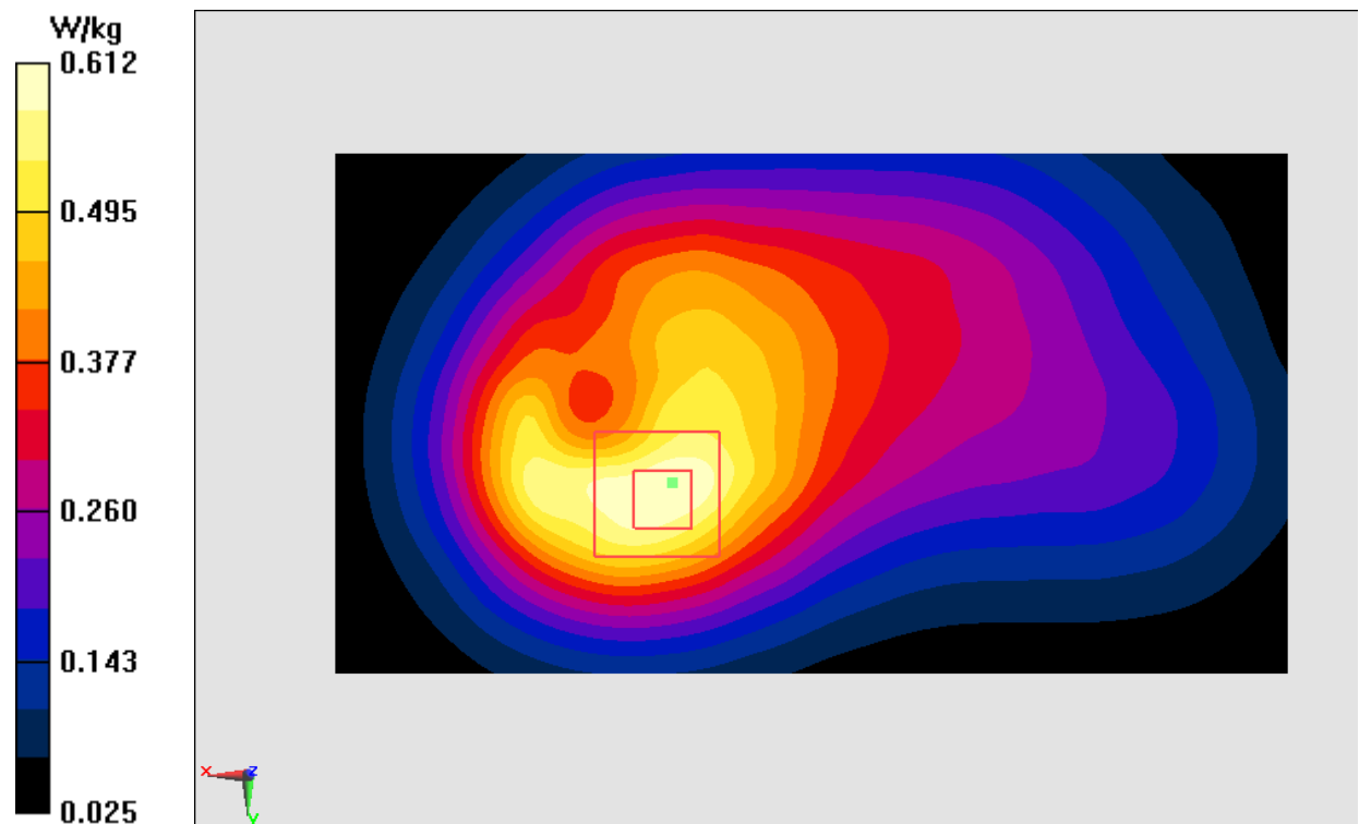
Fig.8 LTE Band4
