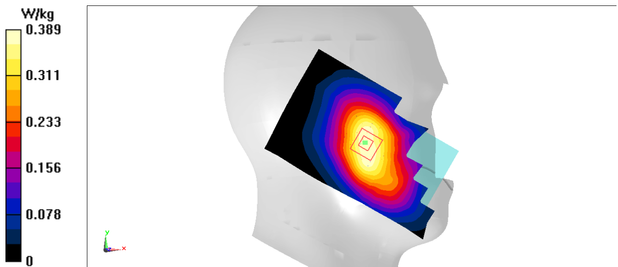
Fig.1 CDMA BC0
