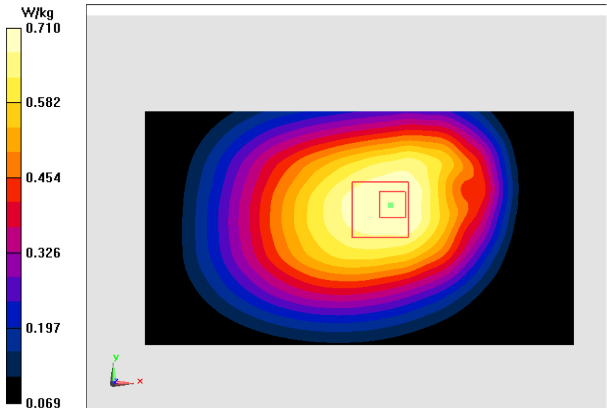
Fig.2 CDMA BC0
