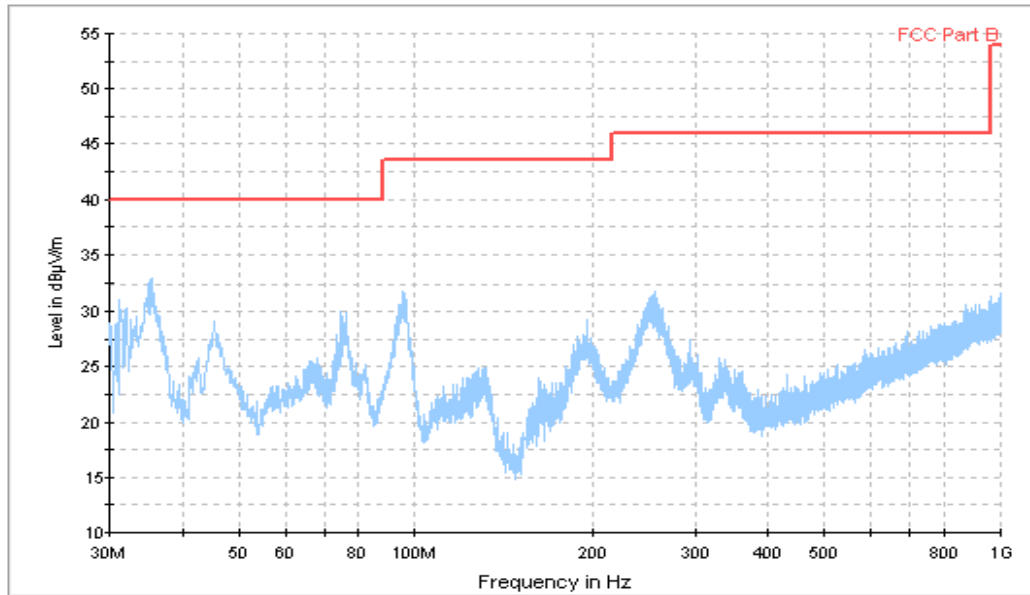
Fig.1 Radiated Emission from 30MHz to 1GHz
