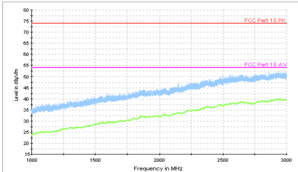
Fig.2 Radiated Emission from 1GHz to 3GHz
