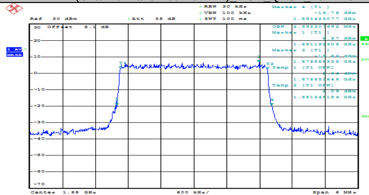
(Channel Bandwidth: 3 MHz) MCH QPSK 15RB#0
