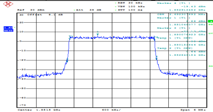
(Channel Bandwidth: 3 MHz) LCH QPSK 15RB#0
