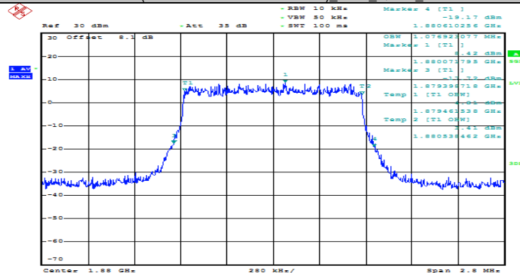
(Channel Bandwidth: 1.4 MHz) MCH_QPSK_6RB#0
