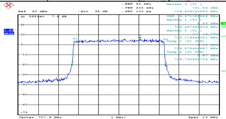
(Channel Bandwidth: 5 MHz) MCH QPSK 25RB#0
