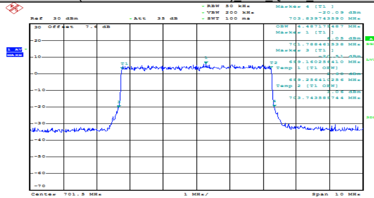
(Channel Bandwidth: 5 MHz) LCH QPSK 25RB#0
