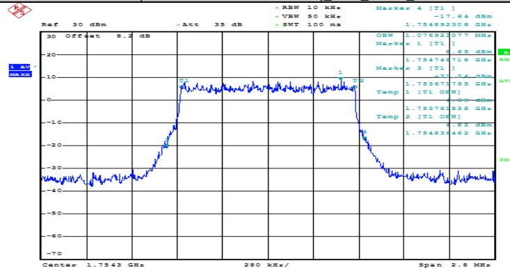
(Channel Bandwidth: 1.4 MHz) HCH_QPSK_6RB#0
