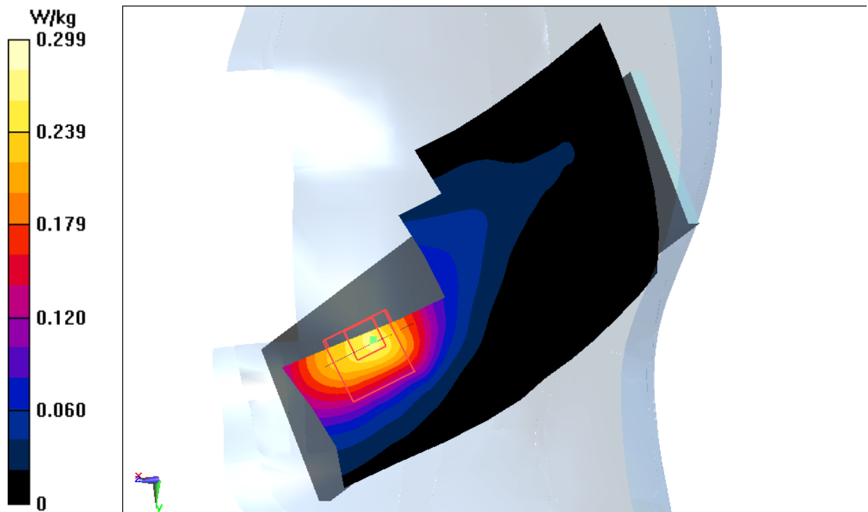
Fig I.3 PCS1900 MHz
