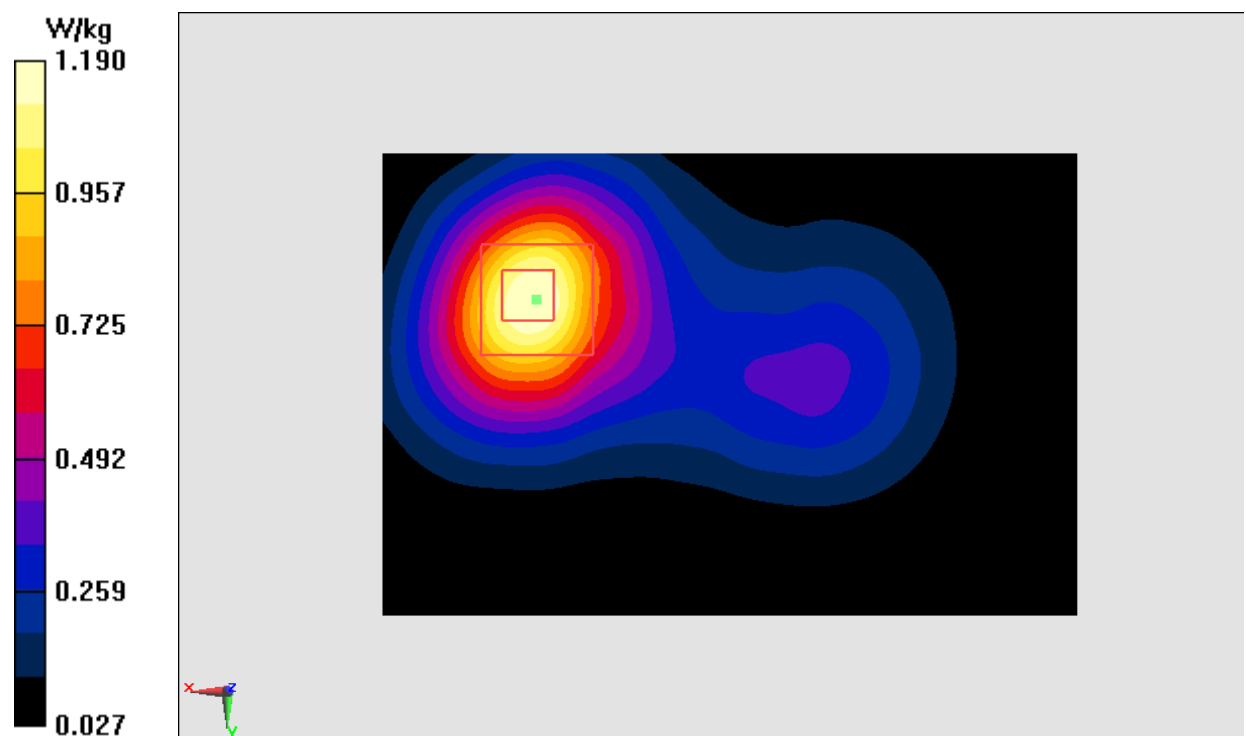
Fig I.4 PCS1900 MHz
