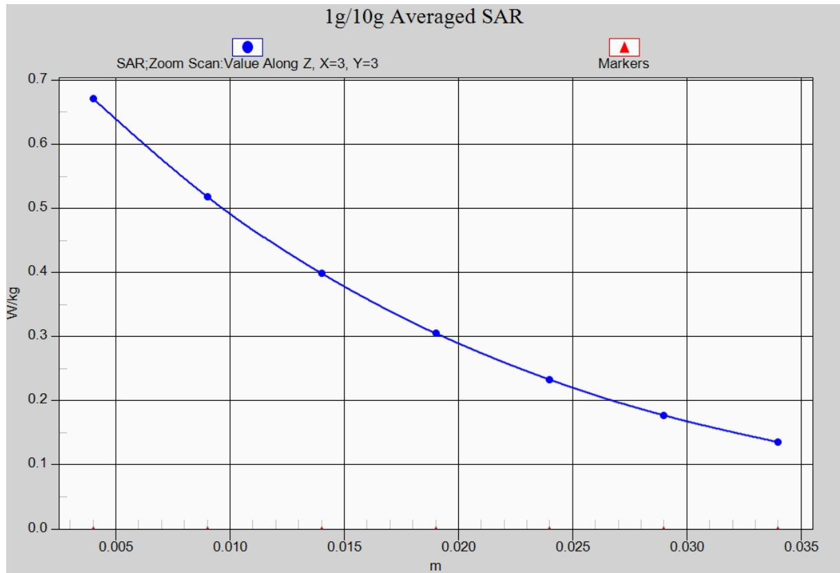
Fig. 21-1 Z-Scan at power reference point (LTE Band26)
