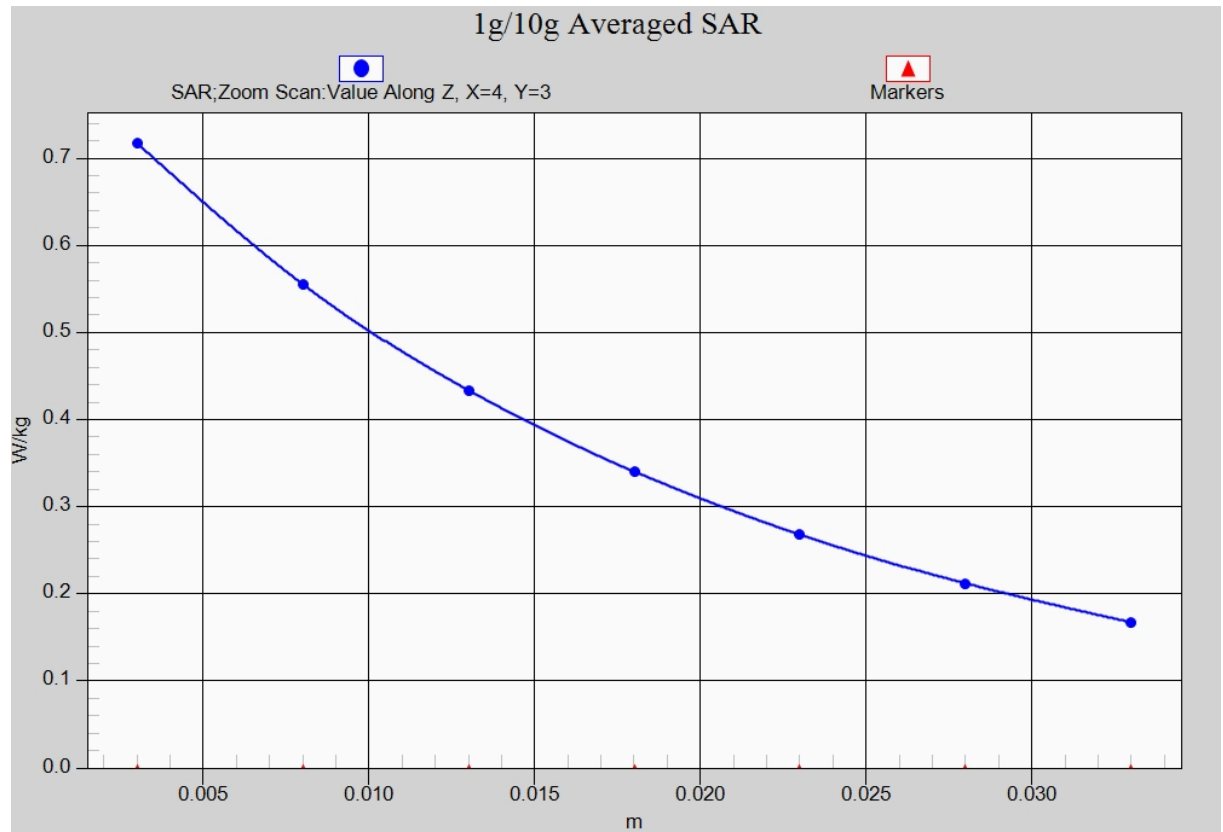
Fig. 20-1 Z-Scan at power reference point (LTE Band26)
