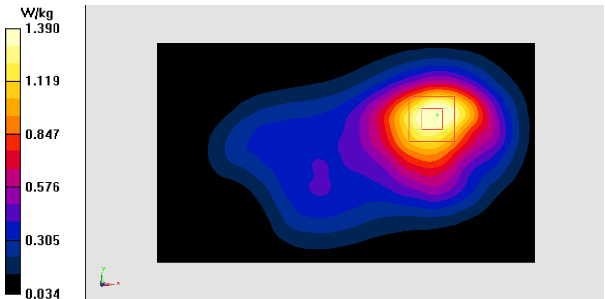
Fig.19 LTE Band 25
