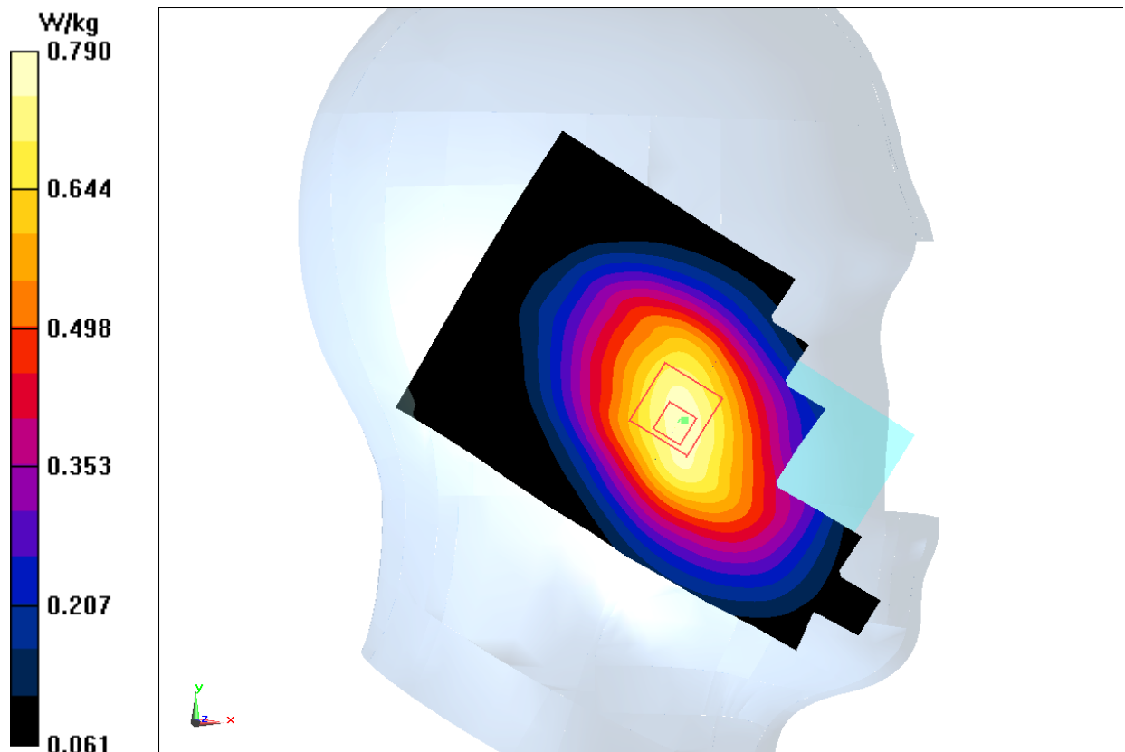
Fig.16 CDMA BC10
