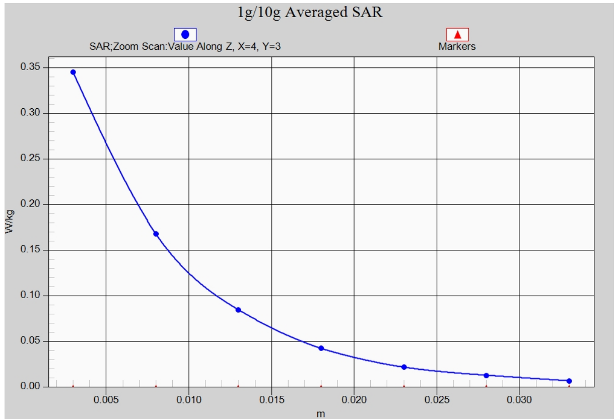
Fig. 22-1 Z-Scan at power reference point (LTE Band 41)
