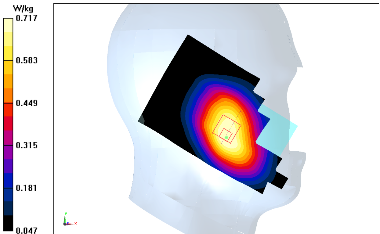
Fig.20 LTE Band 26
