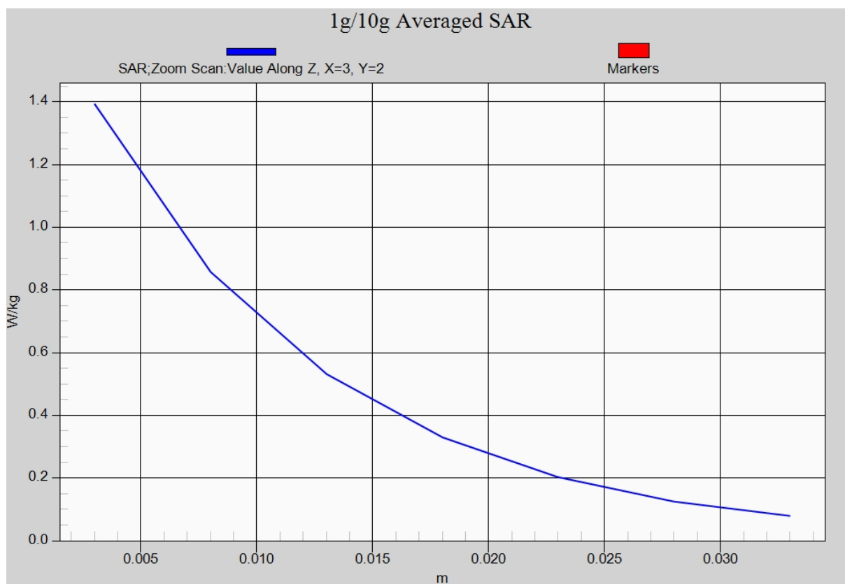
Fig. 19-1 Z-Scan at power reference point (LTE Band25)
