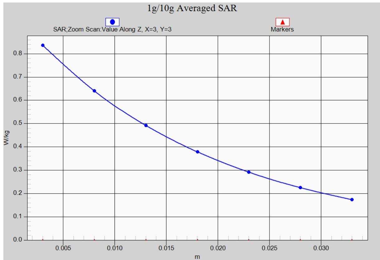
Fig. 11-1 Z-Scan at power reference point (CDMA BC0)
