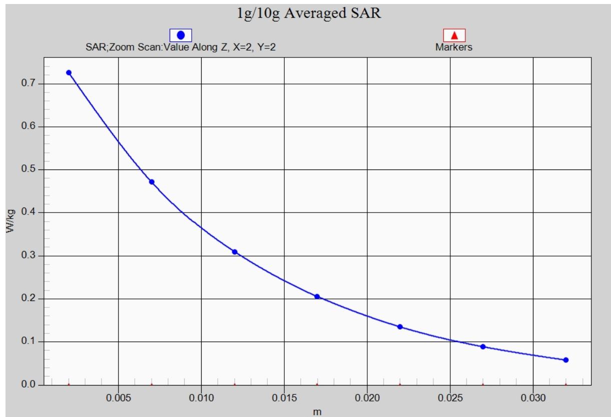
Fig. 13-1 Z-Scan at power reference point (CDMA BC1)
