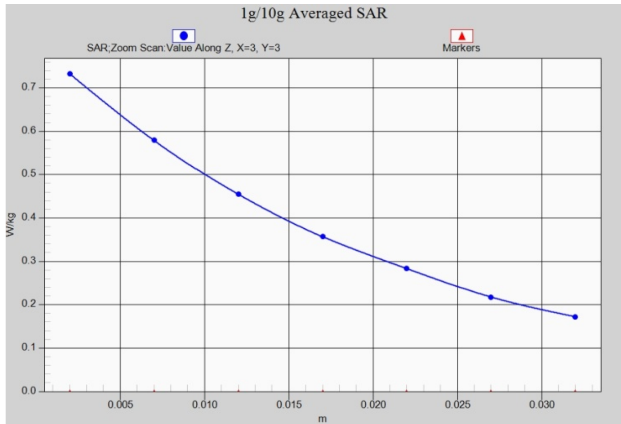
Fig.17-1 Z-Scan at power reference point (CDMA BC10)
