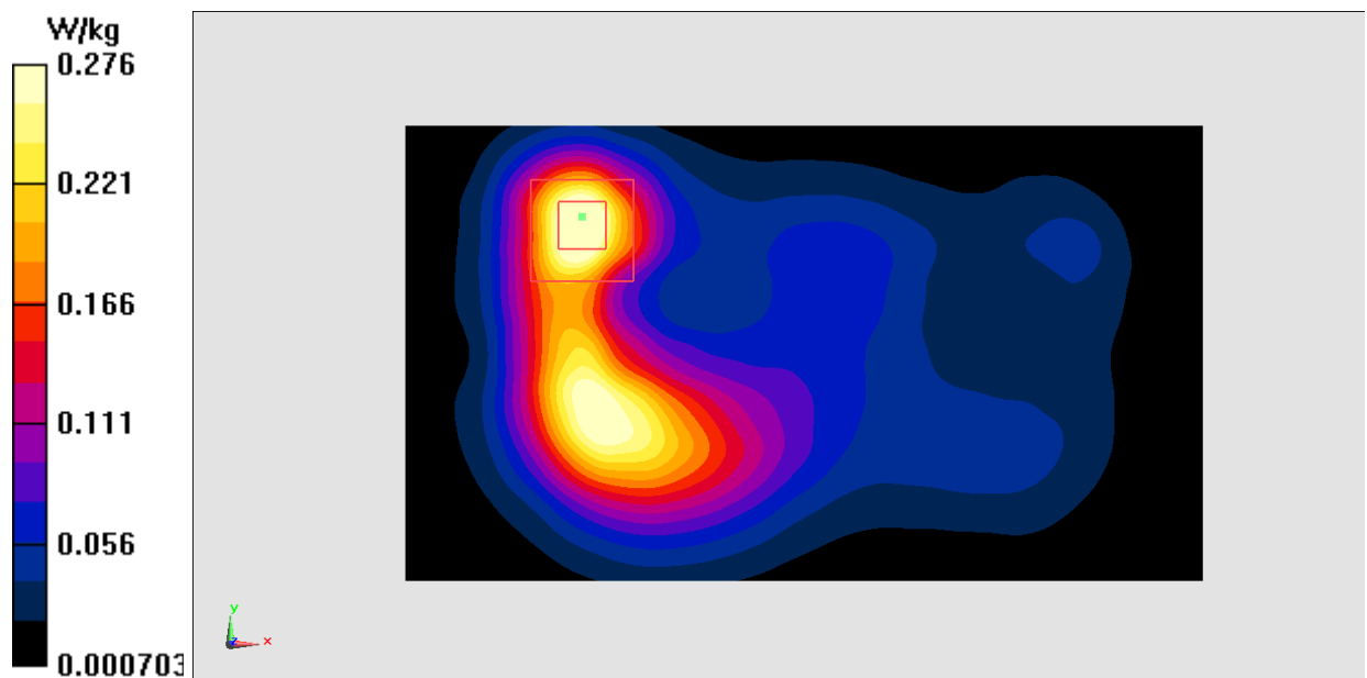
Fig.26 2450 MHz
