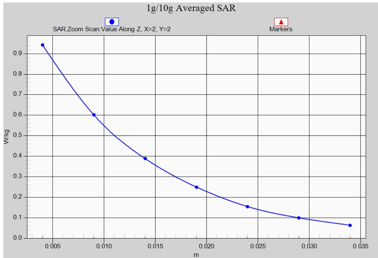
Fig.14-1 Z-Scan at power reference point (CDMA BC1)
