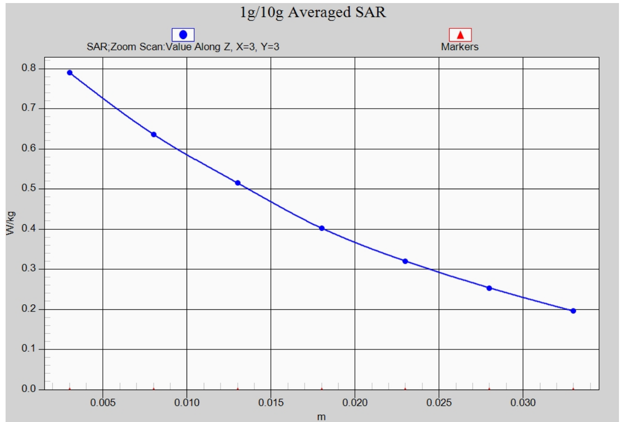
Fig. 16-1 Z-Scan at power reference point (CDMA BC10)
