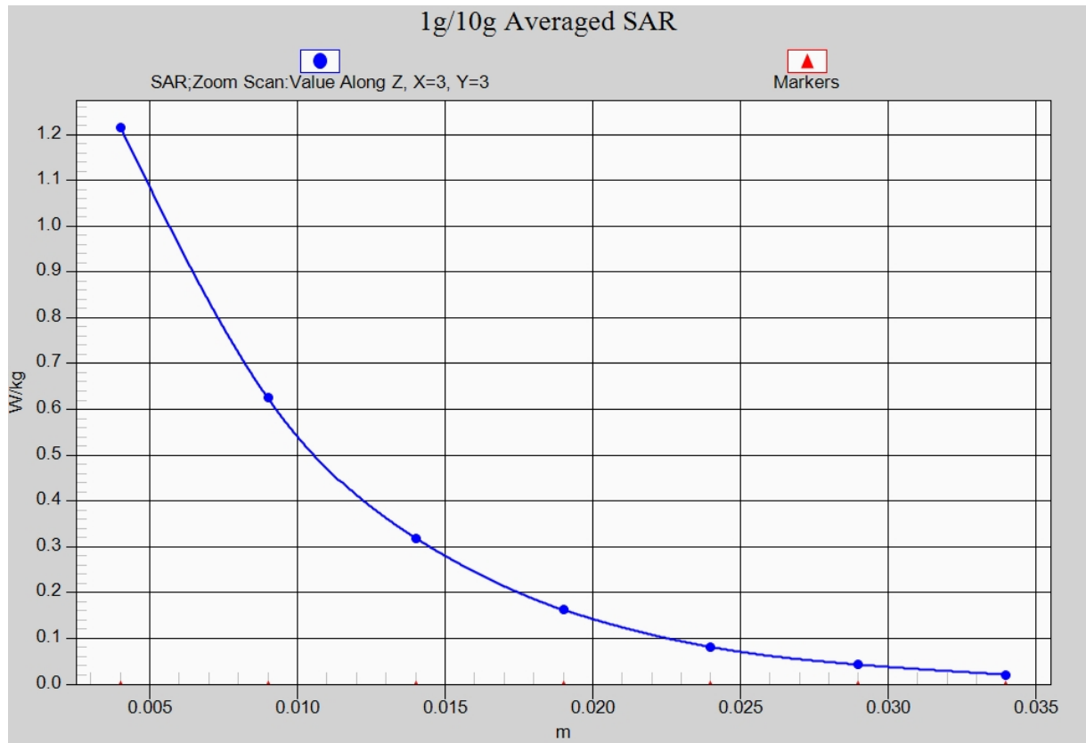
Fig. 23-1 Z-Scan at power reference point (LTE Band 41)
