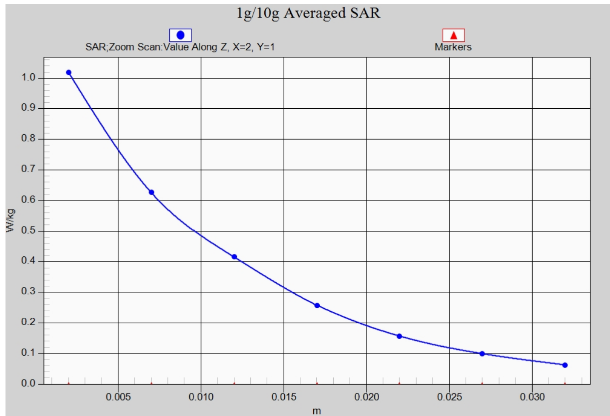
Fig. 18-1 Z-Scan at power reference point (LTE Band25)
