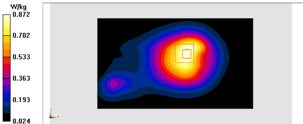
Fig.8 1700 MHz
