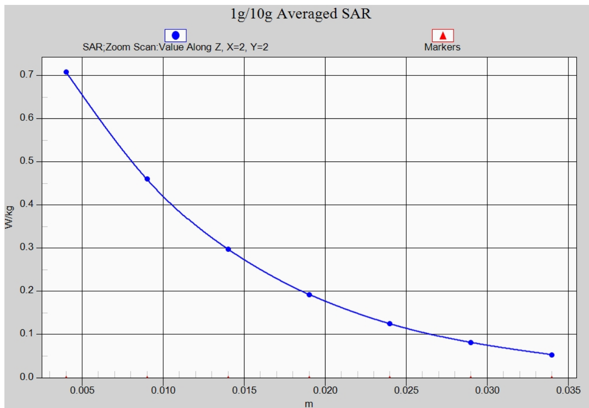
Fig.15-1 Z-Scan at power reference point (CDMA BC1)
