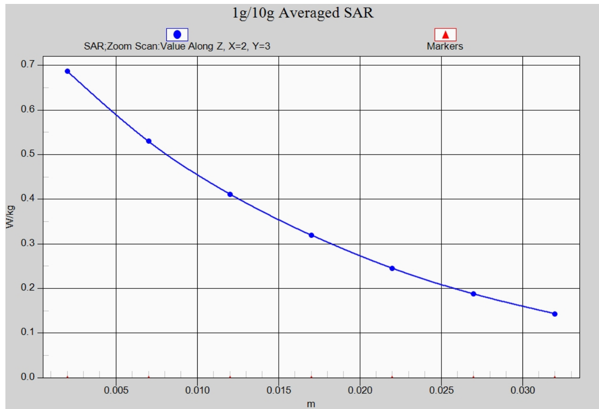
Fig. 12-1 Z-Scan at power reference point (CDMA BC0)
