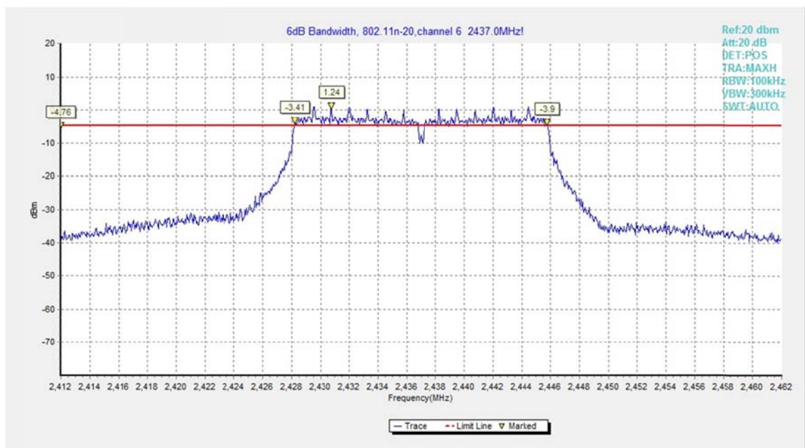
Fig.A.4.8 Occupied 6dB Bandwidth (802.11n-HT20, Ch 6)
