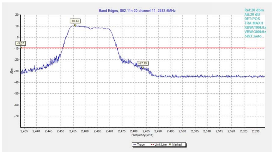
Fig.A.5.6 Band Edges (802.11n-HT20, Ch 11)
