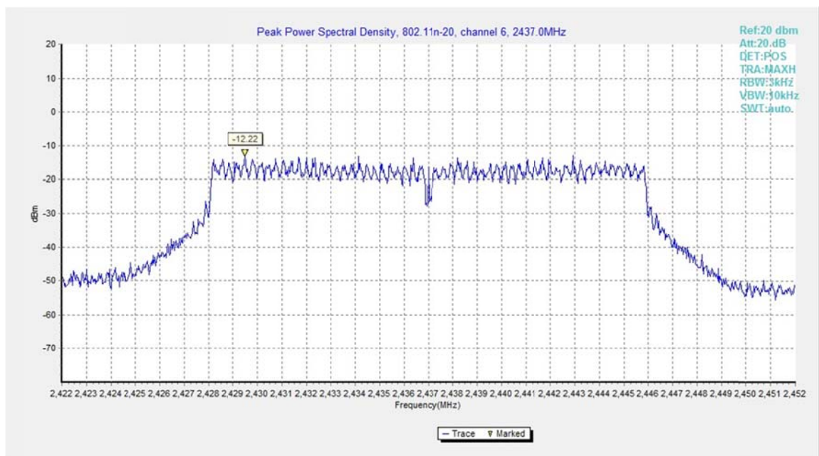
Fig.A.3.8 Power Spectral Density (802.11n-HT20, Ch 6)
