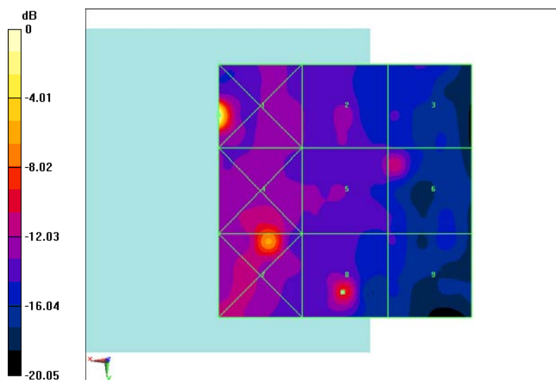
Fig B.14 HAC RF E-Field CDMA 835 Middle
