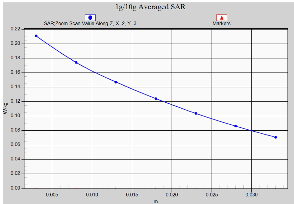
Fig. 20-1 Z-Scan at power reference point (LTE Band17)
