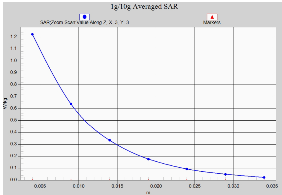
Fig. 19-1 Z-Scan at power reference point (LTE Band7) AP ON
