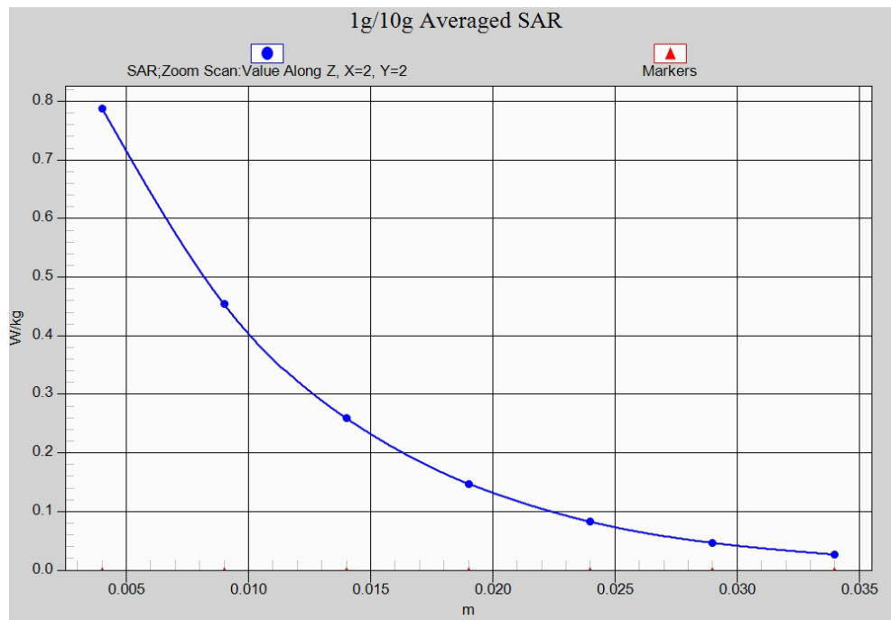
Fig. 18-1 Z-Scan at power reference point (LTE Band7) AP OFF
