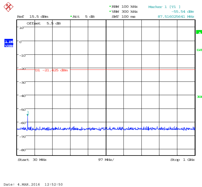
Fig.4. Transmitter Spurious Emission - Conducted: GFSK, 2402 MHz, 30MHz - 1GHz
