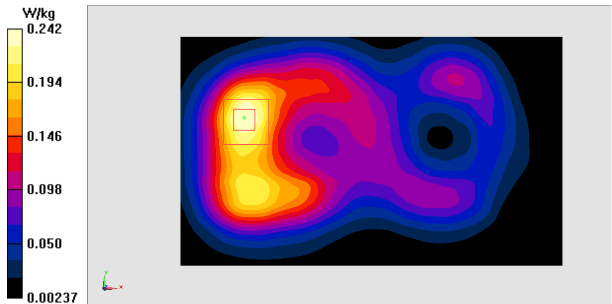
Fig.21 2450 MHz
