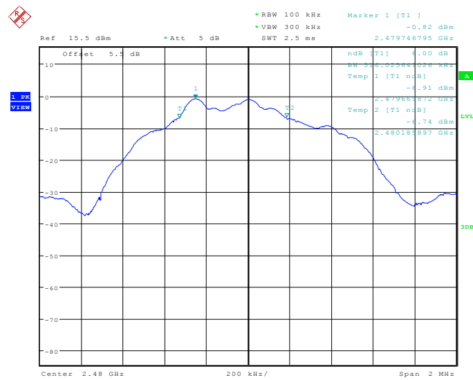
Fig.31. 6dB Bandwidth: GFSK, 2480 MHz
