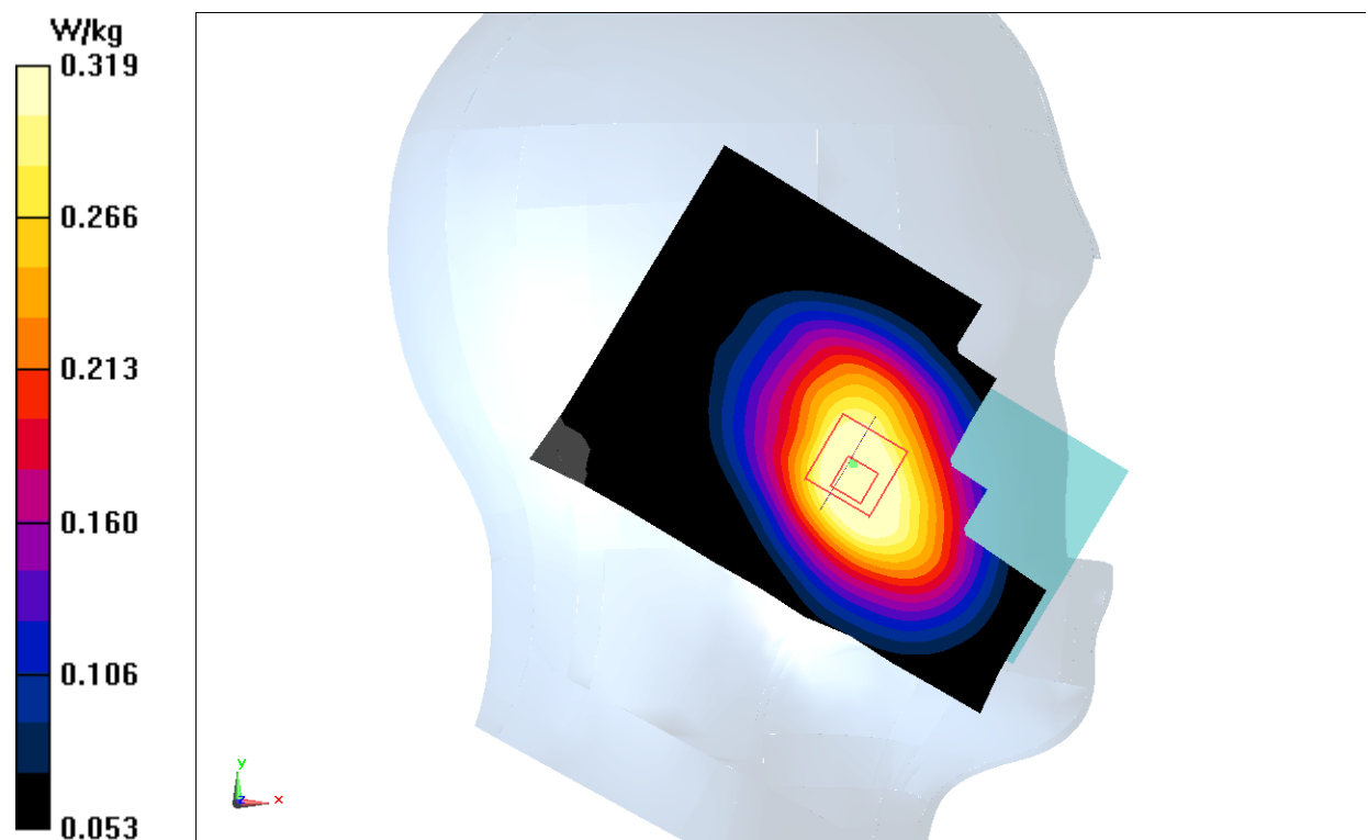
Fig.17 LTE Band12
