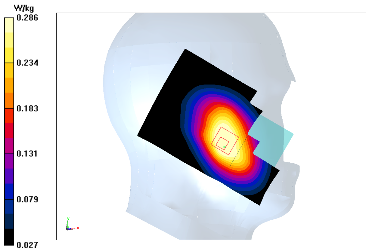
Fig.8 LTE Band5
