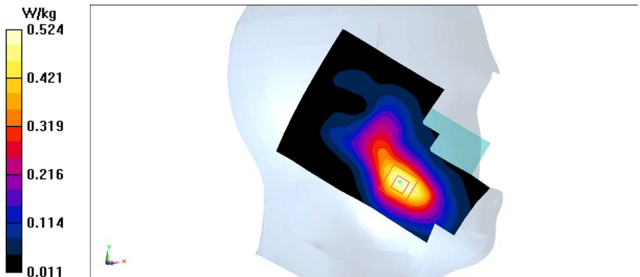
Fig.7 LTE Band4
