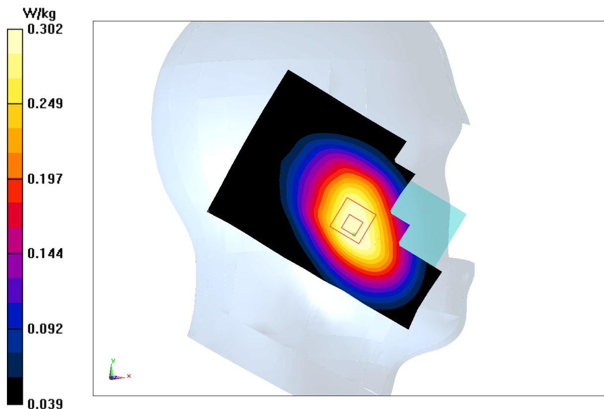
Fig.9 LTE Band12
