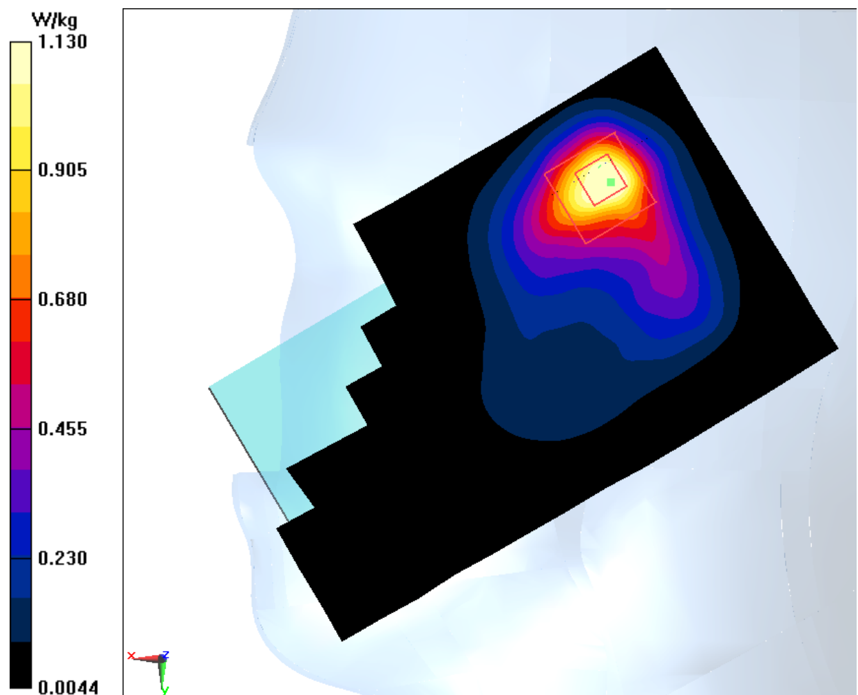
Fig.10 2450 MHz
