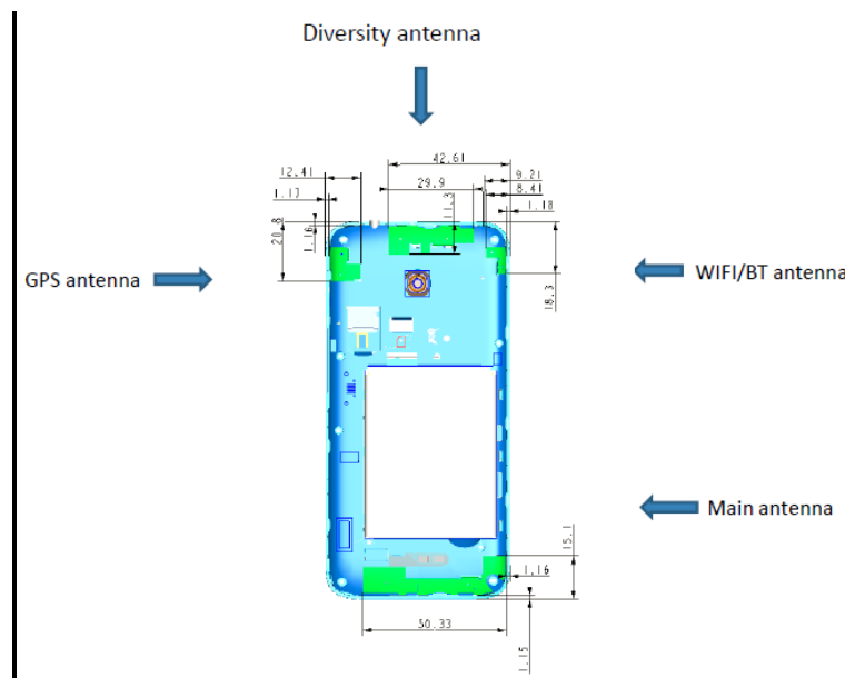
Picture 12.1 Antenna Locations
