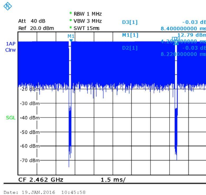
Picture 14.1 The plot of duty factor
