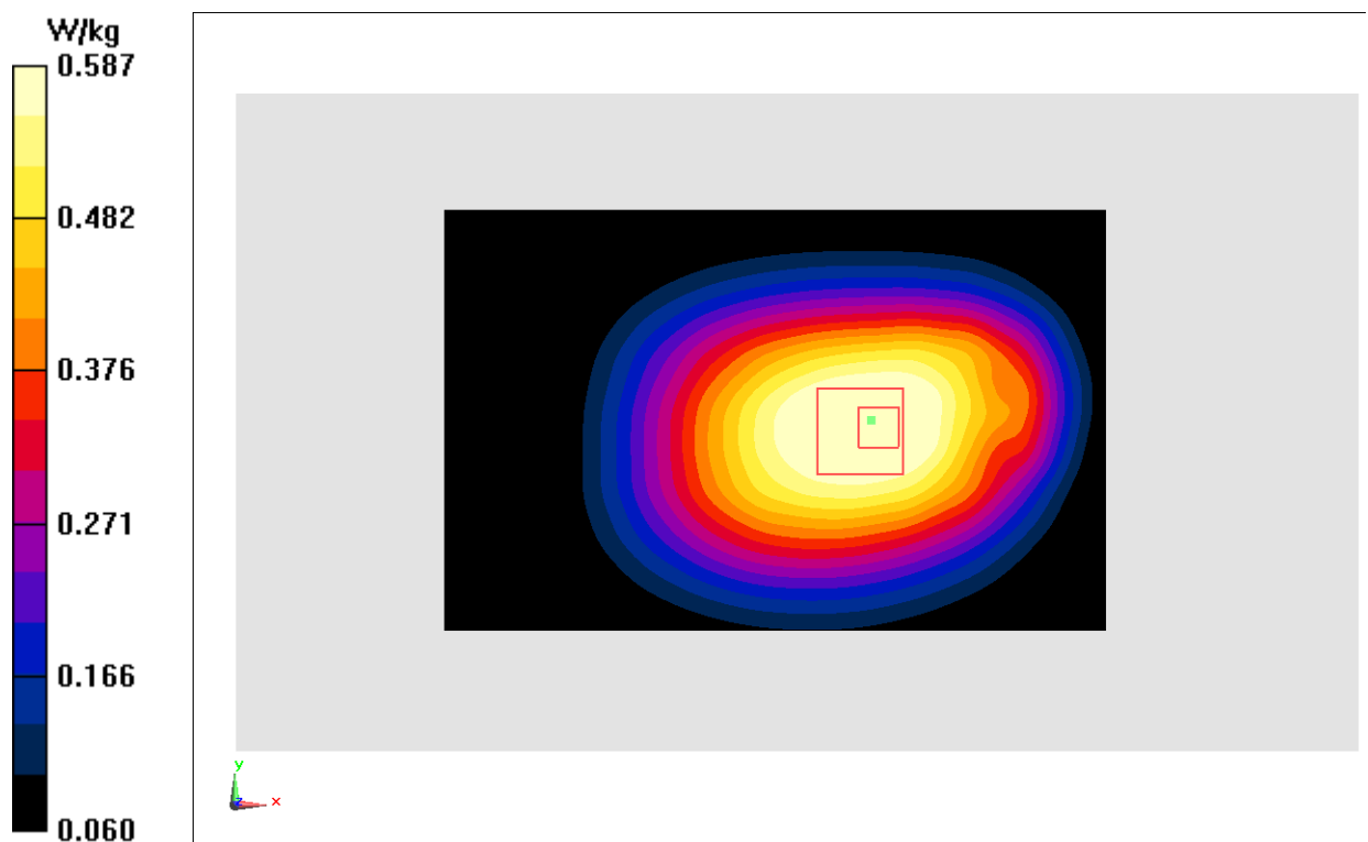
Fig.2 850 MHz
