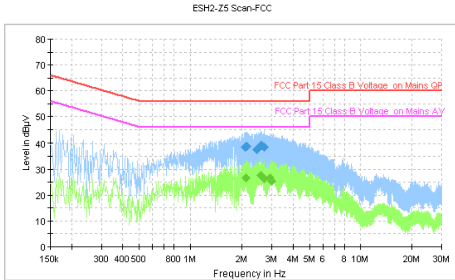
Fig. 100 AC Power line Conducted Emission (Idle, AE1)
