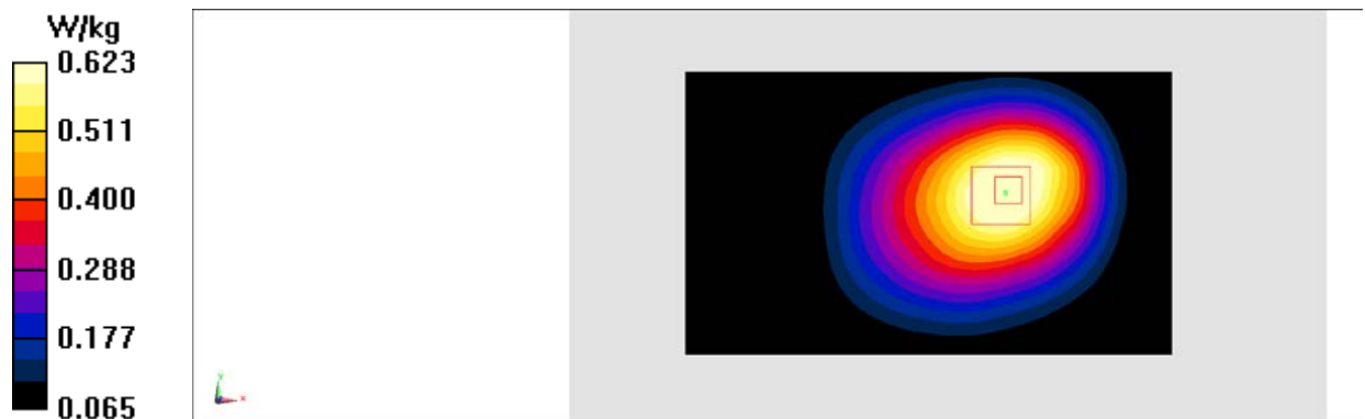
Fig.8 LTE Band 13
