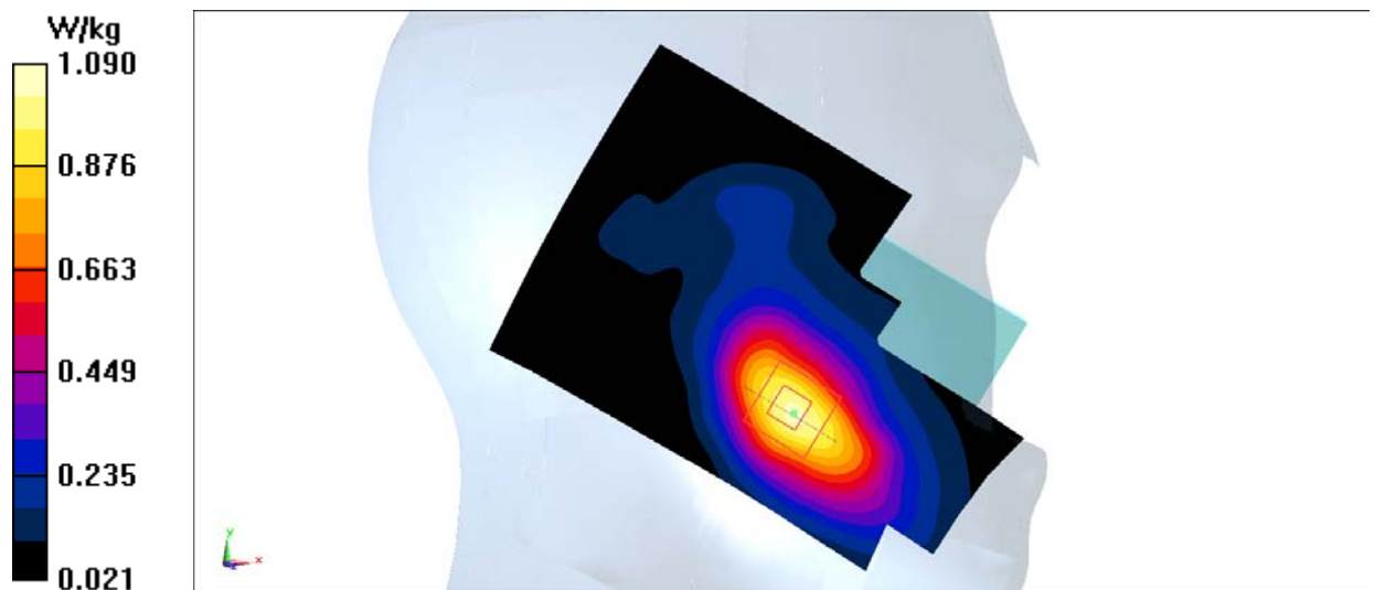
Fig.5 LTE Band4
