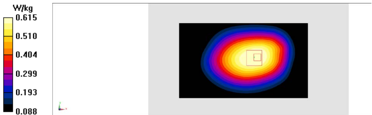
Fig.2 CDMA BC0
