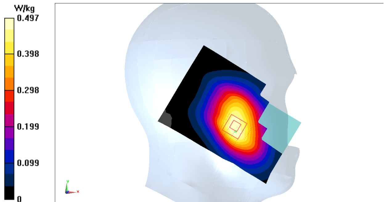
Fig.7 LTE Band 13
