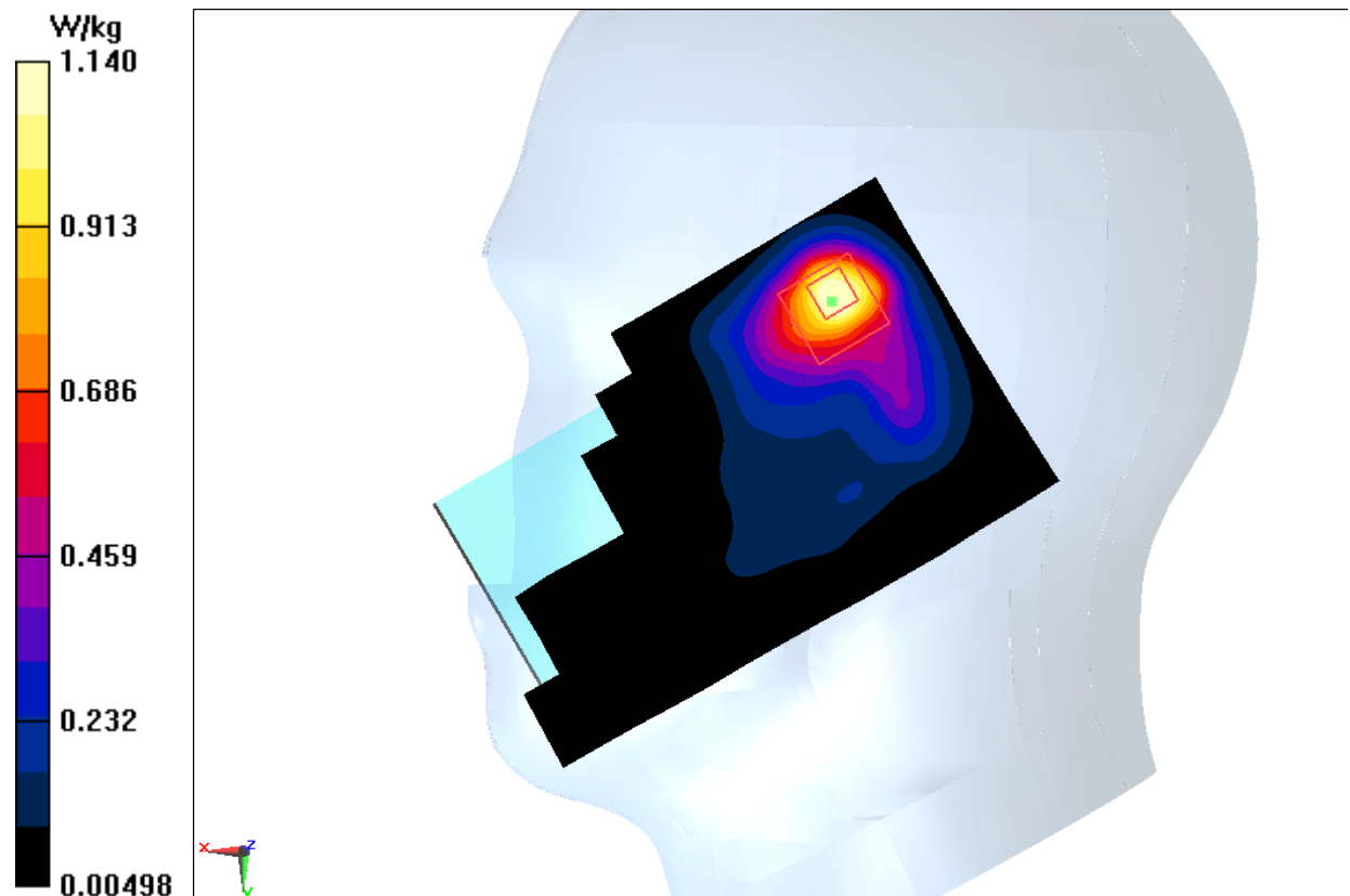
Fig.9 2450 MHz
