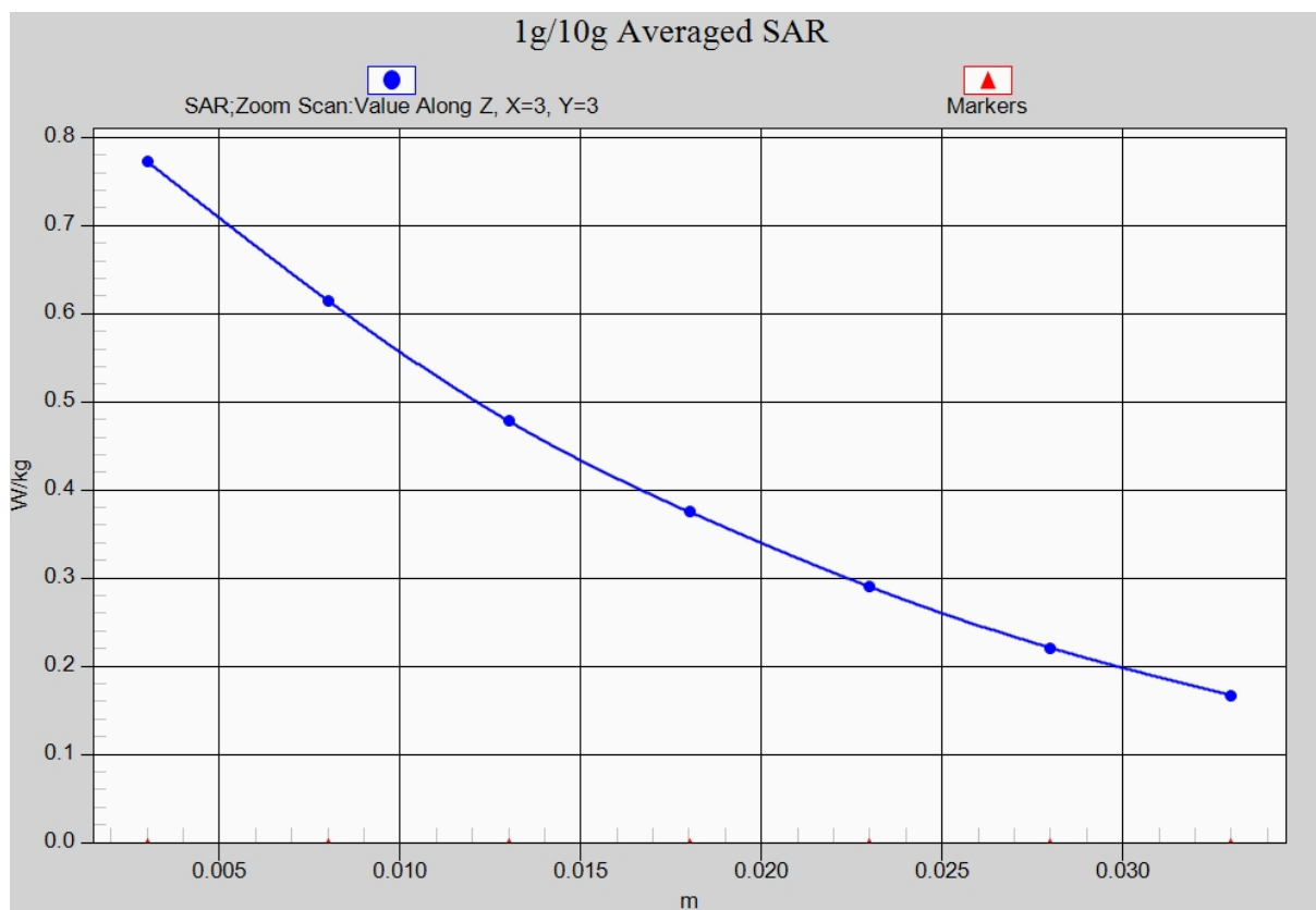
Fig. 5-1 Z-Scan at power reference point (CDMA BC10)
