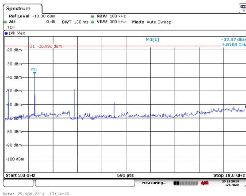
Fig. 36 Conducted Spurious Emission ( \pi/4 DQPSK, Ch39, 3GHz-18 GHz)
