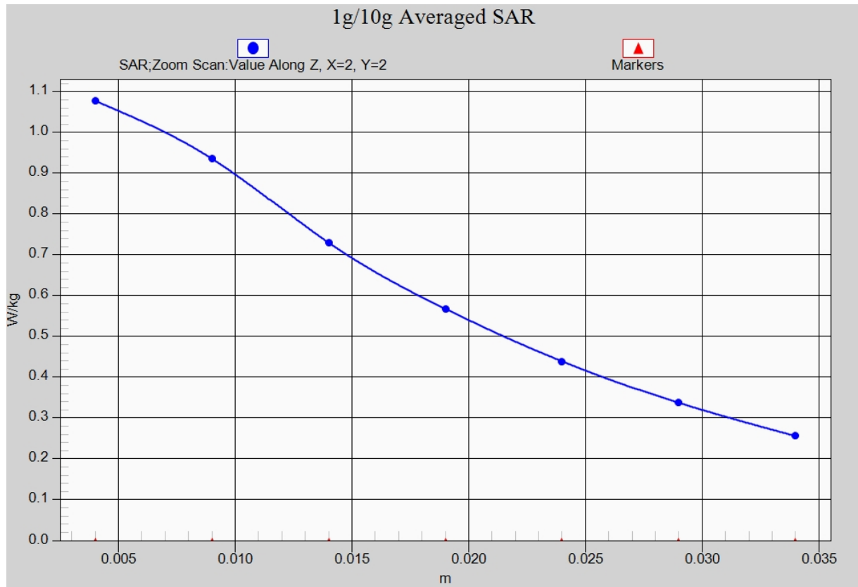
Fig. 6-1 Z-Scan at power reference point (CDMA BC10 CH476)
