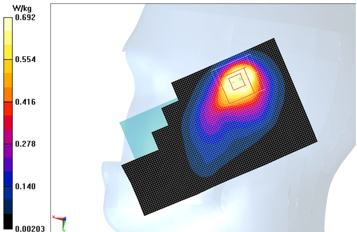
Fig.7 2450 MHz CH6
