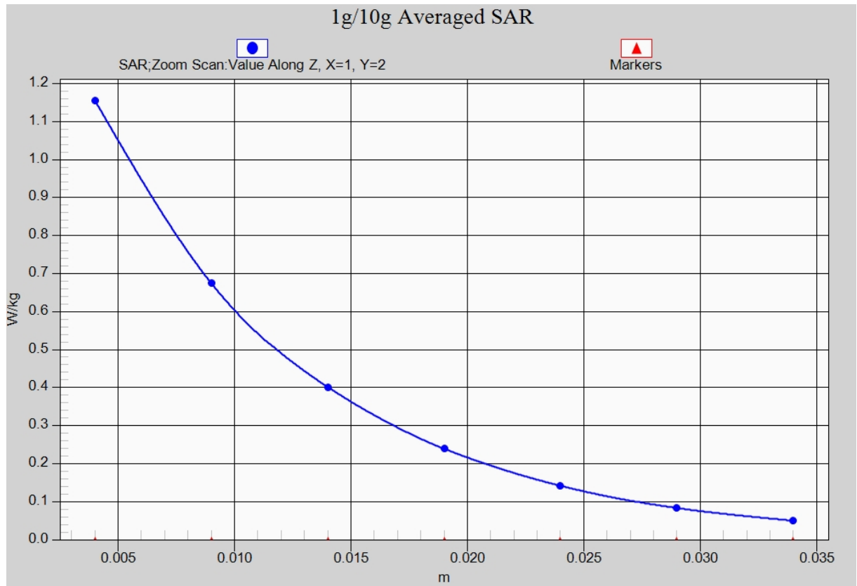
Fig.4-1 Z-Scan at power reference point (CDMA BC1 CH600)
