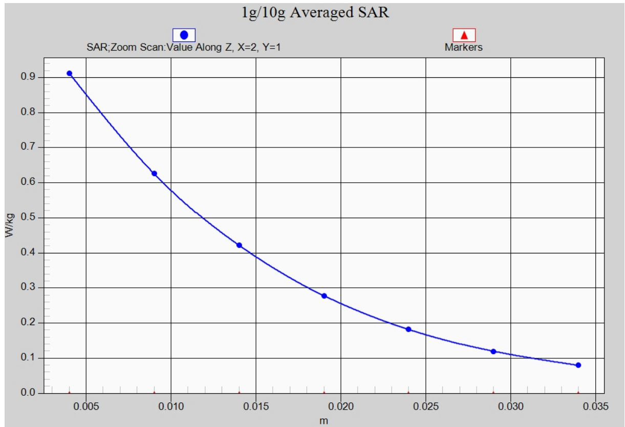
Fig. 3-1 Z-Scan at power reference point (CDMA BC1 CH600)
