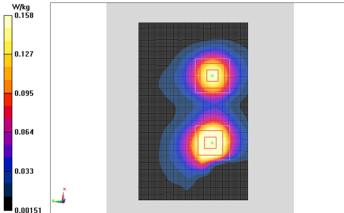
Fig.8 2450 MHz CH6
