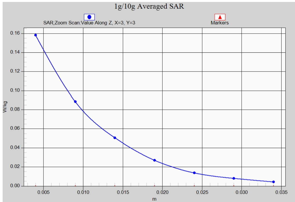
Fig. 8-1 Z-Scan at power reference point (2450 MHz CH6)
