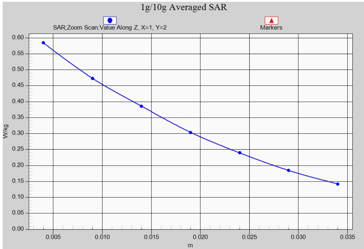
Fig. 5-1 Z-Scan at power reference point (CDMA BC10 CH476)
