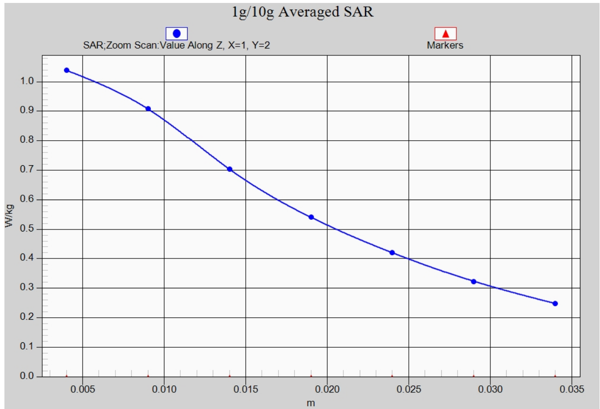
Fig. 2-1 Z-Scan at power reference point (CDMA BC0 CH1013)
