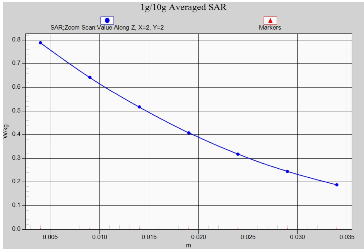
Fig. 1-1 Z-Scan at power reference point (CDMA BC0 CH777)
