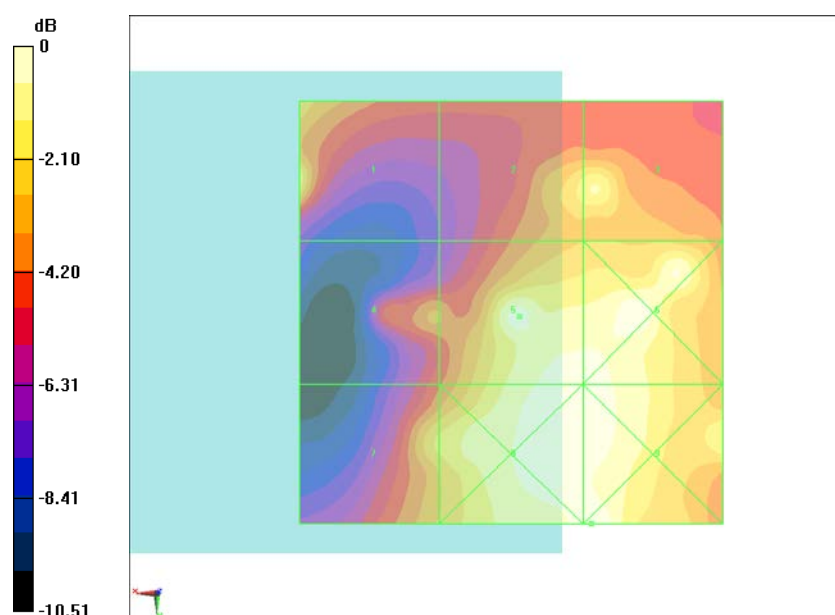
Fig B.4 HAC RF E-Field CDMA BC1 High
