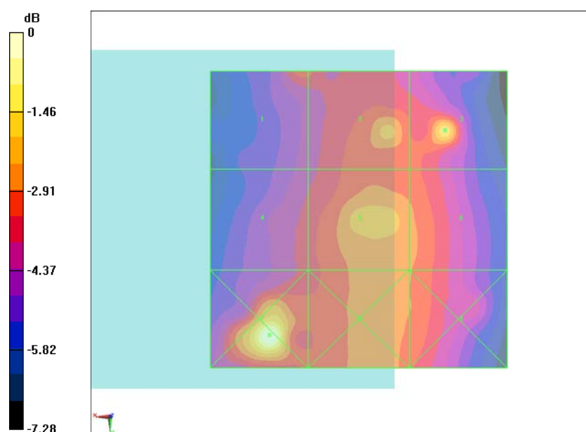
Fig B.9 HAC RF E-Field CDMA BC10 Low
