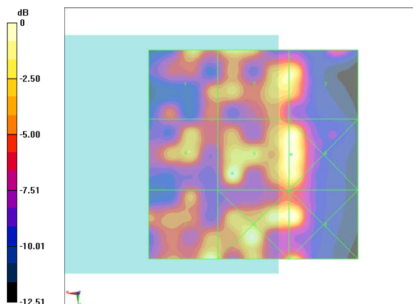
Fig B.7 HAC RF E-Field CDMA BC10 High
