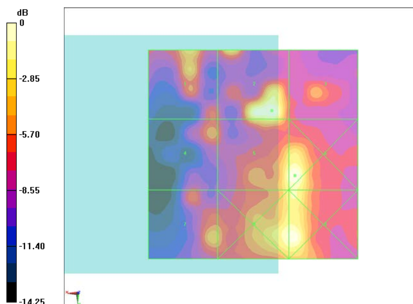
Fig B.5 HAC RF E-Field CDMA BC1 Middle
