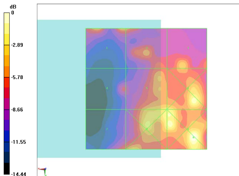
Fig B.6 HAC RF E-Field CDMA BC1 Low
