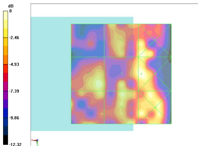
Fig B.8 HAC RF E-Field CDMA BC10 Middle
