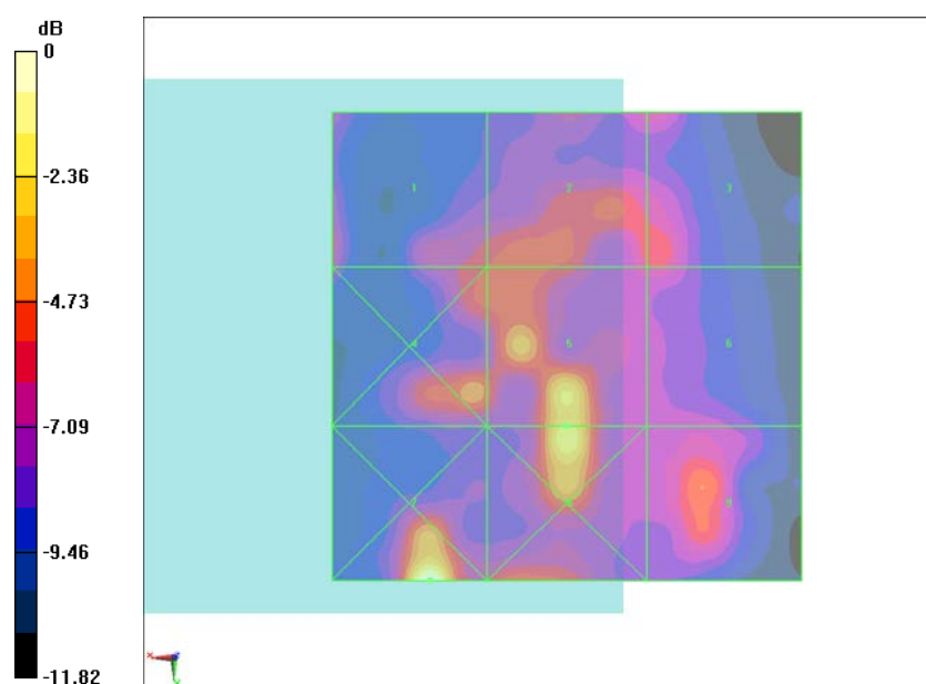
Fig B.3 HAC RF E-Field CDMA BC0 Low
