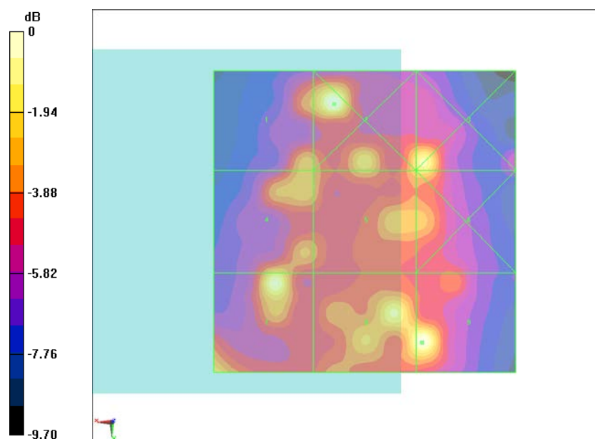
Fig B.2 HAC RF E-Field CDMA BC0 Middle
