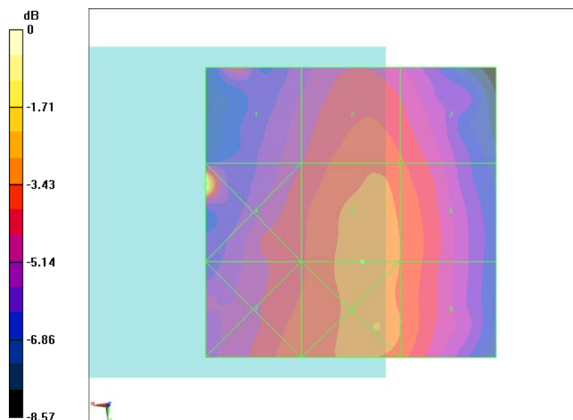
Fig B.1 HAC RF E-Field CDMA BC0 High
