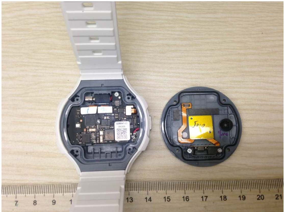
Watch Disassembly
