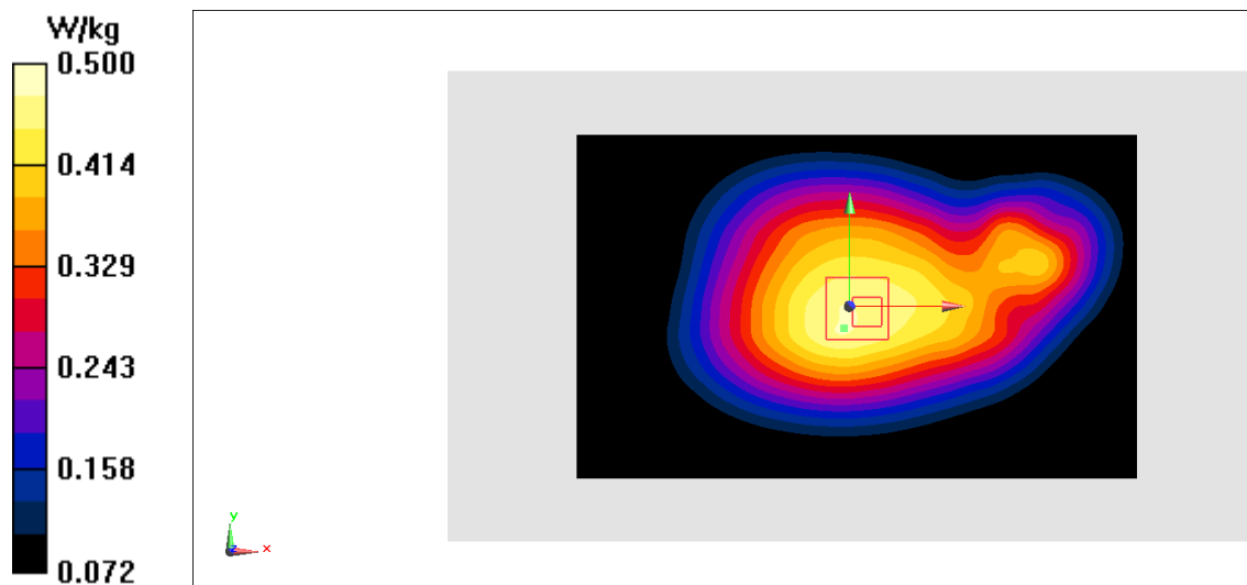
Fig.2 850 MHz
