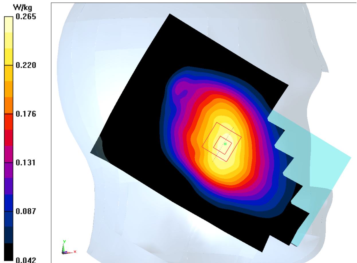
Fig.1 850MHz
