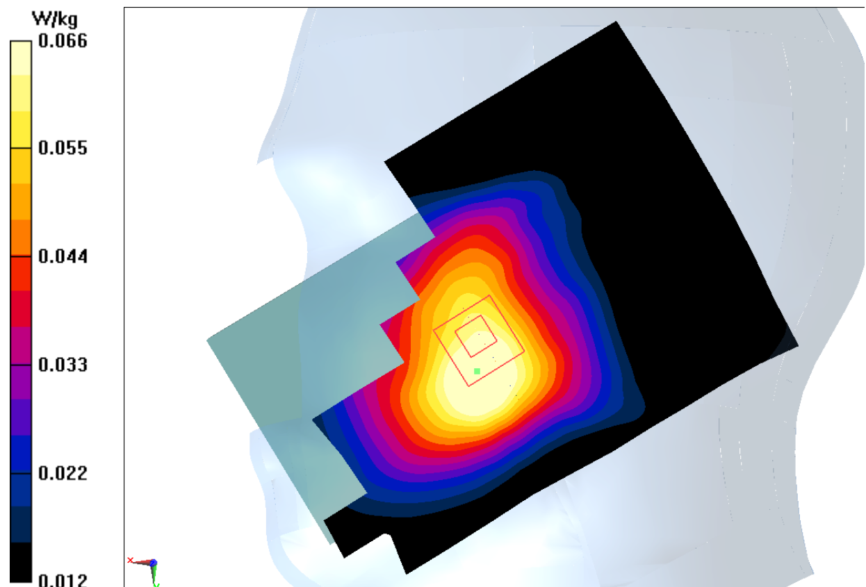
Fig.20 LTE Band12
