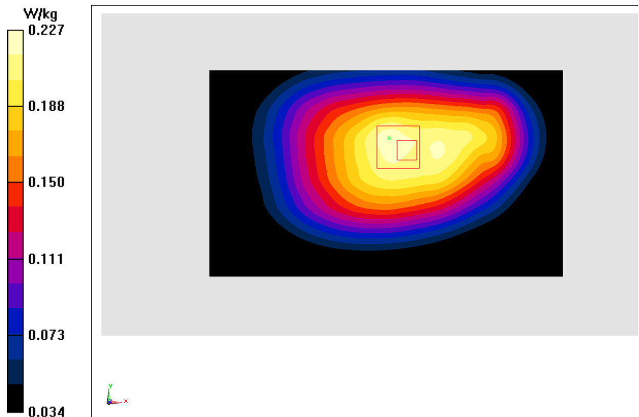
Fig.23 LTE Band17
