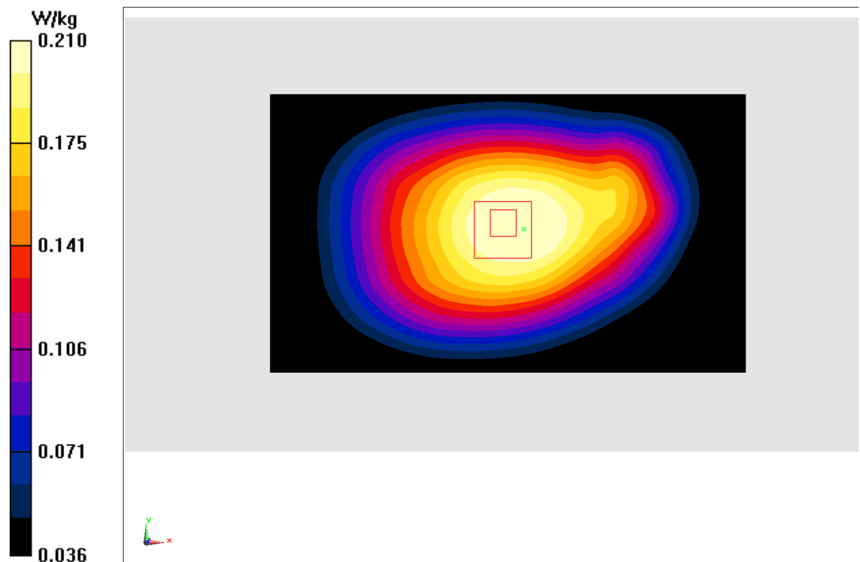
Fig.21 LTE Band12
