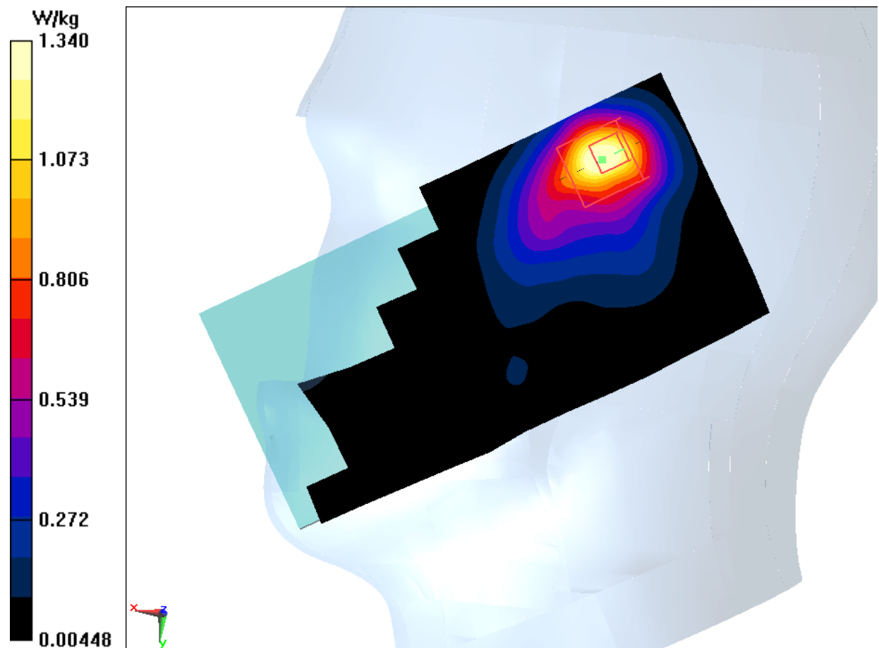
Fig.24 2450 MHz
