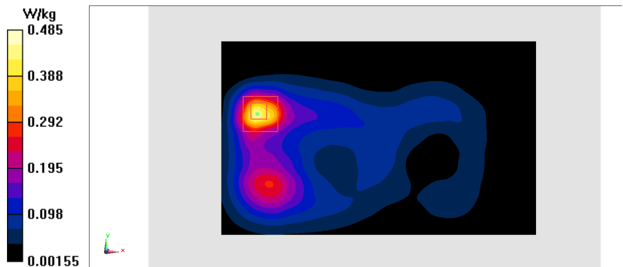
Fig.25 2450 MHz
