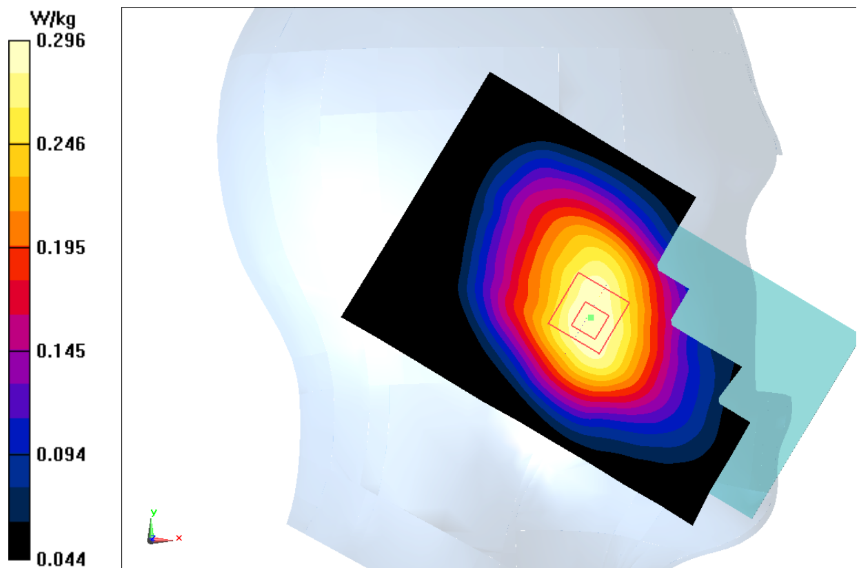
Fig.1 850MHz
