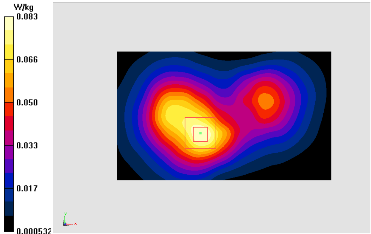
Fig.10 2450 MHz
