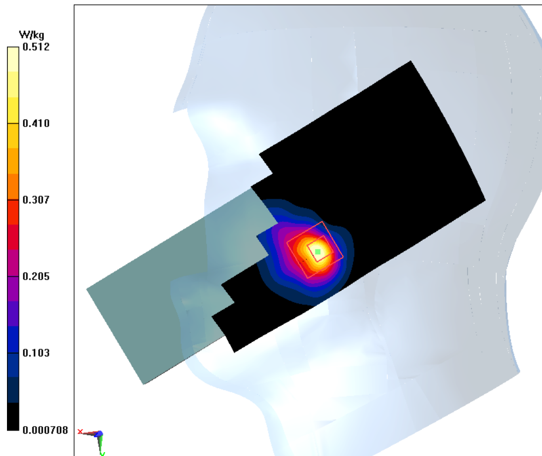
Fig.9 2450 MHz
