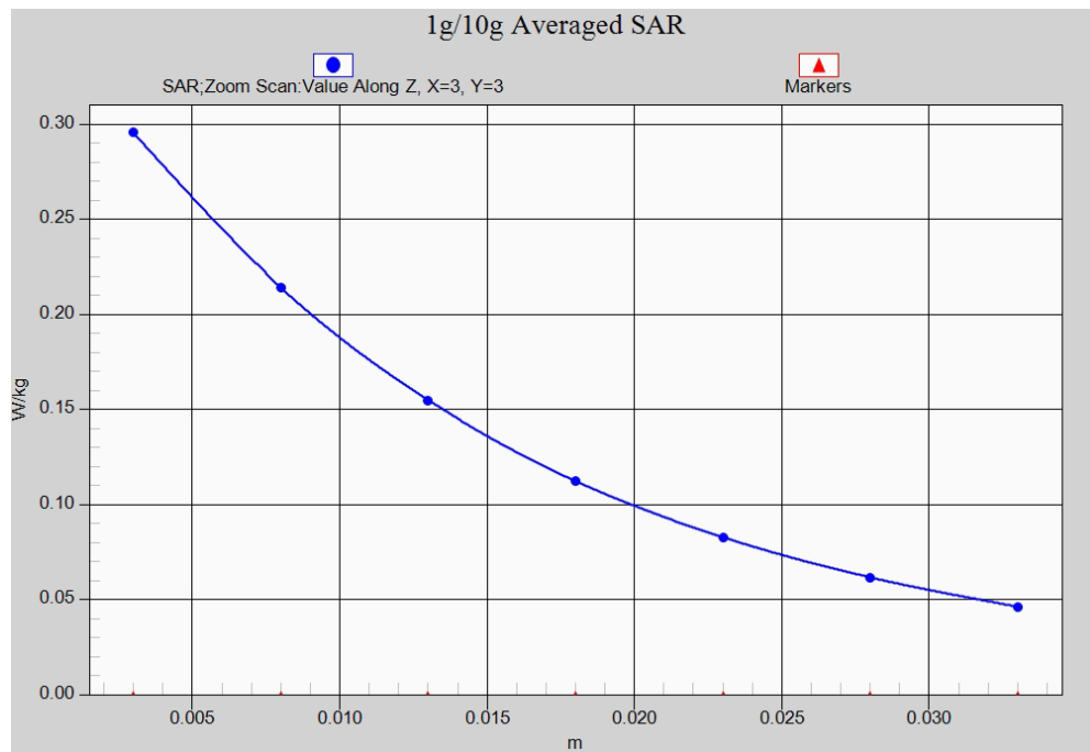
Fig. 7-1 Z-Scan at power reference point (LTE Band13)
