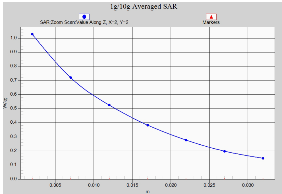
Fig. 8-1 Z-Scan at power reference point (LTE Band13)
