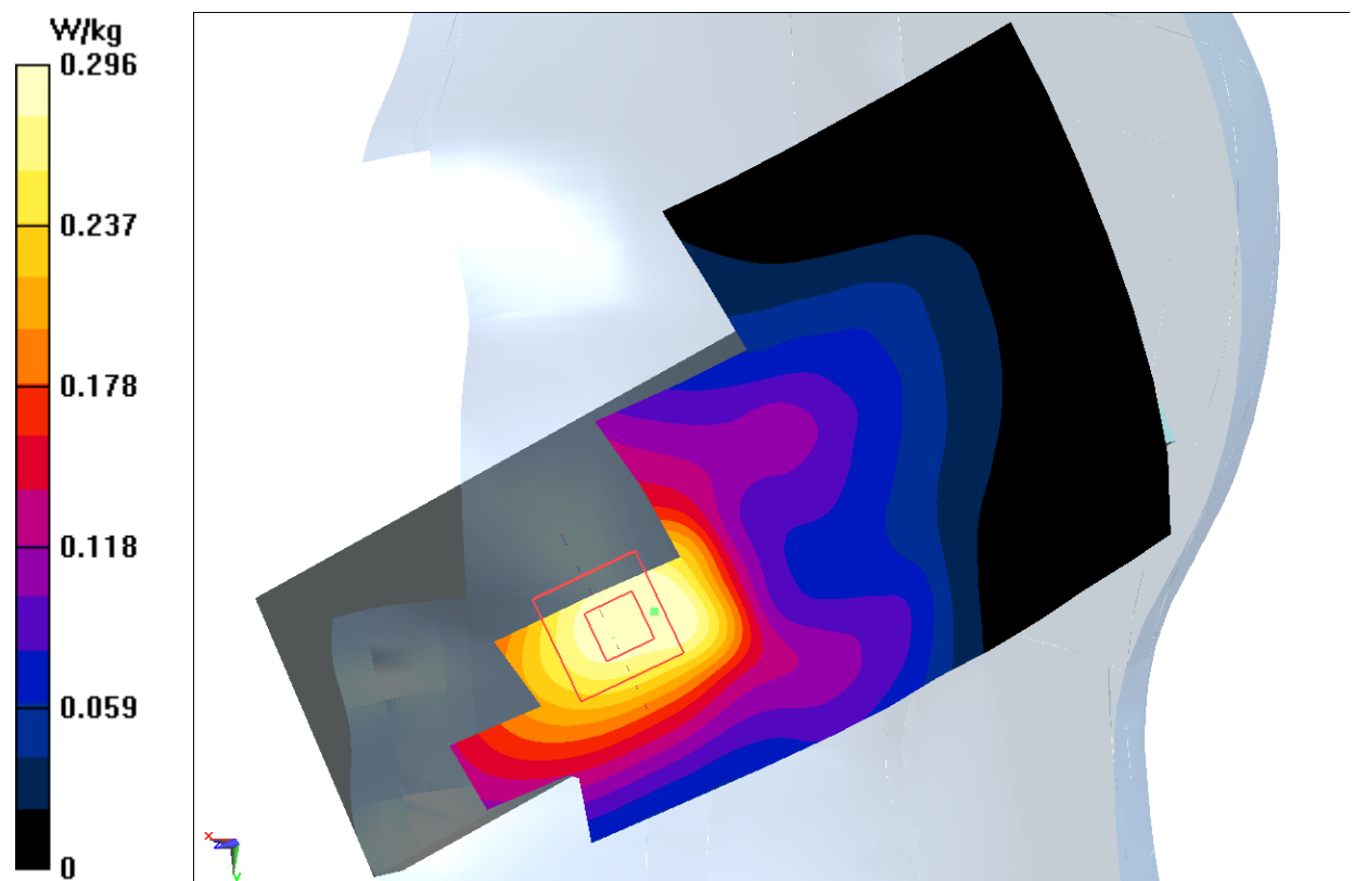
Fig.7 LTE Band 13
