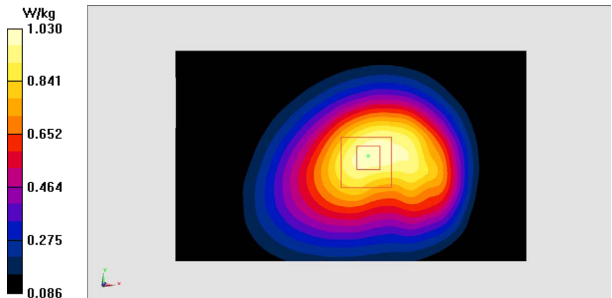
Fig.8 LTE Band 13
