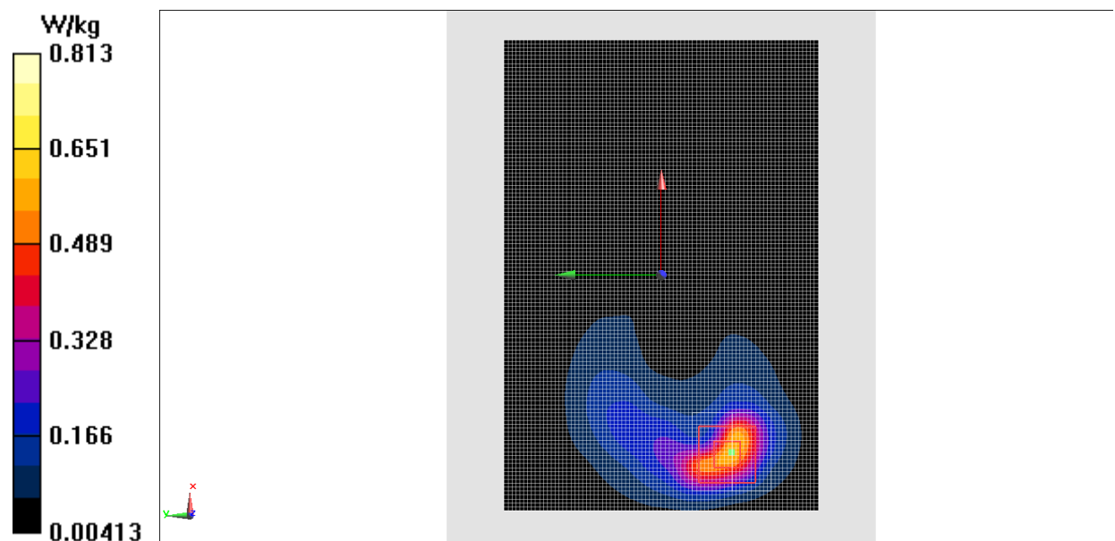
Fig.16 2450 MHz
