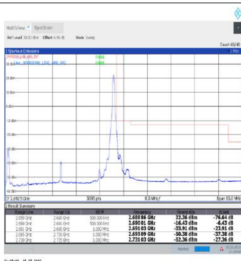
1-N41-30-40-H-2-DFT-PI2BPSK-Edge_1RB_Right-1@105-Ant1-PASS-see graph
