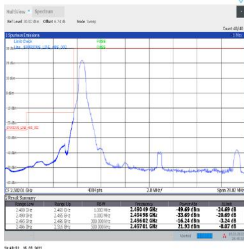
1-N41-30-20-L-4-CP-QPSK-Edge_1RB_Left-1@0-Ant1-PASS-see graph
