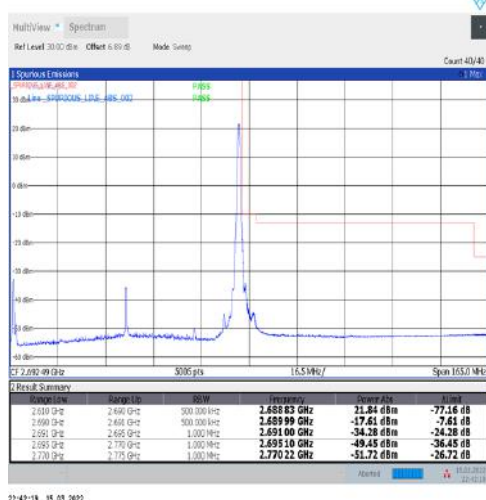
1-N41-30-80-H-5-CP-QPSK-Edge_1RB_Right-1@216-Ant1-PASS-see graph
