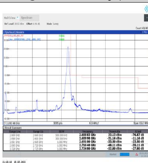
1-N41-30-30-H-5-CP-QPSK-Edge_1RB_Right-1@77-Ant1-PASS-see graph
