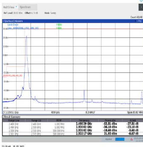
1-N41-30-70-L-4-CP-QPSK-Edge_1RB_Left-1@0-Ant1-PASS-see graph
