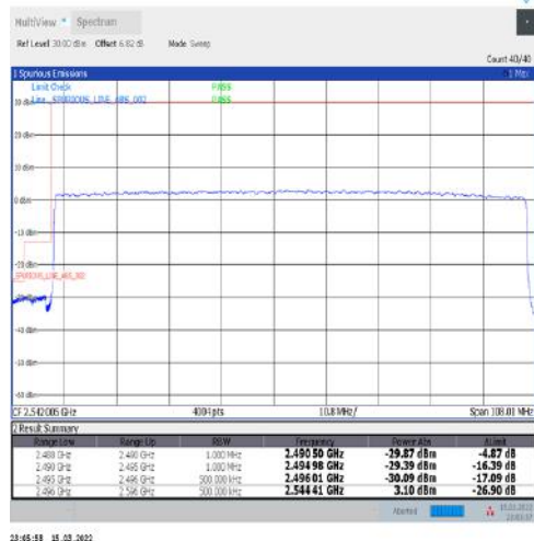
1-N41-30-100-L-3-DFT-PI2BPSK-Outer_Full-270@0-Ant1-PASS-see graph
