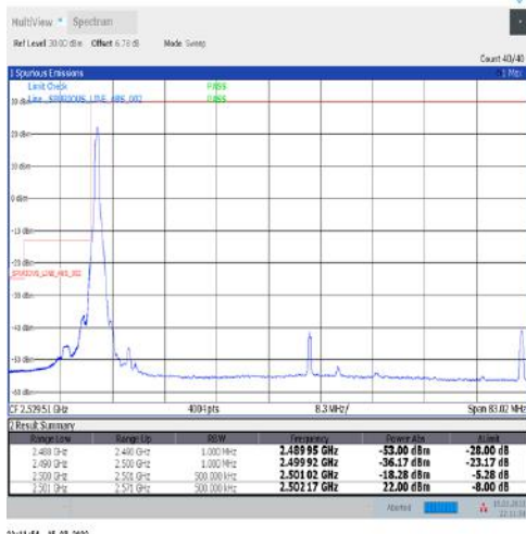
1-N41-30-70-L-1-DFT-PI2BPSK-Edge_1RB_Left-1@0-Ant1-PASS-see graph
