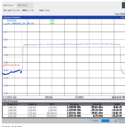
1-N41-30-70-L-3-DFT-PI2BPSK-Outer_Full-180@0-Ant1-PASS-see graph
