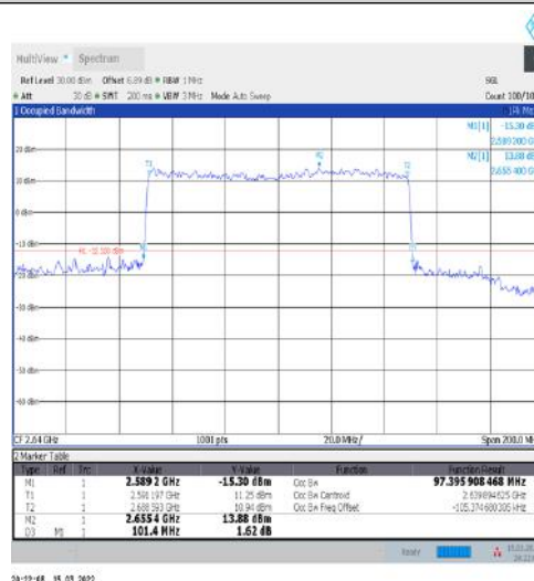
1-N41-30-100-H-6-CP-QPSK-Outer_Full-273@0-Ant1-97.396-101.400-≤100-PASS
