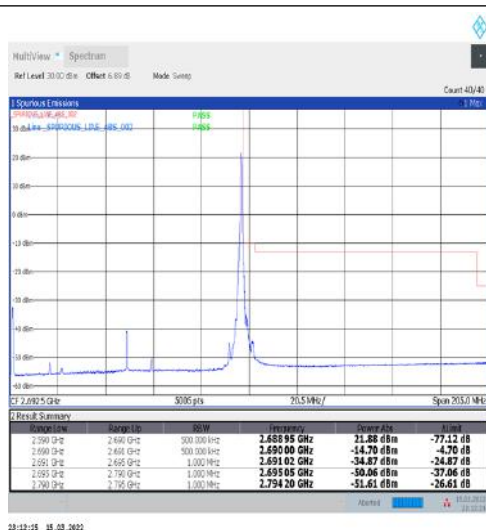
1-N41-30-100-H-2-DFT-PI2BPSK-Edge_1RB_Right-1@272-Ant1-PASS-see graph
