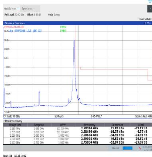
1-N41-30-70-H-5-CP-QPSK-Edge_1RB_Right-1@188-Ant1-PASS-see graph
