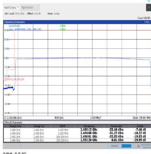
1-N41-30-100-L-6-CP-QPSK-Outer_Full-273@0-Ant1-PASS-see graph
