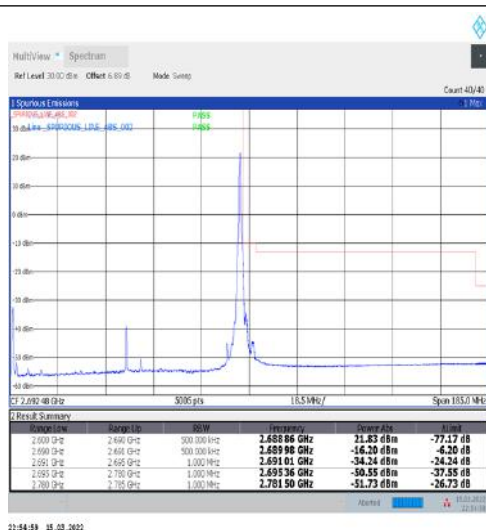
1-N41-30-90-H-2-DFT-PI2BPSK-Edge_1RB_Right-1@244-Ant1-PASS-see graph
