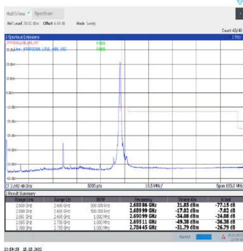
1-N41-30-90-H-5-CP-QPSK-Edge_1RB_Right-1@244-Ant1-PASS-see graph
