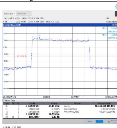
1-N41-30-100-M-5-DFT-256QAM-Outer_Full-270@0-Ant1-96.451-100.200-≤100-PASS
