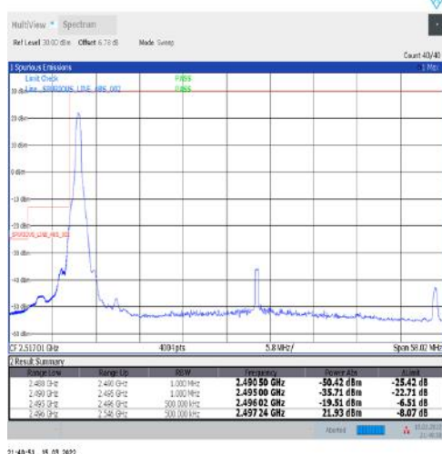
1-N41-30-50-L-4-CP-QPSK-Edge_1RB_Left-1@0-Ant1-PASS-see graph
