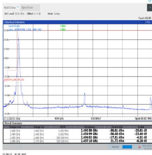
1-N41-30-80-L-4-CP-QPSK-Edge_1RB_Left-1@0-Ant1-PASS-see graph
