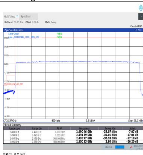
1-N41-30-90-L-3-DFT-PI2BPSK-Outer_Full-240@0-Ant1-PASS-see graph
