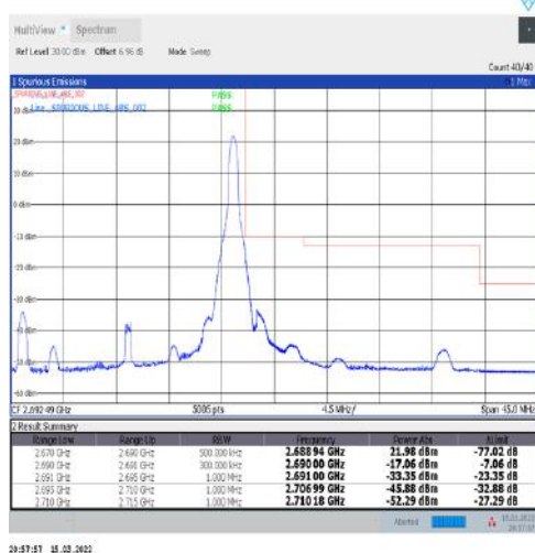
1-N41-30-20-H-5-CP-QPSK-Edge_1RB_Right-1@50-Ant1-PASS-see graph
