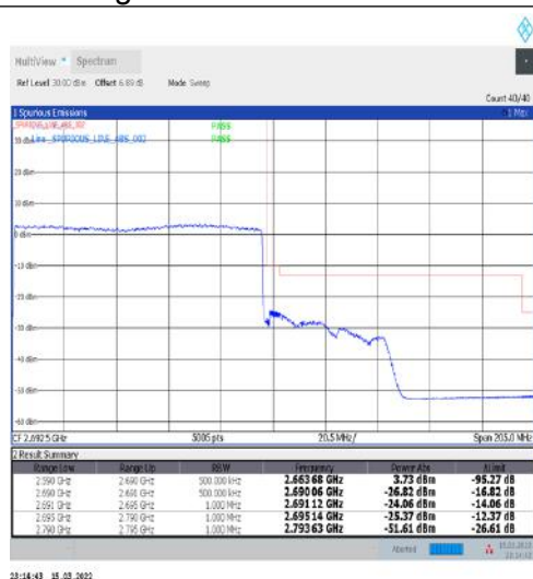
1-N41-30-100-H-3-DFT-PI2BPSK-Outer_Full-270@0-Ant1-PASS-see graph
