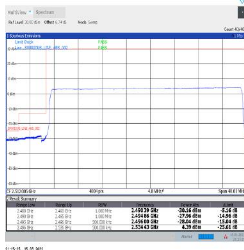
1-N41-30-40-L-6-CP-QPSK-Outer_Full-106@0-Ant1-PASS-see graph
