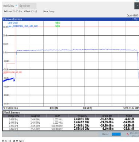
1-N41-30-80-L-3-DFT-PI2BPSK-Outer_Full-216@0-Ant1-PASS-see graph
