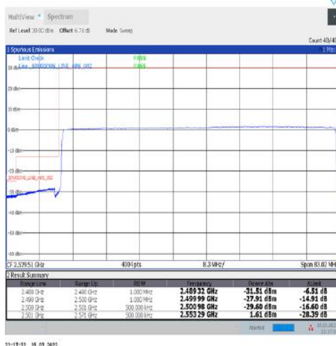
1-N41-30-70-L-6-CP-QPSK-Outer_Full-189@0-Ant1-PASS-see graph
