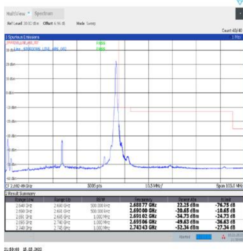
1-N41-30-50-H-5-CP-QPSK-Edge_1RB_Right-1@132-Ant1-PASS-see graph
