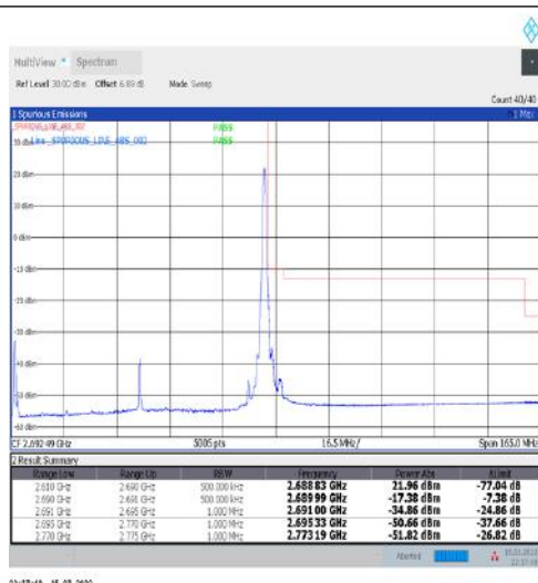
1-N41-30-80-H-2-DFT-PI2BPSK-Edge_1RB_Right-1@216-Ant1-PASS-see graph
