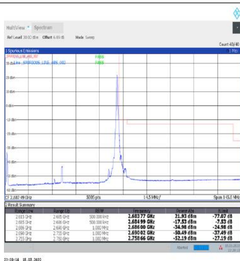
1-N41-30-70-H-2-DFT-PI2BPSK-Edge_1RB_Right-1@188-Ant1-PASS-see graph
