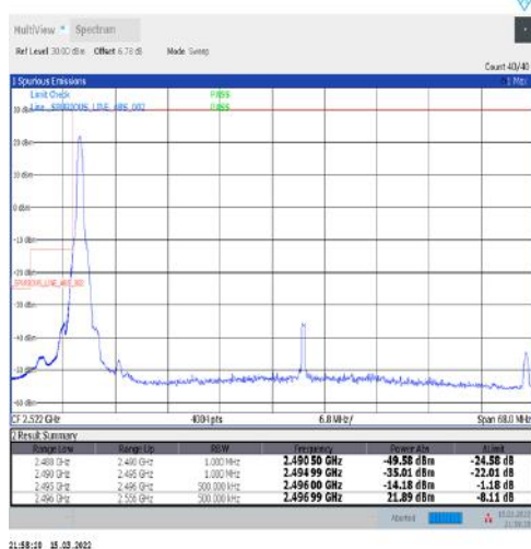
1-N41-30-60-L-4-CP-QPSK-Edge_1RB_Left-1@0-Ant1-PASS-see graph
