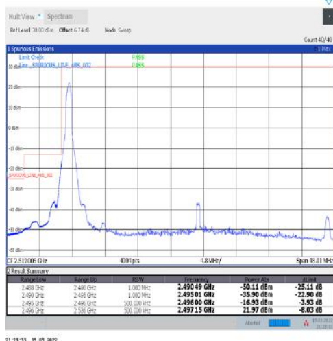
1-N41-30-40-L-4-CP-QPSK-Edge_1RB_Left-1@0-Ant1-PASS-see graph
