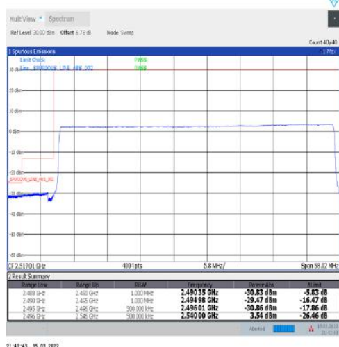
1-N41-30-50-L-6-CP-QPSK-Outer_Full-133@0-Ant1-PASS-see graph
