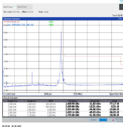
1-N41-30-100-H-5-CP-QPSK-Edge_1RB_Right-1@272-Ant1-PASS-see graph
