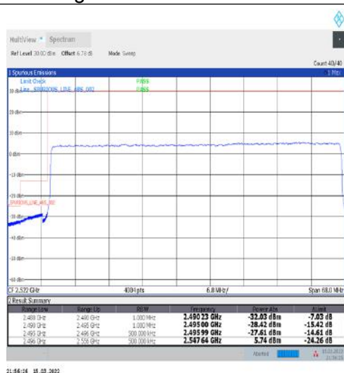
1-N41-30-60-L-3-DFT-PI2BPSK-Outer_Full-162@0-Ant1-PASS-see graph
