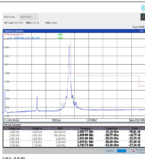
1-N41-30-50-H-2-DFT-PI2BPSK-Edge_1RB_Right-1@132-Ant1-PASS-see graph
