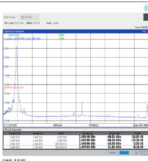
1-N41-30-90-L-1-DFT-PI2BPSK-Edge_1RB_Left-1@0-Ant1-PASS-see graph
