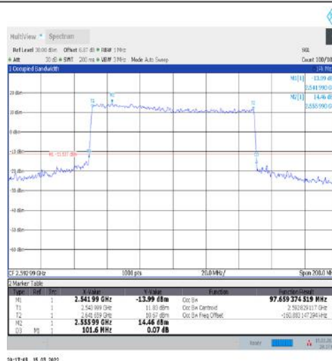
1-N41-30-100-M-7-CP-16QAM-Outer_Full-273@0-Ant1-97.659-101.600-≤100-PASS
