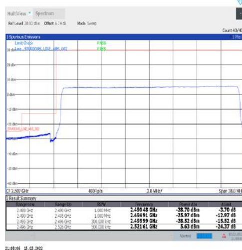
1-N41-30-30-L-6-CP-QPSK-Outer_Full-78@0-Ant1-PASS-see graph
