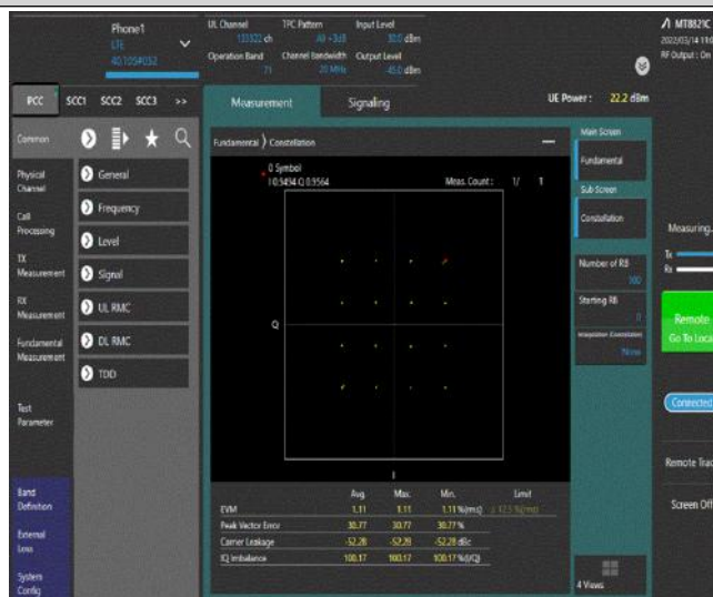
Band71-20MHz-16QAM-133322-100RB#0
