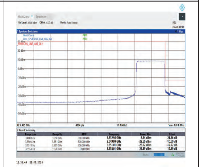
1-N78-3450-3550-PC1-30-30-H-6-CP-QPSK-Outer_Full-78@0-Ant1-1--PASS-see graph
