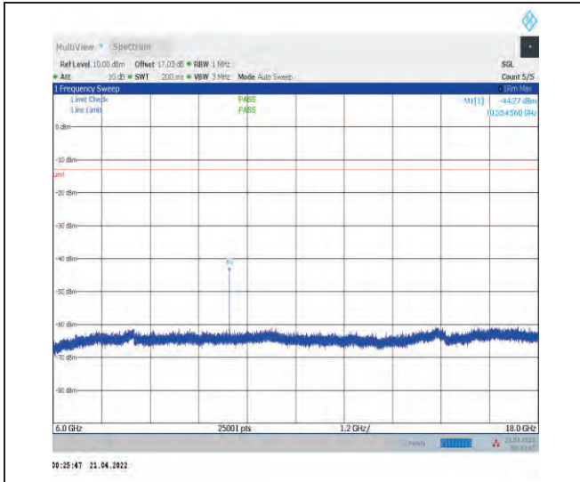
1-N78-3450-3550--30-100-H-1-DFT-PI2BPSK-Inner _1RB_Left-1@1-6000-18000-Ant1--44.27--13-PASS
