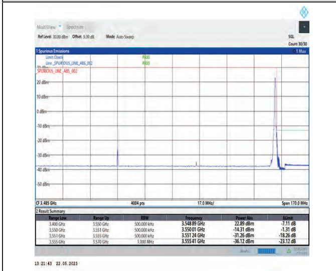
1-N78-3450-3550-PC1-30-100-H-5-CP-QPSK-Edge_1RB_Right-1@272-Ant1-1--PASS-see graph
