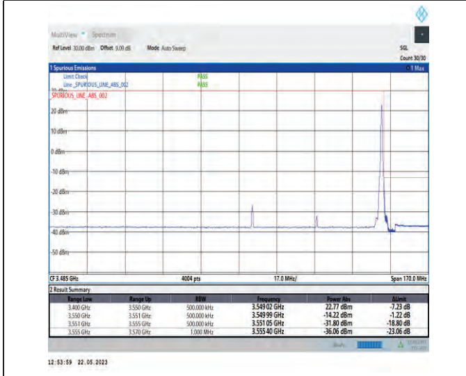
1-N78-3450-3550-PC1-30-60-H-5-CP-QPSK-Edge_1RB_Right-1@161-Ant1-1--PASS-see graph
