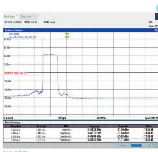
1-N78-3450-3550-PC1-30-20-L-3-DFT-PI2BPSK-Outer_Full-50@0-Ant1-1--PASS-see graph
