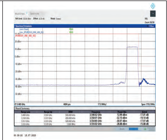
1-N78-3450-3550-PC1-30-15-H-3-DFT-PI2BPSK-Outer_Full-36@0-Ant1-1--PASS-see graph
