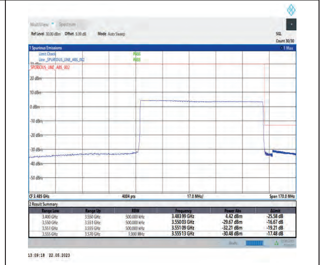
1-N78-3450-3550-PC1-30-80-H-6-CP-QPSK-Outer_Full-217@0-Ant1-1--PASS-see graph
