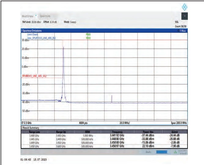
1-N78-3450-3550-PC1-30-60-L-1-DFT-PI2BPSK-Edge_1RB_Left-1@0-Ant1-1--PASS-see graph
