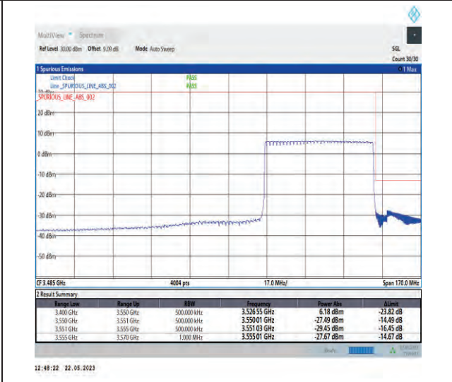
1-N78-3450-3550-PC1-30-50-H-6-CP-QPSK-Outer_Full-133@0-Ant1-1--PASS-see graph
