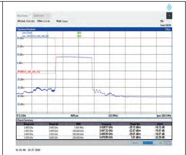
1-N78-3450-3550-PC1-30-50-L-3-DFT-PI2BPSK-Outer_Full-128@0-Ant1-1--PASS-see graph
