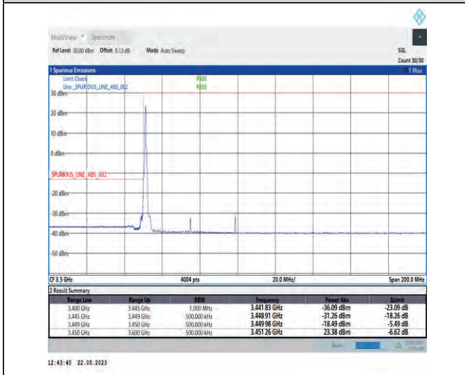
1-N78-3450-3550-PC1-30-50-L-4-CP-QPSK-Edge_1RB_Left-1@0-Ant1-1--PASS-see graph
