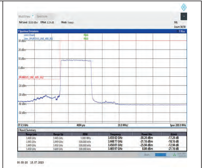
1-N78-3450-3550-PC1-30-40-L-3-DFT-PI2BPSK-Outer_Full-100@0-Ant1-1--PASS-see graph
