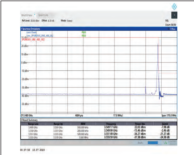
1-N78-3450-3550-PC1-30-15-H-2-DFT-PI2BPSK-Edge_1RB_Right-1@37-Ant1-1--PASS-see graph
