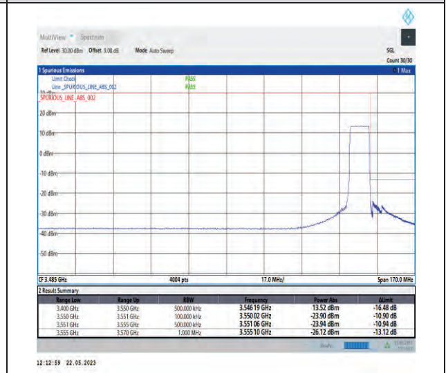
1-N78-3450-3550-PC1-30-10-H-6-CP-QPSK-Outer_Full-24@0-Ant1-1--PASS-see graph
