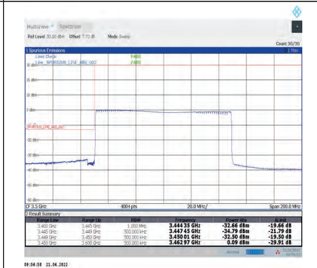
1-N78-3450-3550--30-100-L-6-CP-QPSK-Outer_F ull-273@0-Ant1-PASS-see graph
