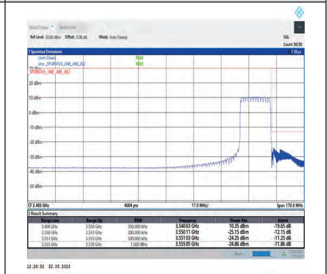
1-N78-3450-3550-PC1-30-20-H-6-CP-QPSK-Outer _Full-51@0-Ant1-1--PASS-see graph
