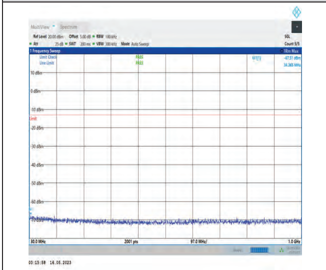
1-N78-3450-3550-PC1-30-100-H-1-DFT-PI2BPSK- Inner_1RB_Left-1@1-30-1000-Ant1-34.37--67.51--1 3-PASS
