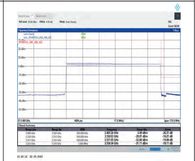
1-N78-3450-3550-PC1-30-100-H-6-CP-QPSK-Outer_Full-273@0-Ant1-1--PASS-see graph
