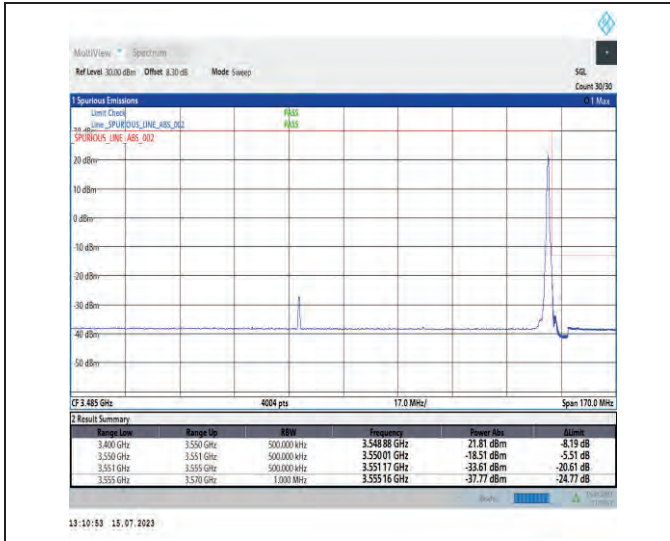
1-N78-3450-3550-PC1-30-80-H-2-DFT-PI2BPSK-Edge_1RB_Right-1@216-Ant1-1--PASS-see graph
