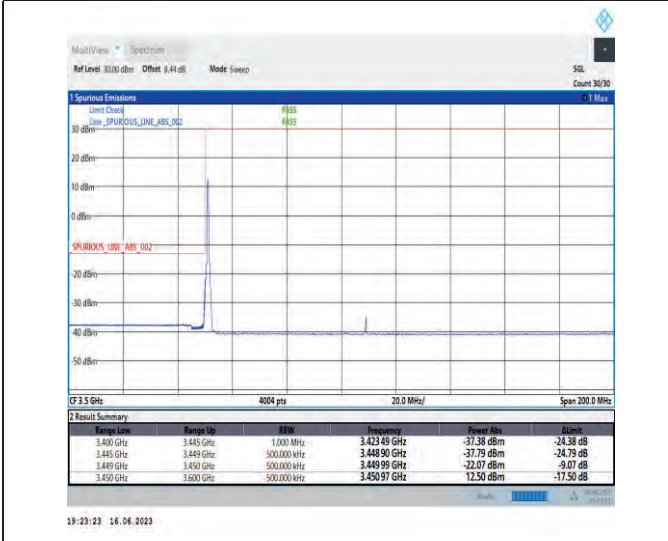
1-N78-3450-3550-PC1-30-60-L-4-CP-QPSK-Edge_1RB_Left-1@0-Ant1-1--PASS-see graph
