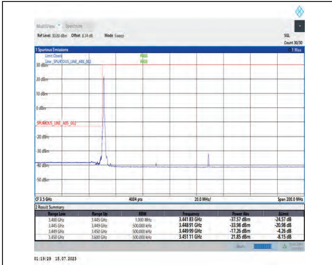
1-N78-3450-3550-PC1-30-80-L-1-DFT-PI2BPSK-Edge_1RB_Left-1@0-Ant1-1--PASS-see graph
