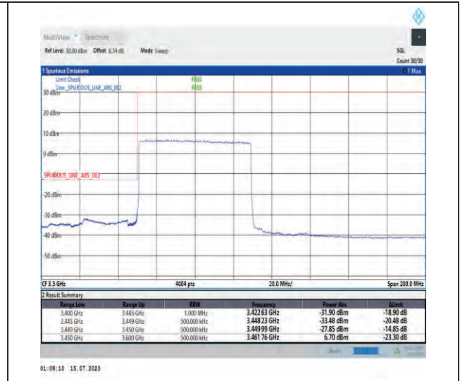
1-N78-3450-3550-PC1-30-60-L-3-DFT-PI2BPSK-Outer_Full-162@0-Ant1-1--PASS-see graph
