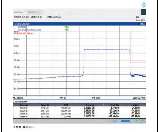
1-N78-3450-3550-PC1-30-60-H-6-CP-QPSK-Outer_Full-162@0-Ant1-1--PASS-see graph
