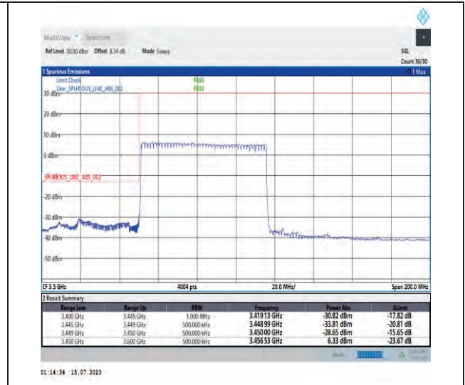
1-N78-3450-3550-PC1-30-70-L-3-DFT-PI2BPSK-Outer_Full-180@0-Ant1-1--PASS-see graph
