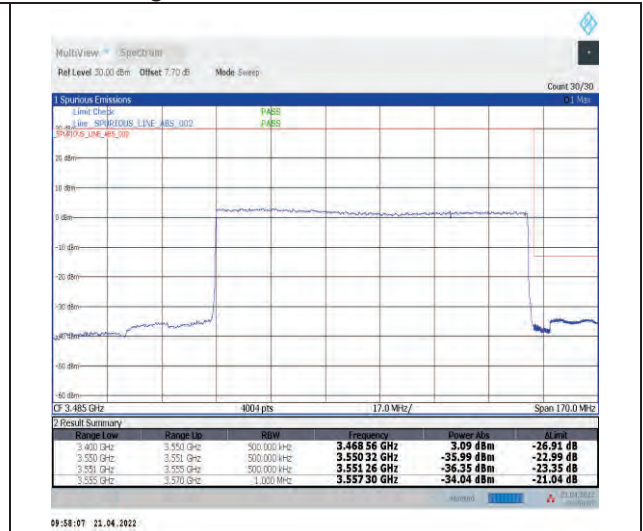
1-N78-3450-3550--30-100-H-3-DFT-PI2BPSK-Out er_Full-270@0-Ant1-PASS-see graph
