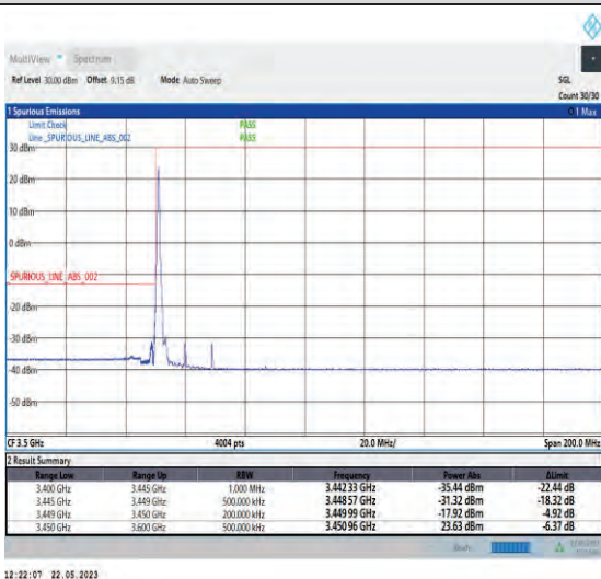
1-N78-3450-3550-PC1-30-20-L-4-CP-QPSK-Edge_1RB_Left-1@0-Ant1-1--PASS-see graph
