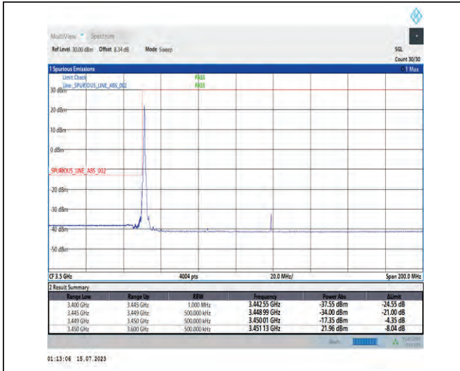
1-N78-3450-3550-PC1-30-70-L-1-DFT-PI2BPSK-Edge_1RB_Left-1@0-Ant1-1--PASS-see graph
