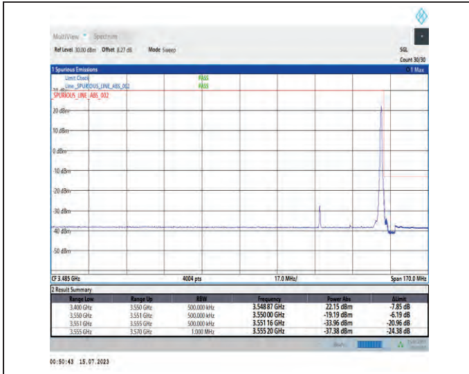
1-N78-3450-3550-PC1-30-30-H-2-DFT-PI2BPSK-Edge_1RB_Right-1@77-Ant1-1--PASS-see graph
