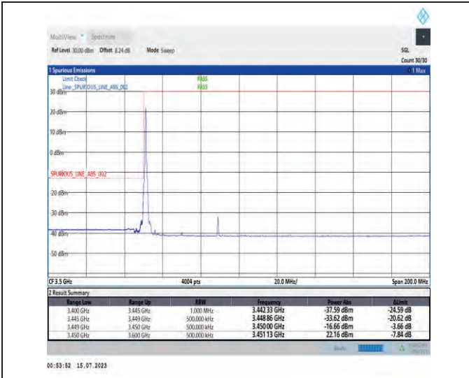
1-N78-3450-3550-PC1-30-40-L-1-DFT-PI2BPSK-Edge_1RB_Left-1@0-Ant1-1--PASS-see graph
