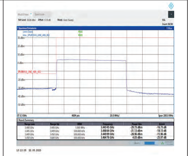
1-N78-3450-3550-PC1-30-90-L-6-CP-QPSK-Outer_Full-245@0-Ant1-1--PASS-see graph
