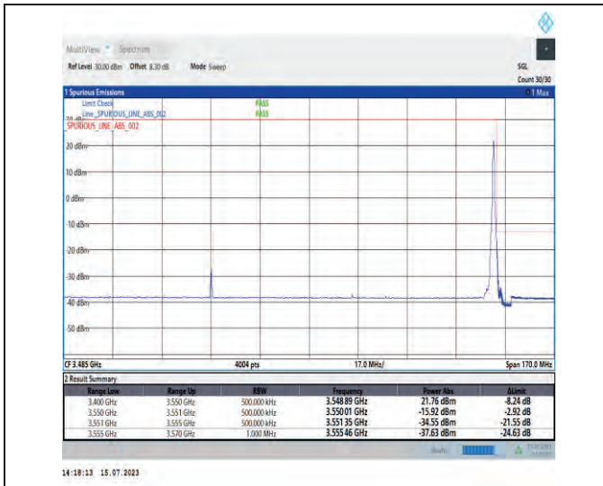
1-N78-3450-3550-PC1-30-100-H-2-DFT-PI2BPSK-Edge_1RB_Right-1@272-Ant1-1--PASS-see graph
