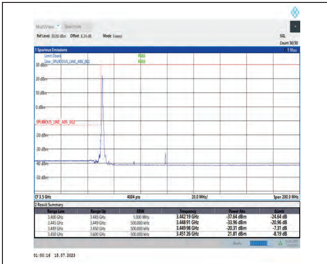
1-N78-3450-3550-PC1-30-50-L-1-DFT-PI2BPSK-Edge_1RB_Left-1@0-Ant1-1--PASS-see graph
