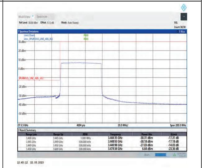
1-N78-3450-3550-PC1-30-50-L-6-CP-QPSK-Outer_Full-133@0-Ant1-1--PASS-see graph
