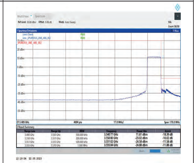
1-N78-3450-3550-PC1-30-15-H-6-CP-QPSK-Outer_Full-38@0-Ant1-1--PASS-see graph
