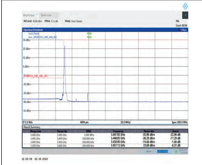
1-N78-3450-3550-PC1-30-30-L-4-CP-QPSK-Edge_1R_B_Left-1@0-Ant1-1--PASS-see graph
