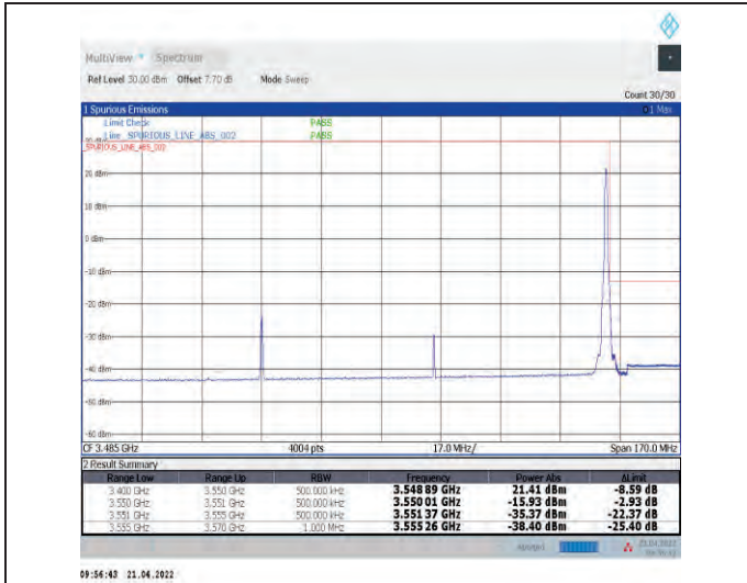
1-N78-3450-3550--30-100-H-2-DFT-PI2BPSK-Edge_1 RB_Right-1@272-Ant1-PASS-see graph
