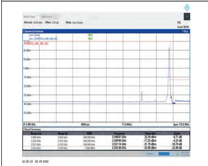
1-N78-3450-3550-PC1-30-30-H-5-CP-QPSK-Edge_1RB_Right-1@77-Ant1-1--PASS-see graph
