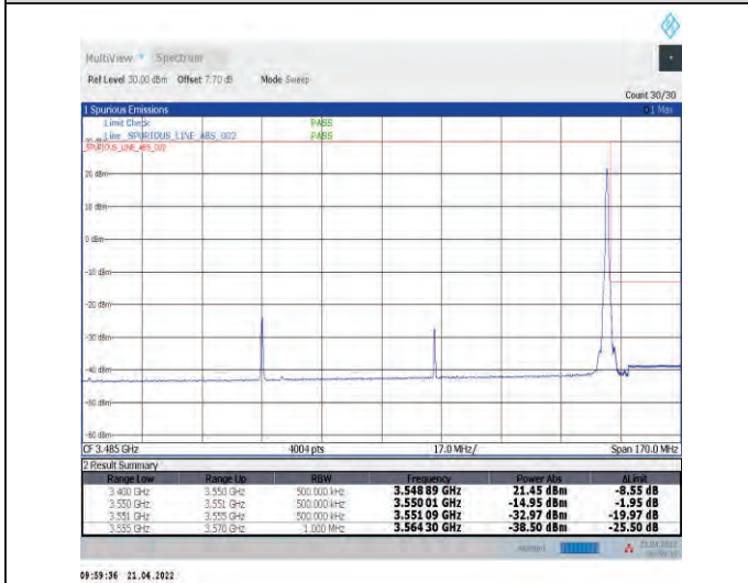
1-N78-3450-3550--30-100-H-5-CP-QPSK-Edge_1RB_Right-1@272-Ant1-PASS-see graph
