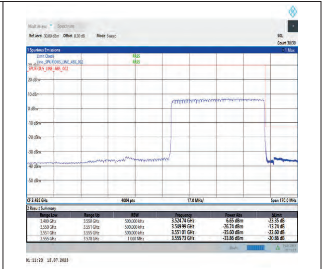
1-N78-3450-3550-PC1-30-60-H-3-DFT-PI2BPSK-Outer_Full-162@0-Ant1-1--PASS-see graph
