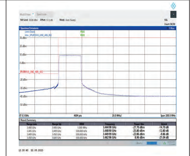
1-N78-3450-3550-PC1-30-30-L-6-CP-QPSK-Outer_Full-78@0-Ant1-1--PASS-see graph
