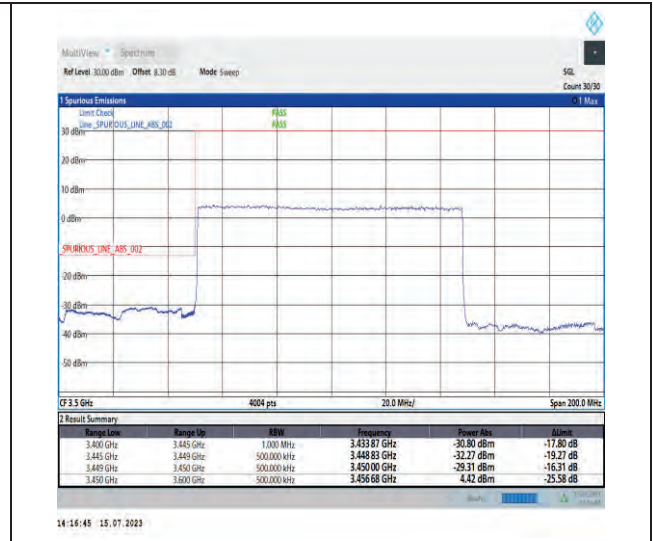
1-N78-3450-3550-PC1-30-100-L-3-DFT-PI2BPSK-Outer_Full-270@0-Ant1-1--PASS-see graph
