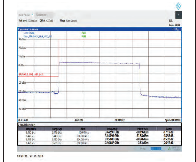
1-N78-3450-3550-PC1-30-100-L-6-CP-QPSK-Outer_Full-273@0-Ant1-1--PASS-see graph
