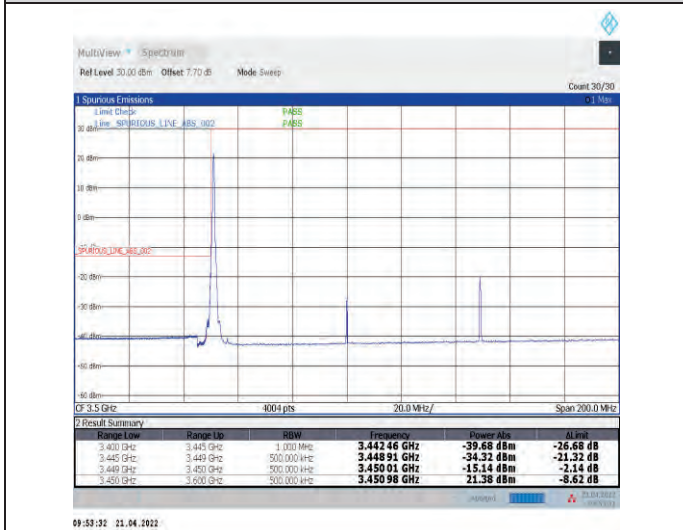
1-N78-3450-3550--30-100-L-4-CP-QPSK-Edge_1RB_Left-1@0-Ant1-PASS-see graph
