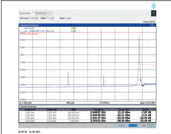
1-N78-3450-3550--30-90-H-5-CP-QPSK-Edge_1RB_R ight-1@244-Ant1-PASS-see graph
