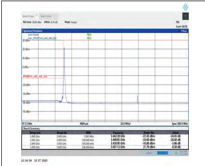
1-N78-3450-3550-PC1-30-90-L-1-DFT-PI2BPSK-Edge_1RB_Left-1@0-Ant1-1--PASS-see graph
