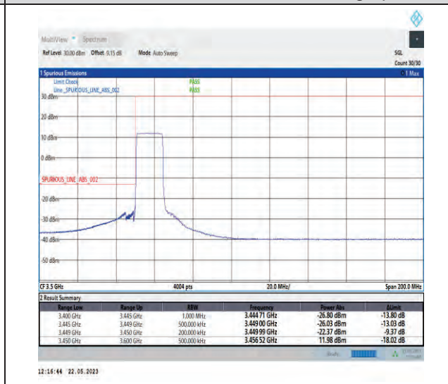
1-N78-3450-3550-PC1-30-15-L-6-CP-QPSK-Outer_Full-38@0-Ant1-1--PASS-see graph
