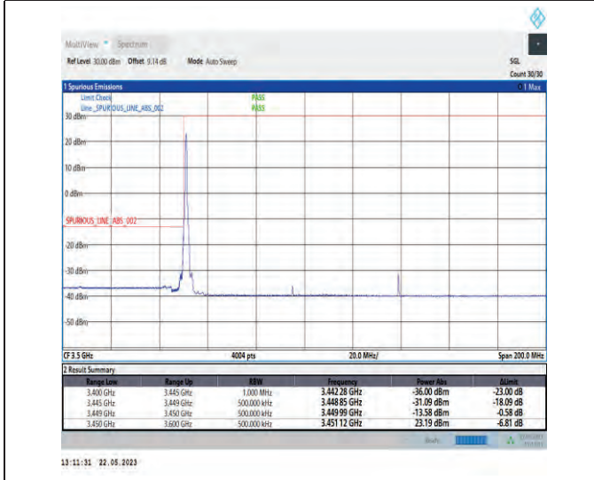
1-N78-3450-3550-PC1-30-90-L-4-CP-QPSK-Edge_1RB_Left-1@0-Ant1-1--PASS-see graph
