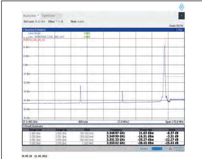
1-N78-3450-3550--30-90-H-2-DFT-PI2BPSK-Edge_1R_B_Right-1@244-Ant1-PASS-see graph
