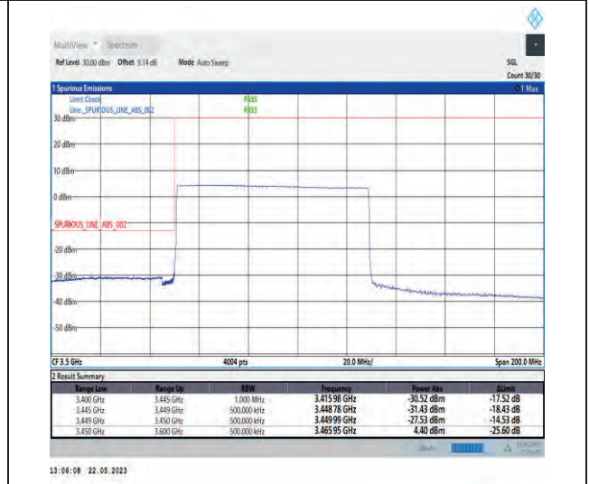
1-N78-3450-3550-PC1-30-80-L-6-CP-QPSK-Outer_Full-217@0-Ant1-1--PASS-see graph
