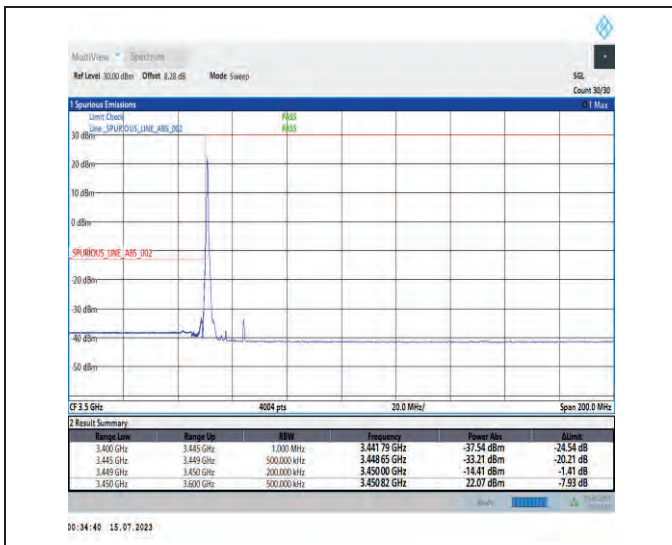
1-N78-3450-3550-PC1-30-15-L-1-DFT-PI2BPSK-Edge_e_1RB_Left-1@0-Ant1-1--PASS-see graph
