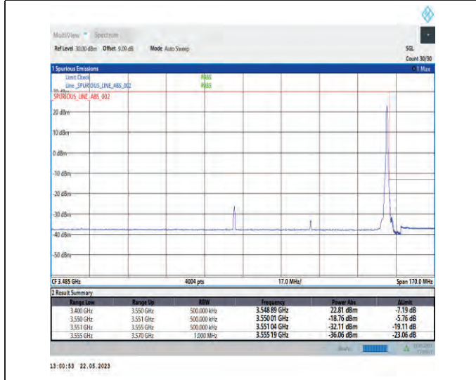
1-N78-3450-3550-PC1-30-70-H-5-CP-QPSK-Edge_1RB_Right-1@188-Ant1-1--PASS-see graph
