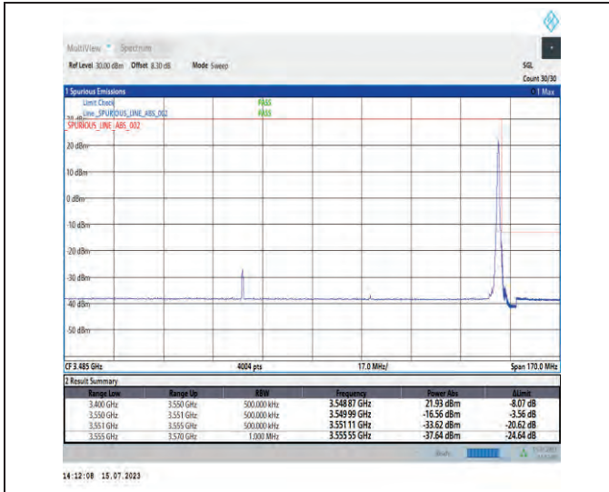
1-N78-3450-3550-PC1-30-90-H-2-DFT-PI2BPSK-Edge_1RB_Right-1@244-Ant1-1--PASS-see graph
