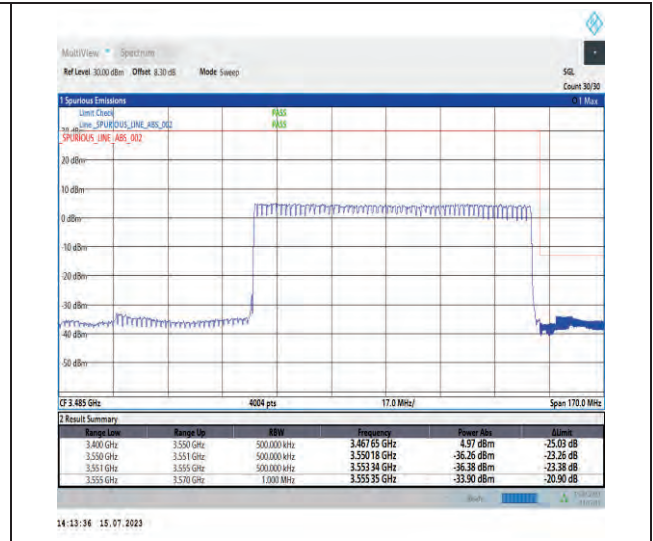
1-N78-3450-3550-PC1-30-90-H-3-DFT-PI2BPSK-Outer_Full-240@0-Ant1-1--PASS-see graph
