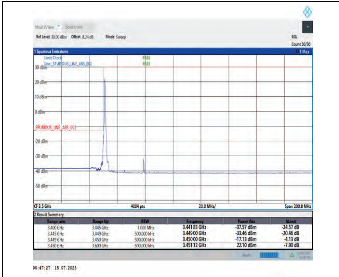
1-N78-3450-3550-PC1-30-30-L-1-DFT-PI2BPSK-Edge_e_1RB_Left-1@0-Ant1-1--PASS-see graph
