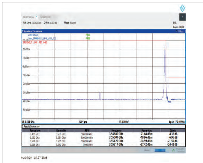
1-N78-3450-3550-PC1-30-70-H-2-DFT-PI2BPSK-Edge_1RB_Right-1@188-Ant1-1--PASS-see graph
