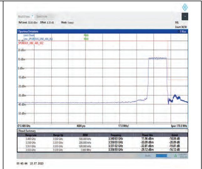
1-N78-3450-3550-PC1-30-20-H-3-DFT-PI2BPSK- Outer_Full-50@0-Ant1-1--PASS-see graph
