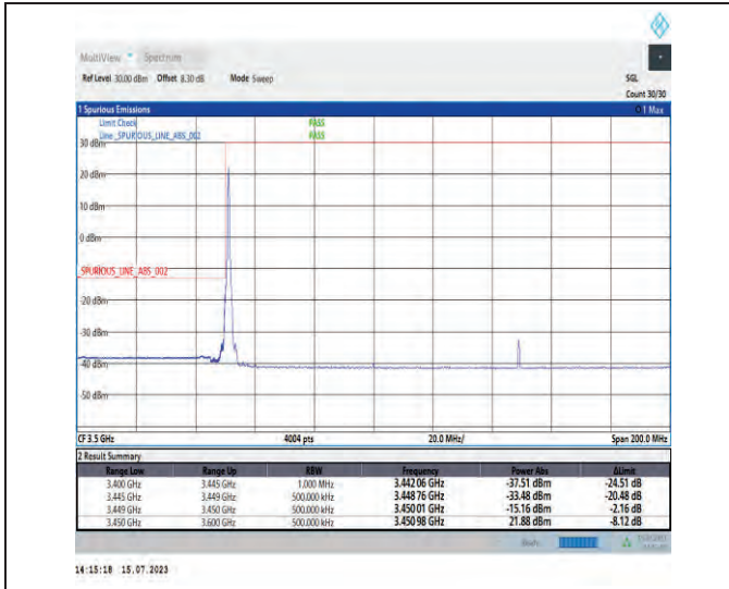
1-N78-3450-3550-PC1-30-100-L-1-DFT-PI2BPSK-Edge_e_1RB_Left-1@0-Ant1-1--PASS-see graph
