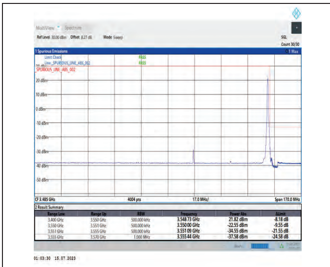
1-N78-3450-3550-PC1-30-50-H-2-DFT-PI2BPSK-Edge_1RB_Right-1@132-Ant1-1--PASS-see graph
