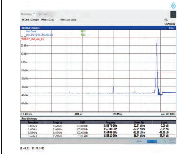
1-N78-3450-3550-PC1-30-50-H-5-CP-QPSK-Edge_1RB_Right-1@132-Ant1-1--PASS-see graph
