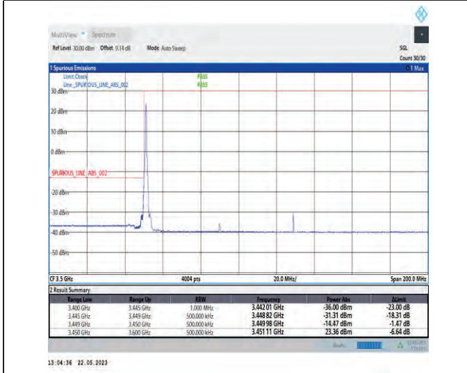
1-N78-3450-3550-PC1-30-80-L-4-CP-QPSK-Edge_1RB_Left-1@0-Ant1-1--PASS-see graph
