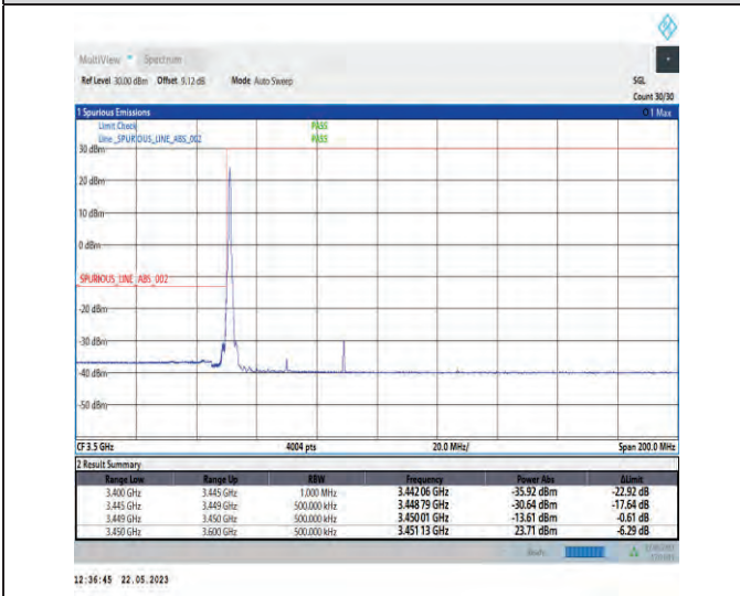
1-N78-3450-3550-PC1-30-40-L-4-CP-QPSK-Edge_1RB_Left-1@0-Ant1-1--PASS-see graph
