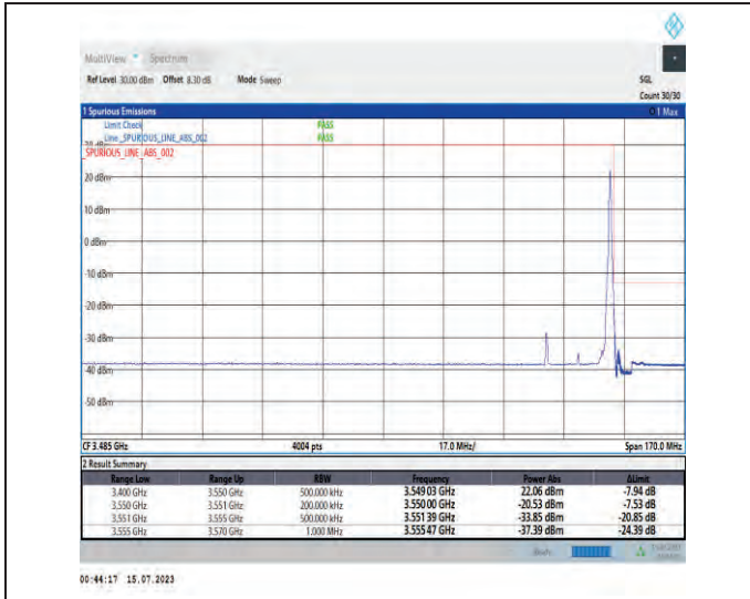
1-N78-3450-3550-PC1-30-20-H-2-DFT-PI2BPSK-Edge _1RB_Right-1@50-Ant1-1--PASS-see graph
