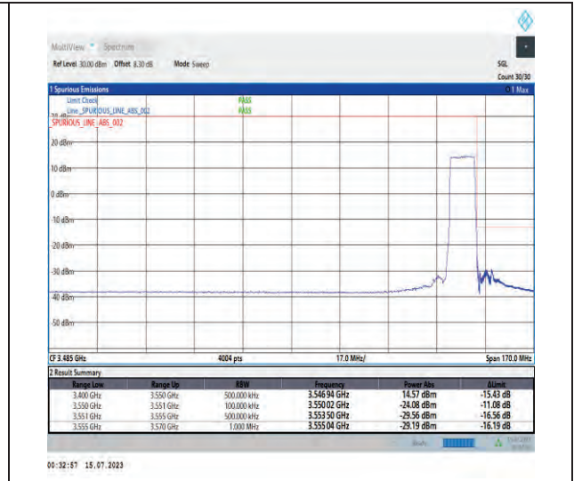
1-N78-3450-3550-PC1-30-10-H-3-DFT-PI2BPSK-Outer_Full-24@0-Ant1-1--PASS-see graph
