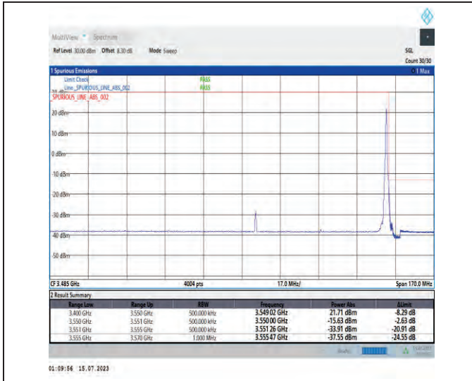
1-N78-3450-3550-PC1-30-60-H-2-DFT-PI2BPSK-Edge_1RB_Right-1@161-Ant1-1--PASS-see graph
