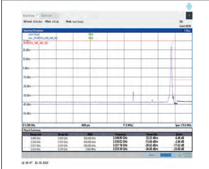
1-N78-3450-3550-PC1-30-40-H-5-CP-QPSK-Edge_1RB_Right-1@105-Ant1-1--PASS-see graph
