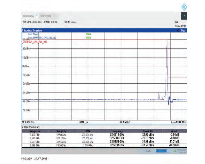
1-N78-3450-3550-PC1-30-10-H-2-DFT-PI2BPSK-Edge_1RB_Right-1@23-Ant1-1--PASS-see graph
