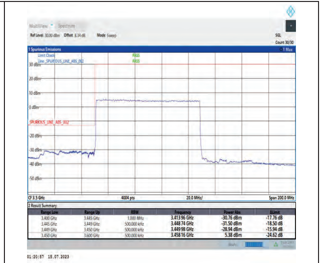
1-N78-3450-3550-PC1-30-80-L-3-DFT-PI2BPSK-Outer_Full-216@0-Ant1-1--PASS-see graph
