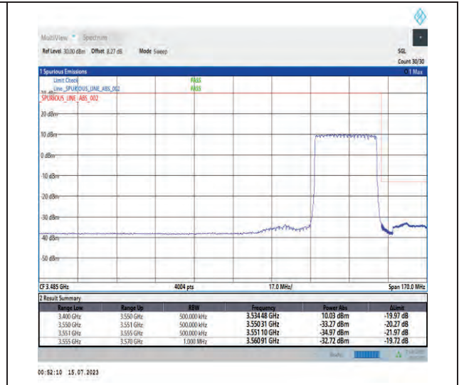
1-N78-3450-3550-PC1-30-30-H-3-DFT-PI2BPSK-Outer_Full-75@0-Ant1-1--PASS-see graph
