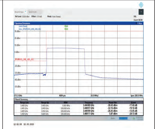
1-N78-3450-3550-PC1-30-60-L-6-CP-QPSK-Outer_Full-162@0-Ant1-1--PASS-see graph
