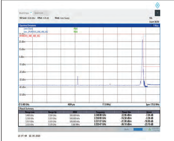
1-N78-3450-3550-PC1-30-80-H-5-CP-QPSK-Edge_1RB_Right-1@216-Ant1-1--PASS-see graph
