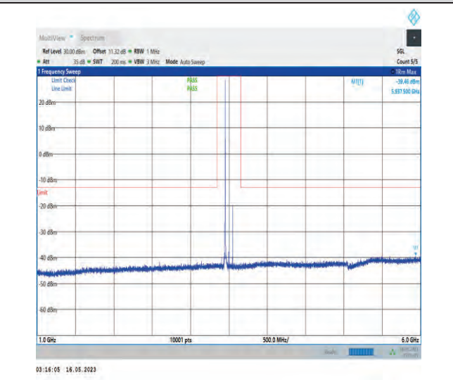
1-N78-3450-3550-PC1-30-100-H-1-DFT-PI2BPSK- Inner_1RB_Left-1@1-1000-6000-Ant1-5937.50--39.46- -13-PASS
