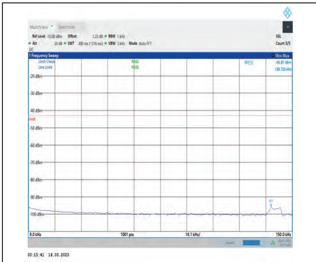
1-N78-3450-3550-PC1-30-100-H-1-DFT-PI2BPSK- Inner_1RB_Left-1@1-0.009-0.15-Ant1-0.14--95.87-- 43-PASS
