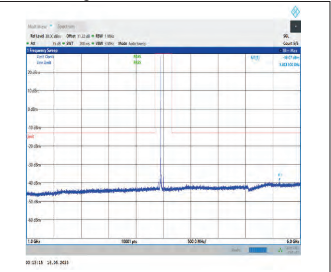
1-N78-3450-3550-PC1-30-100-M-1-DFT-PI2BPSK-In ner_1RB_Left-1@1-1000-6000-Ant1-5623.50--39.07- -13-PASS
