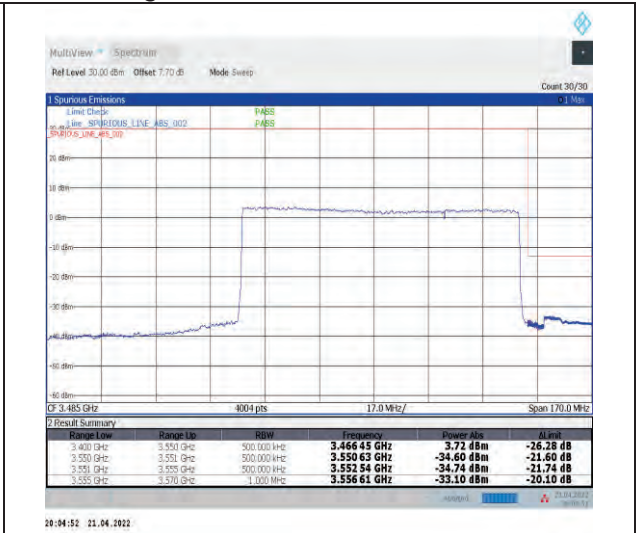
1-N78-3450-3550--30-90-H-3-DFT-PI2BPSK-Outer_Full-240@0-Ant1-PASS-see graph
