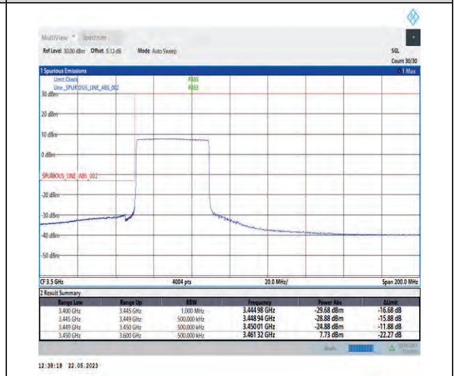
1-N78-3450-3550-PC1-30-40-L-6-CP-QPSK-Outer_Full-106@0-Ant1-1--PASS-see graph
