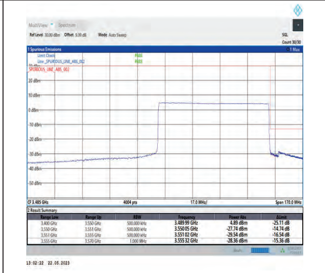
1-N78-3450-3550-PC1-30-70-H-6-CP-QPSK-Outer_Full-189@0-Ant1-1--PASS-see graph
