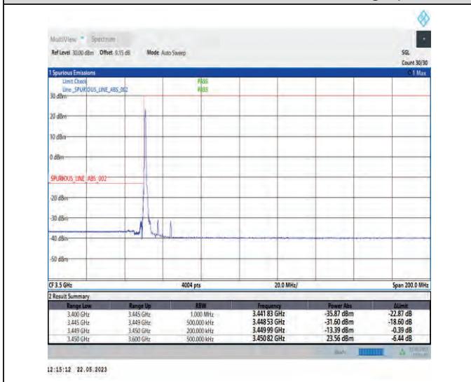
1-N78-3450-3550-PC1-30-15-L-4-CP-QPSK-Edge_1RB_Left-1@0-Ant1-1--PASS-see graph
