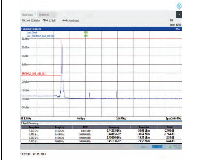
1-N78-3450-3550-PC1-30-70-L-4-CP-QPSK-Edge_1RB_Left-1@0-Ant1-1--PASS-see graph
