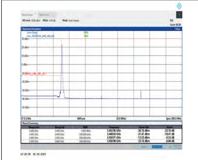
1-N78-3450-3550-PC1-30-100-L-4-CP-QPSK-Edge_1RB_Left-1@0-Ant1-1--PASS-see graph
