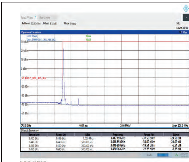
1-N78-3450-3550-PC1-30-20-L-1-DFT-PI2BPSK-Edge_e_1RB_Left-1@0-Ant1-1--PASS-see graph
