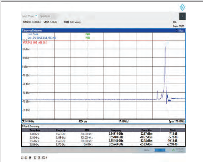
1-N78-3450-3550-PC1-30-10-H-5-CP-QPSK-Edge_1RB_Right-1@23-Ant1-1--PASS-see graph
