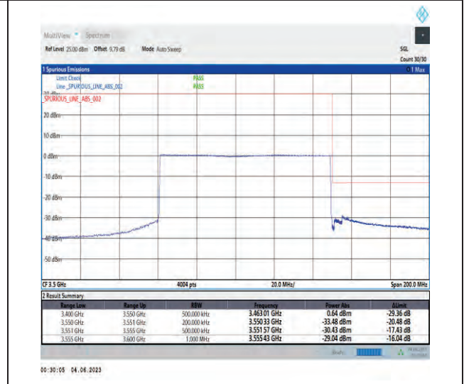
1-N78-3450-3550-PC1-30-90-H-6-CP-QPSK-Outer_Full-245@0-Ant1-1--PASS-see graph
