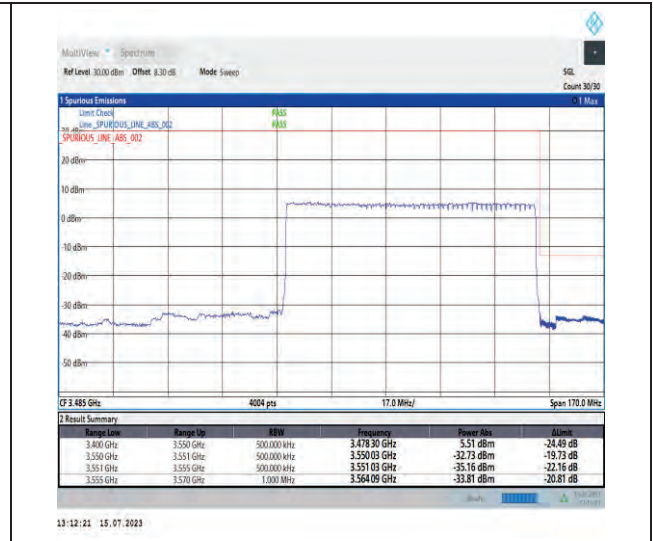
1-N78-3450-3550-PC1-30-80-H-3-DFT-PI2BPSK-Outer_Full-216@0-Ant1-1--PASS-see graph
