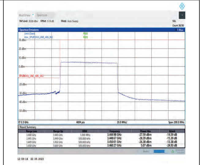
1-N78-3450-3550-PC1-30-70-L-6-CP-QPSK-Outer_Full-189@0-Ant1-1--PASS-see graph
