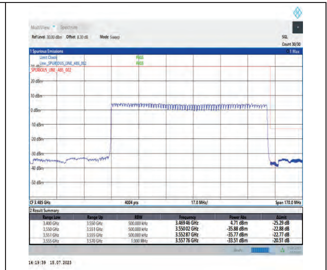
1-N78-3450-3550-PC1-30-100-H-3-DFT-PI2BPSK-Outer_Full-270@0-Ant1-1--PASS-see graph
