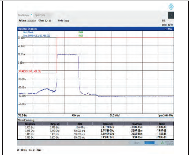
1-N78-3450-3550-PC1-30-30-L-3-DFT-PI2BPSK-Outer_Full-75@0-Ant1-1--PASS-see graph
