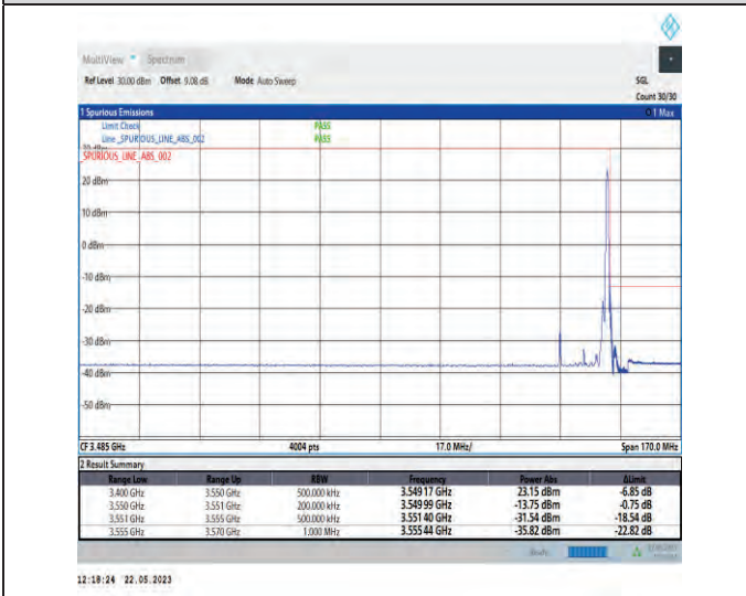
1-N78-3450-3550-PC1-30-15-H-5-CP-QPSK-Edge_1RB_Right-1@37-Ant1-1--PASS-see graph
