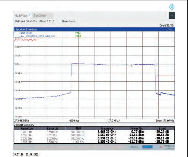
1-N78-3450-3550--30-90-H-6-CP-QPSK-Outer_Fu ll-245@0-Ant1-PASS-see graph
