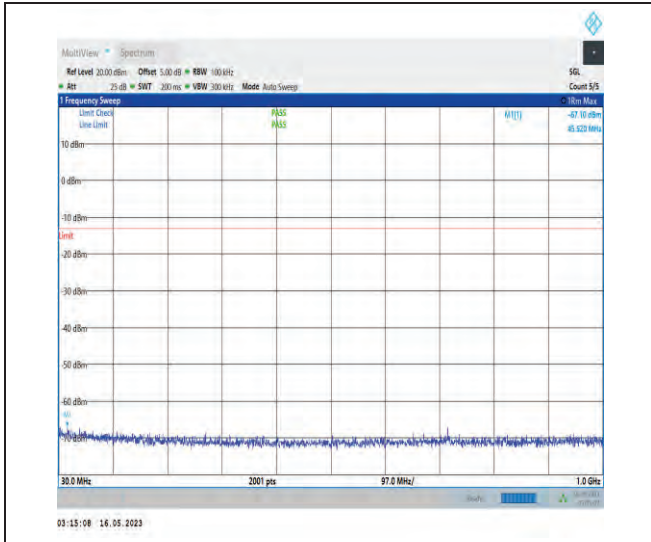
1-N78-3450-3550-PC1-30-100-M-1-DFT-PI2BPSK- nner_1RB_Left-1@1-30-1000-Ant1-45.52--67.10--1 3-PASS
