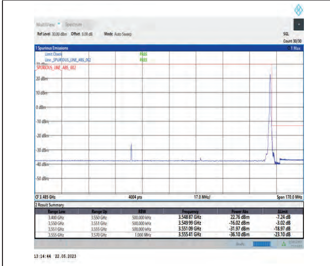
1-N78-3450-3550-PC1-30-90-H-5-CP-QPSK-Edge_1RB_Right-1@244-Ant1-1--PASS-see graph
