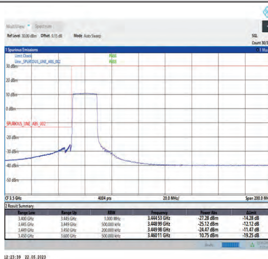
1-N78-3450-3550-PC1-30-20-L-6-CP-QPSK-Outer_Full-51@0-Ant1-1--PASS-see graph
