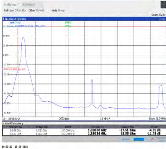
1-N2--15-10-L-1-DFT-PI2BPSK-Edge_1RB_Left-1@0-Ant1-seegraph-PASS-see graph
