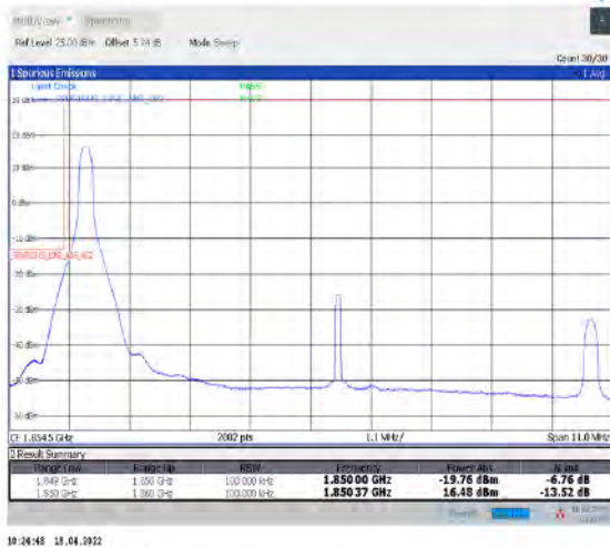
1-N2--15-10-L-4-CP-QPSK-Edge_1RB_Left-1@0-Ant1-seegraph-PASS-see graph
