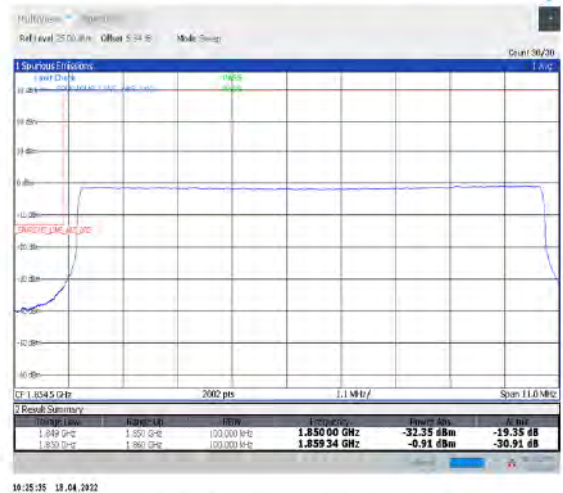
1-N2--15-10-L-6-CP-QPSK-Outer_Full-52@0-Ant1-seegraph-PASS-see graph
