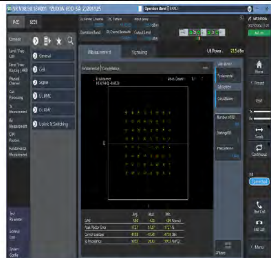
1-N2-PC3-15-20-M-8-CP-64QAM-Outer_Full-106@0-Ant1-see graph-PASS
