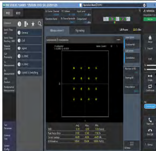
1-N2-PC3-15-20-M-7-CP-16QAM-Outer_Full-106@0-Ant1-see graph-PASS
