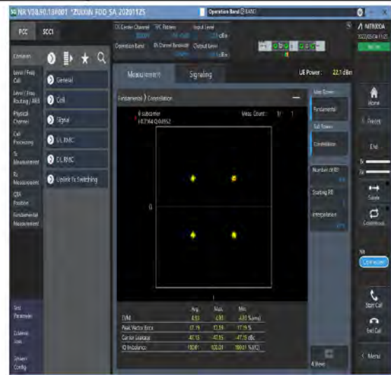
1-N2-PC3-15-20-M-6-CP-QPSK-Outer_Full-106@0-Ant1-see graph-PASS
