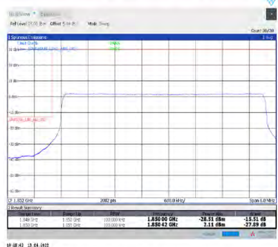
1-N2--15-5-L-6-CP-QPSK-Outer_Full-25@0-Ant1-seegraph-PASS-see graph
