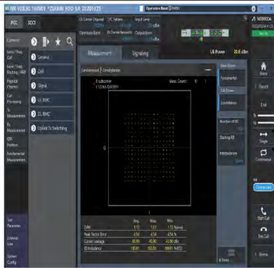
1-N2-PC3-15-20-M-5-DFT-256QAM-Outer_Full-100@0-Ant1-see graph-PASS
