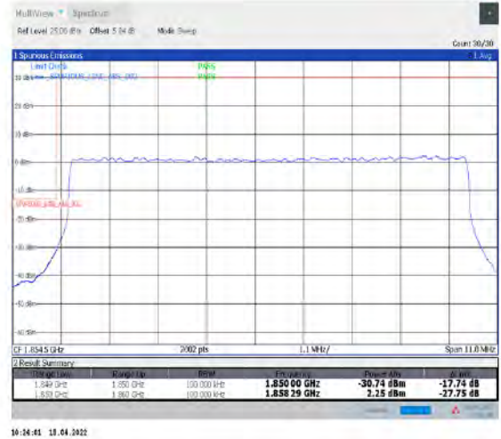
1-N2--15-10-L-3-DFT-PI2BPSK-Outer_Full-50@0-Ant1-seegraph-PASS-see graph
