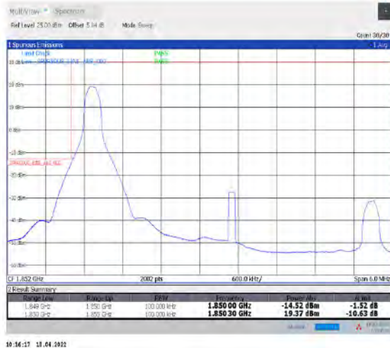
1-N2--15-5-L-1-DFT-PI2BPSK-Edge_1RB_Left-1@0-Ant1-seegraph-PASS-see graph
