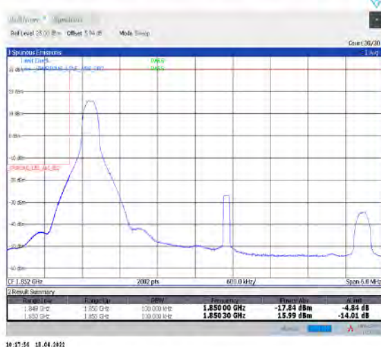
1-N2--15-5-L-4-CP-QPSK-Edge_1RB_Left-1@0-Ant1-seegraph-PASS-see graph
