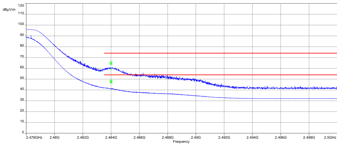
Plot 5: Upper restricted band, 2478 MHz, 2 Msps
