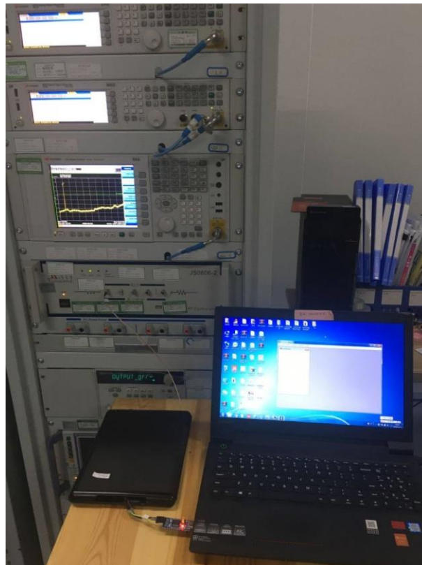
Fig. 4 Conducted emission setup photo
