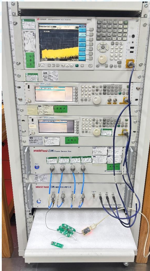
Photo of Setup for RF Conducted (BT)
