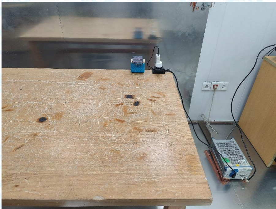
Photo of Setup for Radiated Emission (9KHz-30MHz) (Wireless charging mode)
