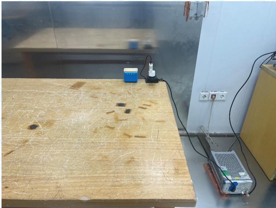
Photo of Setup for Conducted Emission (BT)
