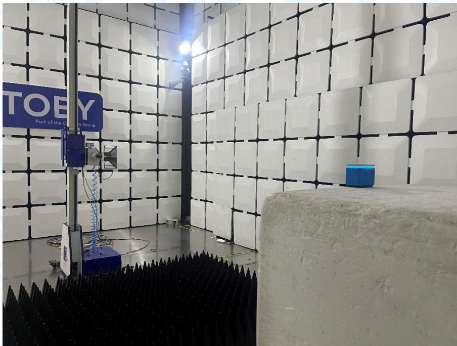
Photo of Setup for Radiated Emission (Above 1 GHz) (BT)
