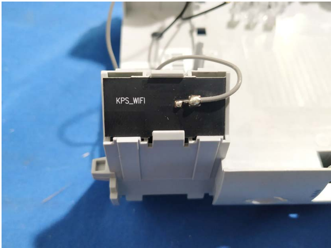
2.4G Antenna 0
