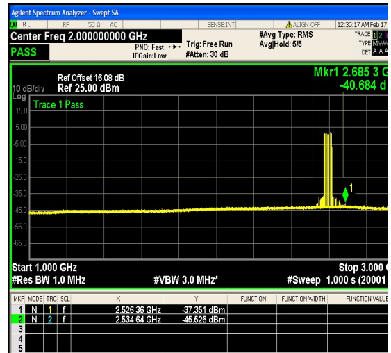
1-N41-PC2-30-50-M-15-DFT-256QAM-Outer _Full-128@0-1000-3000-Ant1--40.68--25-PA SS
