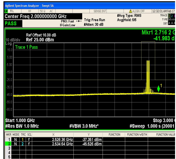
1-N41-PC2-30-50-M-12-DFT-64QAM-Outer_ Full-128@0-1000-3000-Ant1--41.98--25-PAS S
