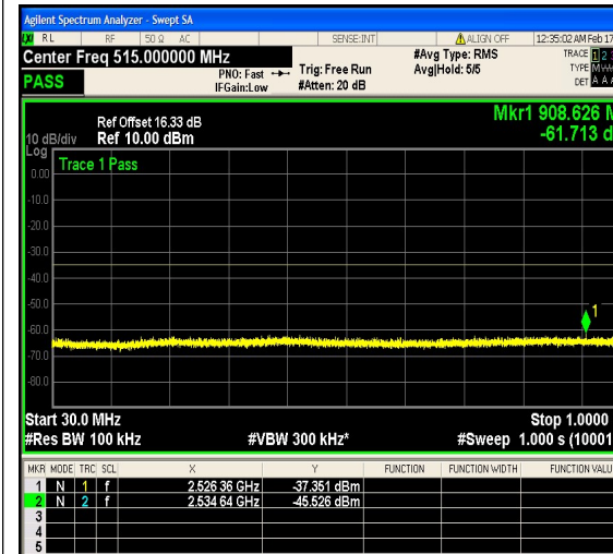
1-N41-PC2-30-50-M-15-DFT-256QAM-Outer _Full-128@0-30-1000-Ant1--61.71--35-PASS
