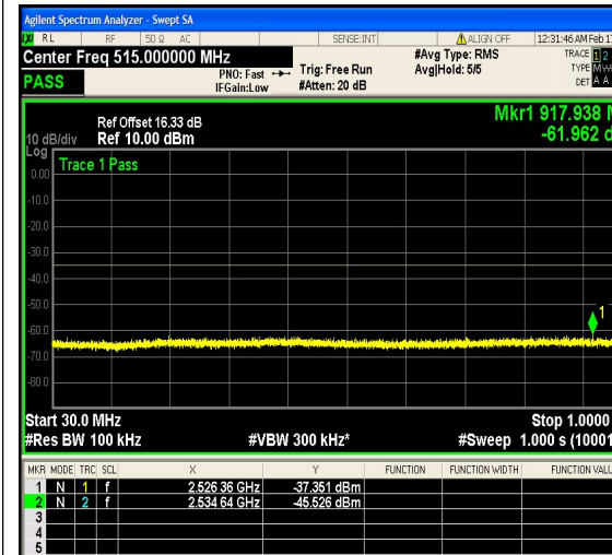
1-N41-PC2-30-50-M-12-DFT-64QAM-Outer_ Full-128@0-30-1000-Ant1--61.96--35-PASS
