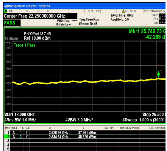
1-N41-PC2-30-50-M-8-DFT-16QAM-Edge_1 RB_Right-1@132-18000-26500-Ant1--42.29-- 25-PASS
