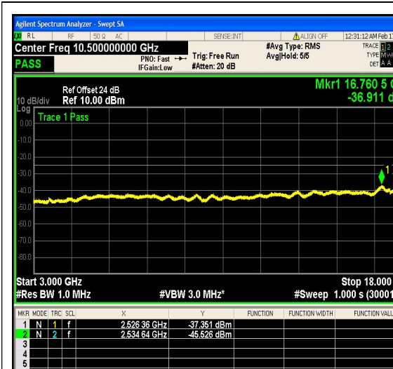
1-N41-PC2-30-50-M-11-DFT-64QAM-Edge_1 RB_Right-1@132-3000-18000-Ant1--36.91-- 25-PASS
