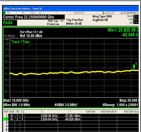
1-N41-PC2-30-50-M-13-DFT-256QAM-Edge _1RB_Left-1@0-18000-26500-Ant1--42.55--2 5-PASS
