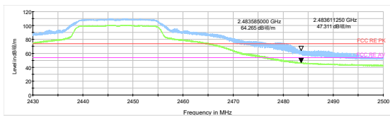
802.11g-Channel 8 Peak+ Average
