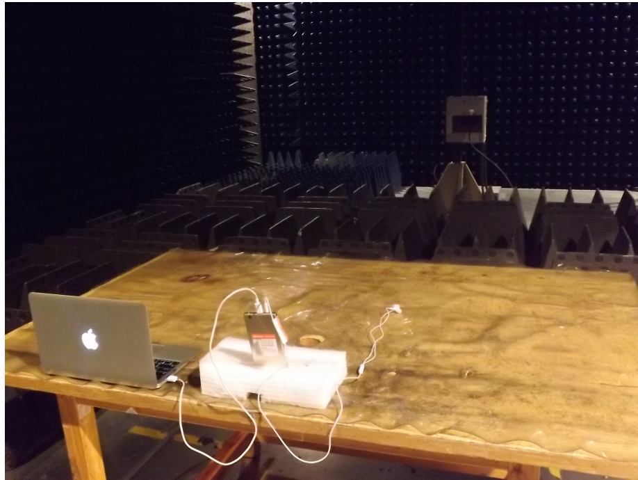
Photograph – Radiated Emission Test Setup for Above 1GHz at Test Site 1#
