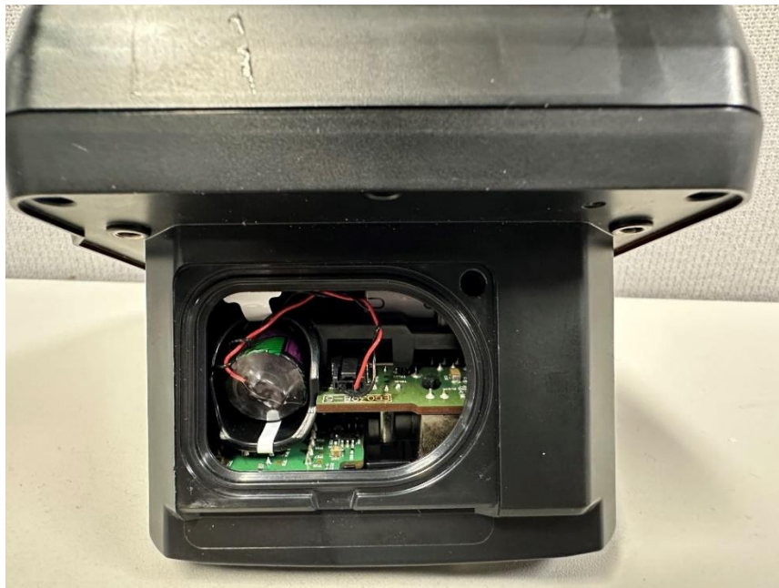
Figure 12 G6-500 OPT/IPT Assembled unit viewed from the rear side (cover removed)
