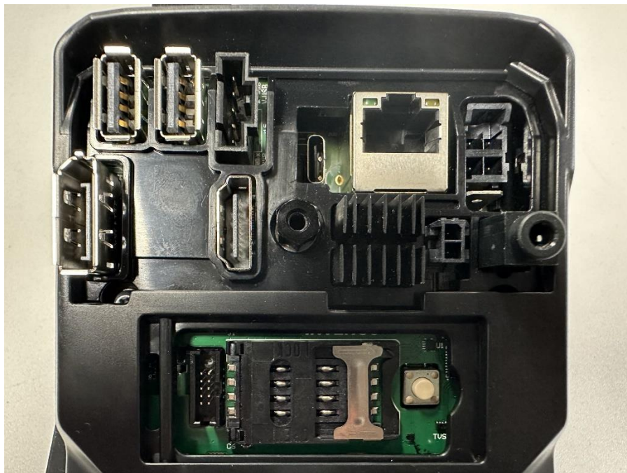
Figure 14 G6-500 OPT/IPT Assembled unit close-up viewed from the back side
