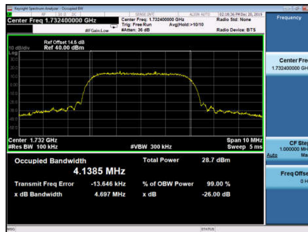
(Plot G2: WCDMA 1700 MHz Channel = 1412 bandwidth)
