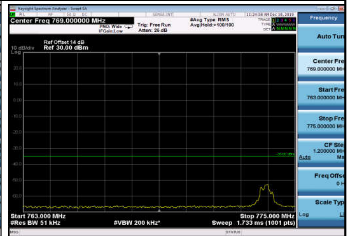
HighRange_FDD13_5MHz_784.5_fullRB _High_Q16
