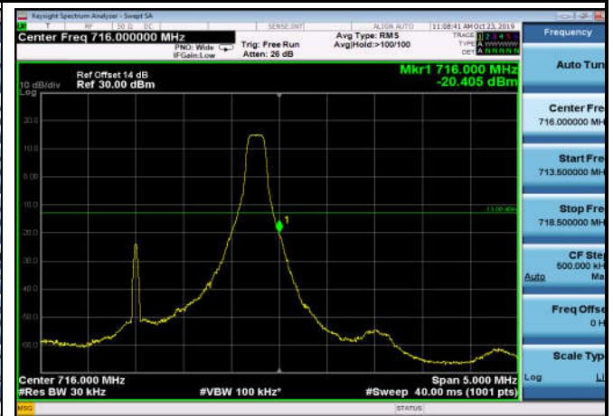
HighRange_FDD12_3MHz_714.5_OneRB _high_Q16
