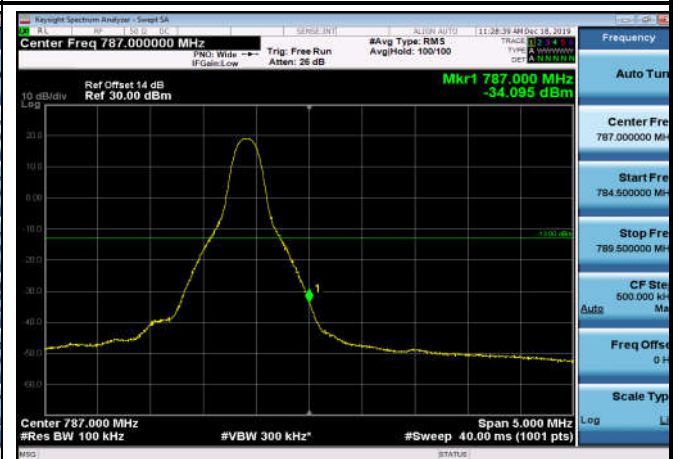
HighRange_FDD13_10MHz_782_OneRB _high_Q16
