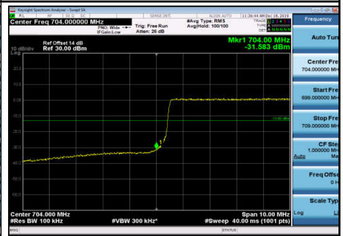
LowRange_FDD17_10MHz_709_fullIRB _Low_Q16
