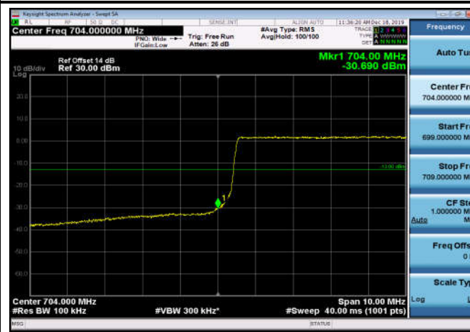
LowRange_FDD17_10MHz_709_fullIRB _Low_QPSK
