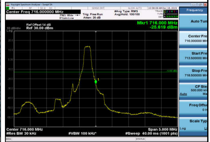
HighRange_FDD12_1.4MHz_715.3_fullIRB _High_Q16
