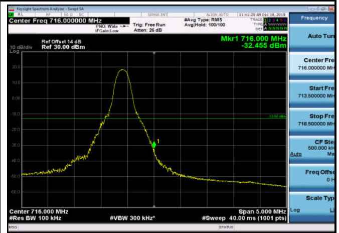
HighRange_FDD17_10MHz_711_OneRB _high_Q16
