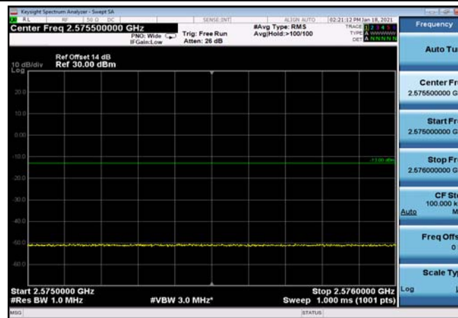
HighRange_FDD07_5MHz_2567.5_OneRB _high_QPSK
