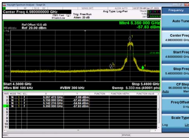
U-NII-2a ,Plot 1,Band Edge-802.11a(40 MHz),5270MHz,Ant1
