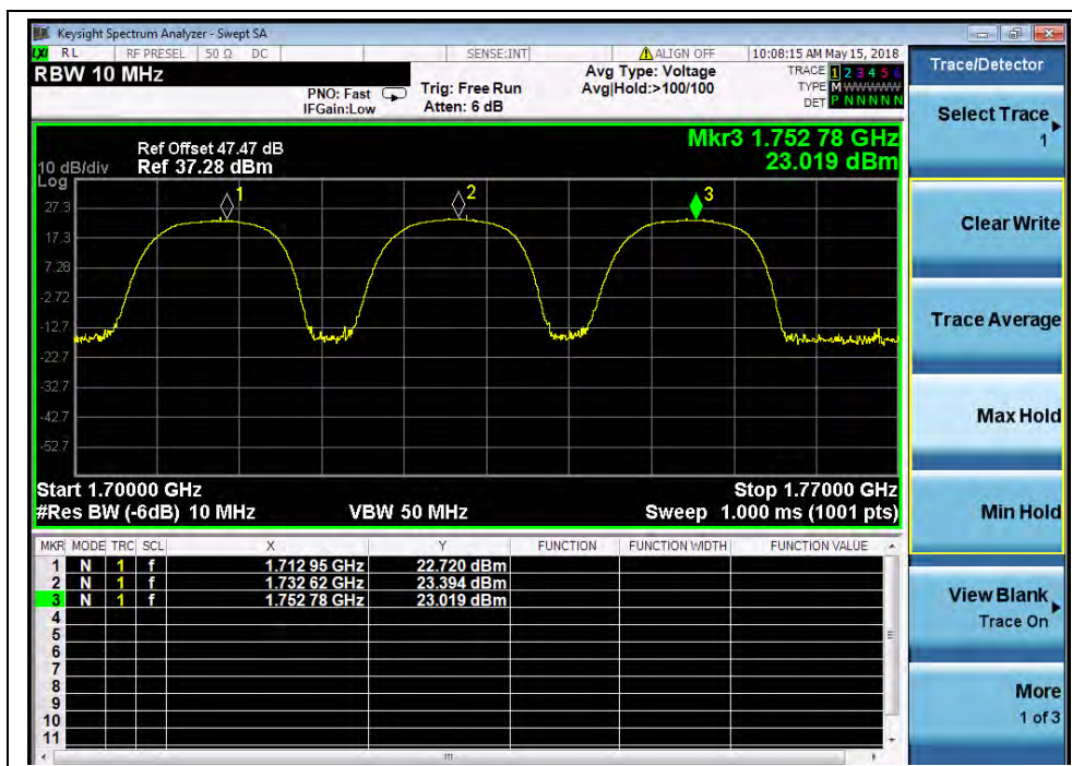
(Plot R, HSPA+1700 MHz, Channel = 1312, 1412, 1513)
