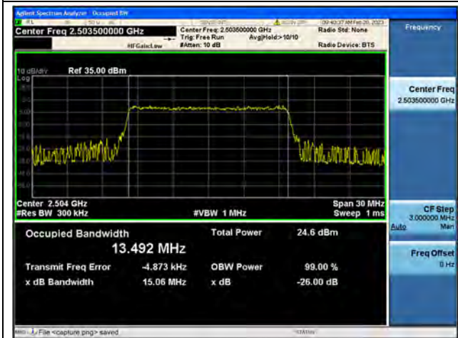
Band41 / 15MHz / 64QAM/ Low CH
