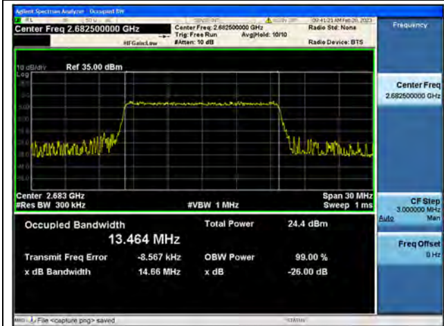
Band41 / 15MHz / 64QAM/ High CH
