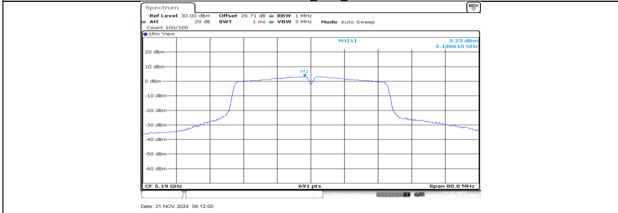
11N40SISO Ant3 5190
