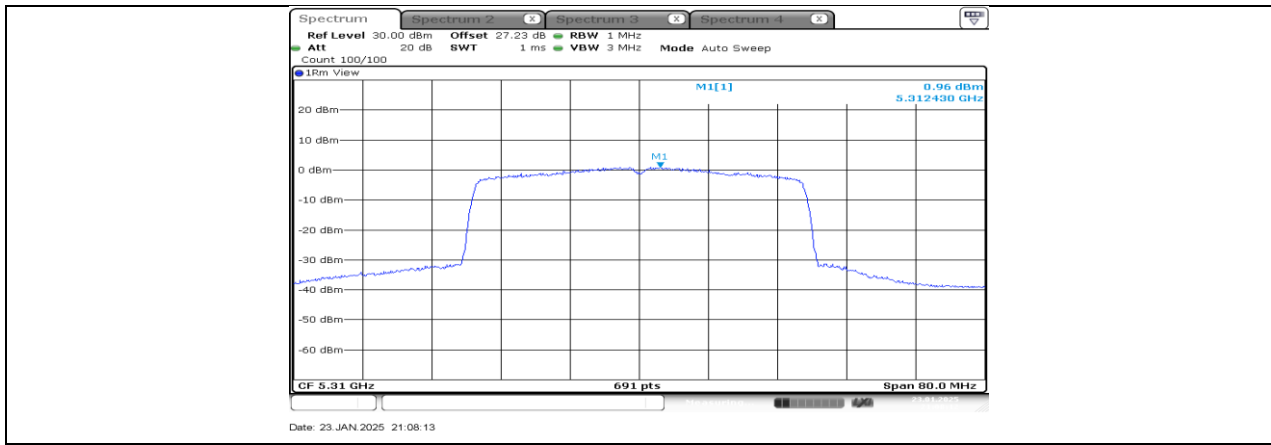
11AX40SISO SU_Ant3_5310
