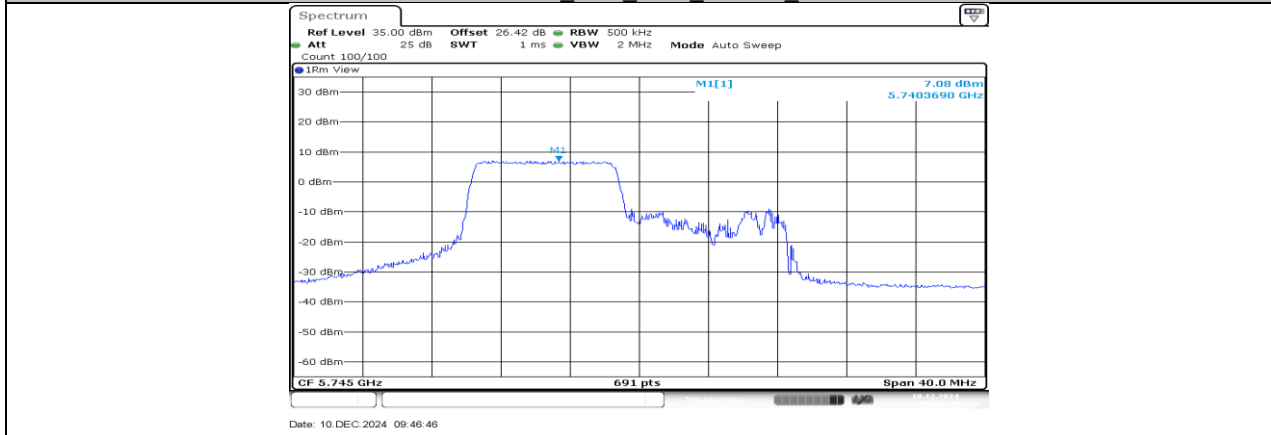
11AX20SISO Ant3_5745_106Tone_RU53
