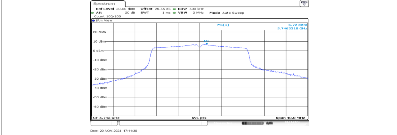
11N20SISO Ant3 5745
