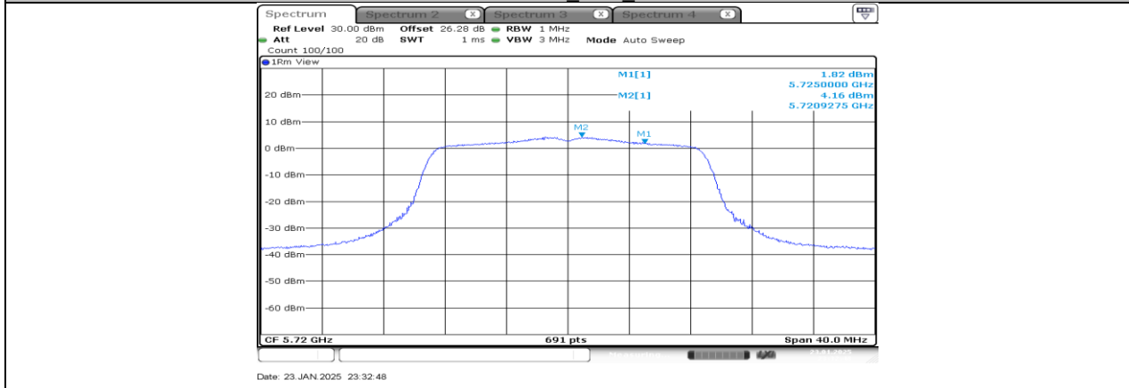
11N20SISO_Ant3_5720_UNII-2C
