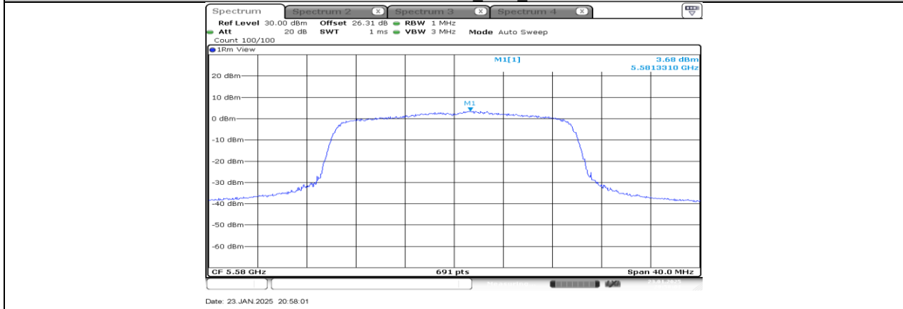
11AX20SISO SU_Ant3_5580
