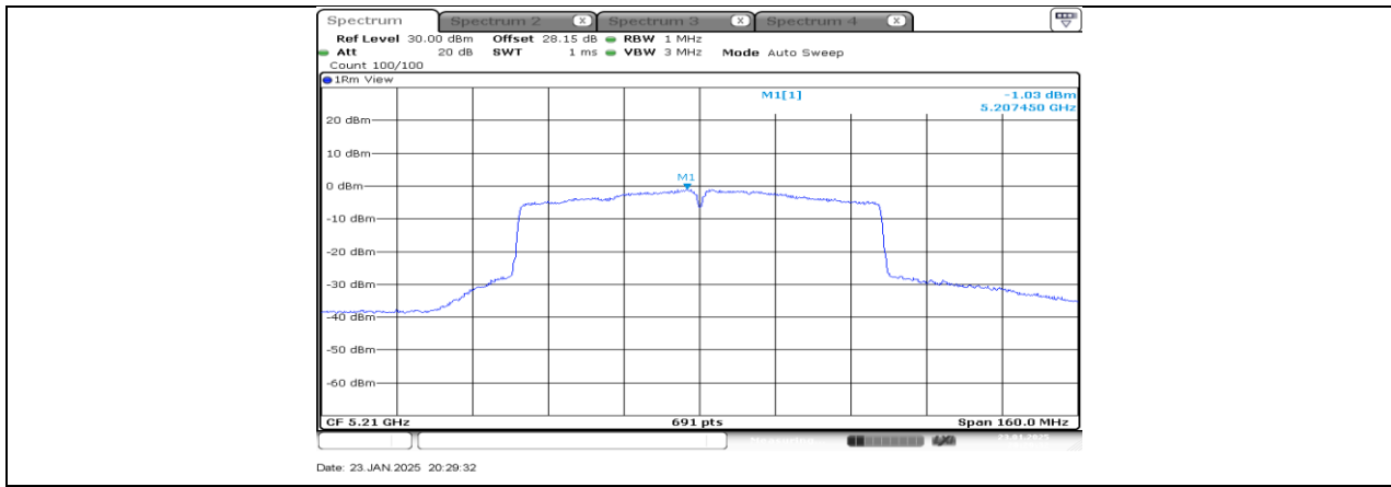
11AC80SISO_Ant3_5210
