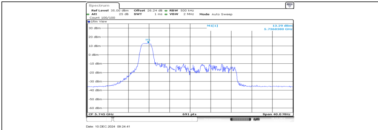
11AX20SISO Ant3_5745_26Tone_RU0
