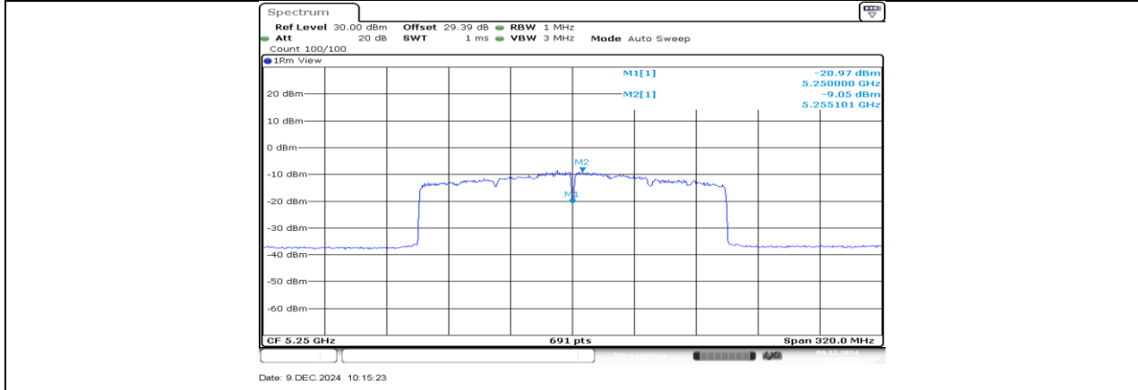
11AX160SISO SU_Ant3_5250_UNII-2A
