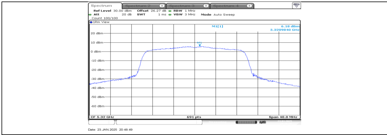
11AX20SISO SU_Ant3_5320
