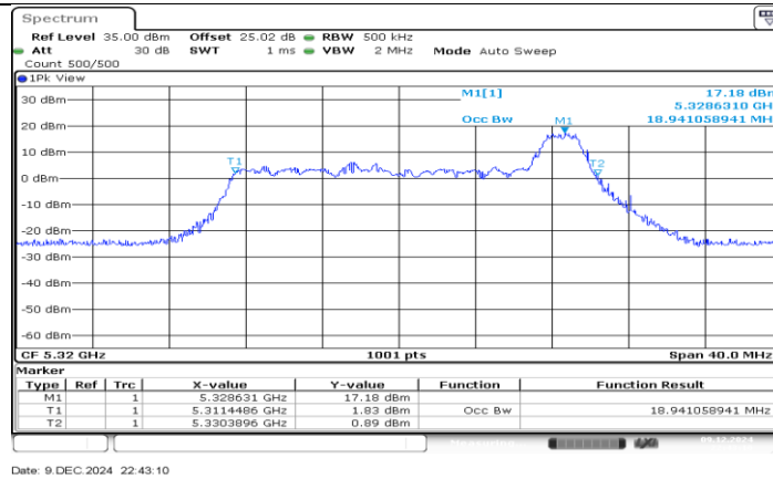
11AX20SISO Ant3_5320_26Tone_RU8
