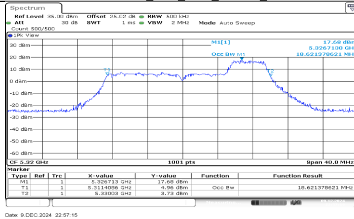
11AX20SISO Ant3_5320_52Tone_RU40
