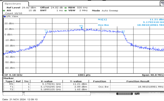
11AX20SISO_SU_Ant3_5180
