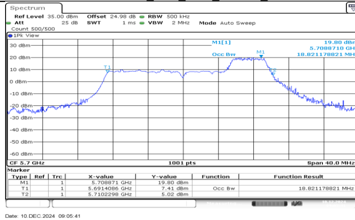
11AX20SISO Ant3_5700_52Tone_RU40
