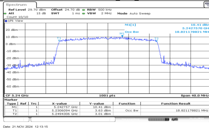
11AX20SISO SU_Ant3_5240
