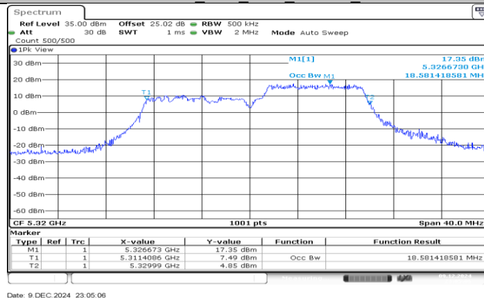
11AX20SISO Ant3_5320_106Tone_RU54
