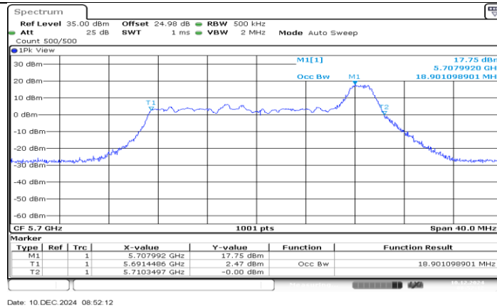
11AX20SISO Ant3_5700_26Tone_RU8
