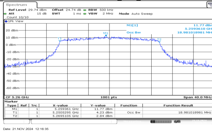
11AX20SISO SU_Ant3_5260
