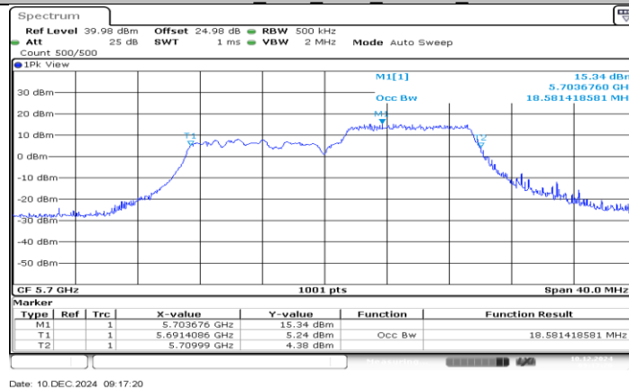
11AX20SISO Ant3_5700_106Tone_RU54
