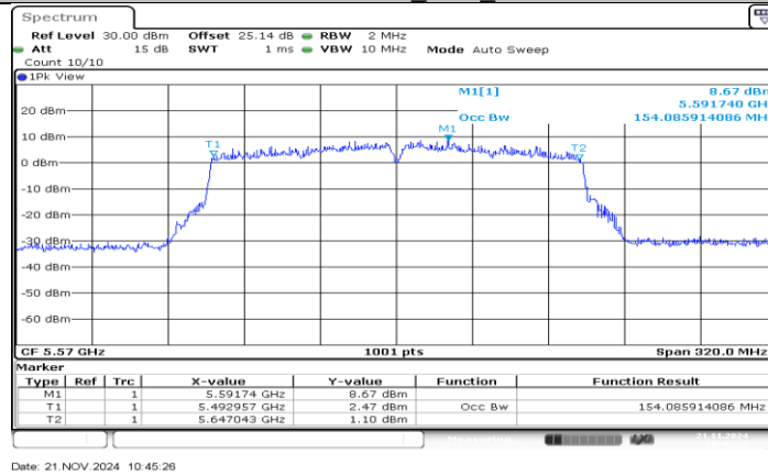
11AC160SISO_Ant3_5570
