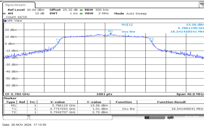
11N20SISO_Ant3_5785
