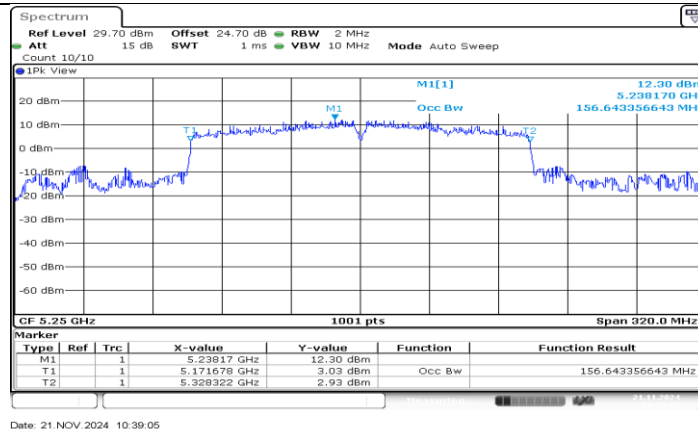
11AC160SISO_Ant3_5250
