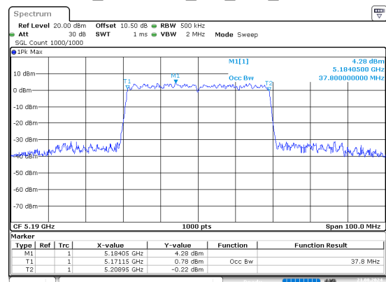
ac40_5190MHz_RU_Full_Chain 0
