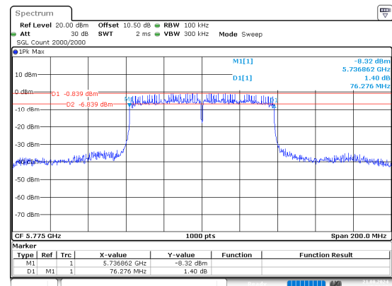
ac80_5775MHz_Chain 0
