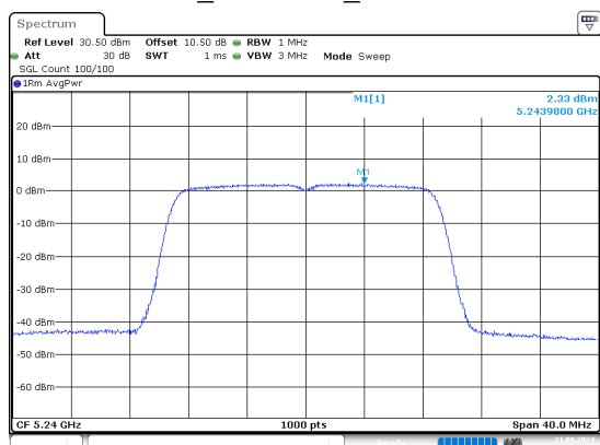
n20_5240MHz_Chain 0
