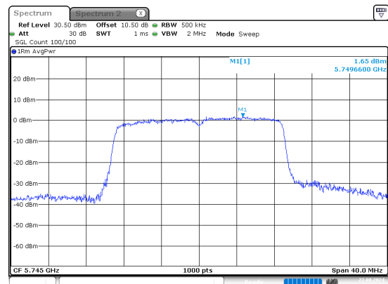
ac20_5745MHz_Chain 1
