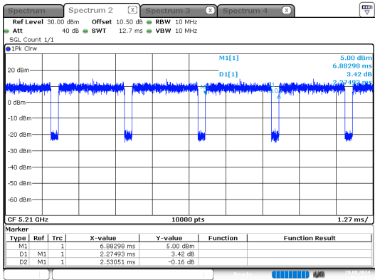
ax80_5210MHz_RU_Full_Chain 0
