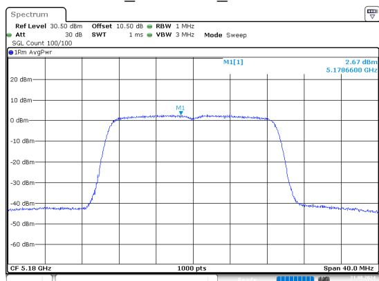
n20_5180MHz_Chain 0
