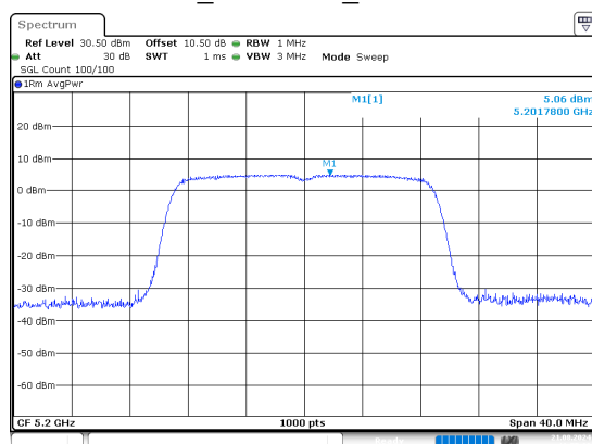
n20_5200MHz_Chain 1
