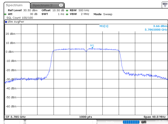
a_5785MHz_Chain 1
