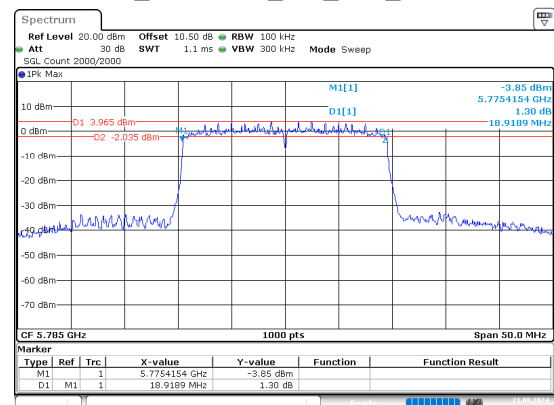
ax20_5785MHz_RU_Full_Chain 0
