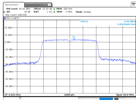
a_5825MHz_Chain 1
