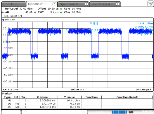
ax20_5200MHz_RU_Full_Chain 0
