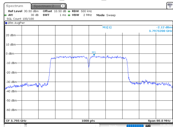
ac40_5795MHz_Chain 1
