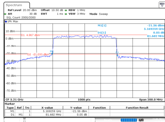
ax80_5210MHz_RU_Full_Chain 0
