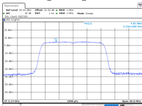
n20_5240MHz_Chain 1
