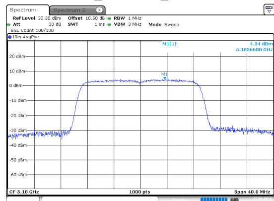
ac20_5180MHz_Chain 1
