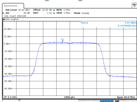
n20_5200MHz_Chain 0
