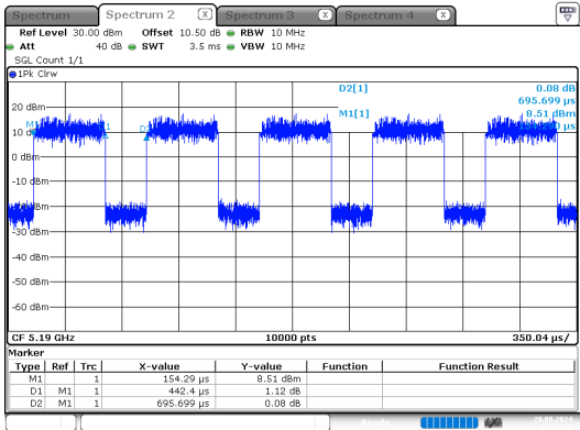
ax40_5190MHz_RU_Full_Chain 0
