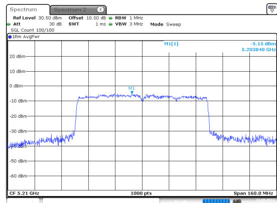
ax80_5210MHz_RU_Full_Chain 1
