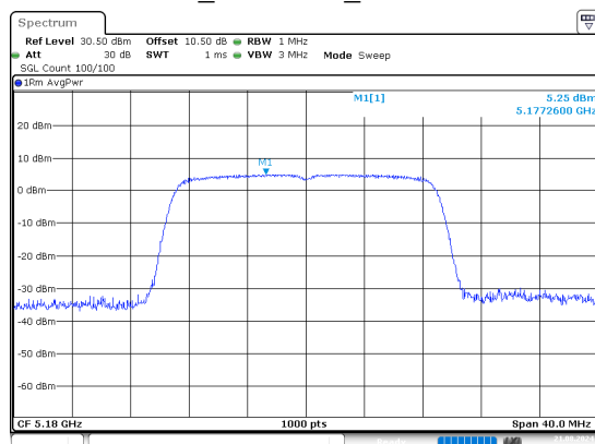
n20_5180MHz_Chain 1
