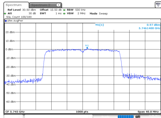
ax20_5745MHz_RU_Full_Chain 1
