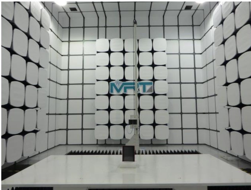
Description: Radiated Emission Test Setup for 18 ~ 25GHz
